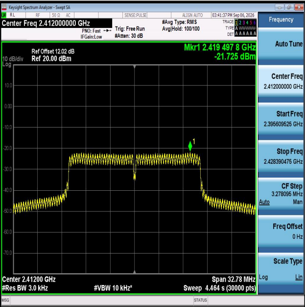
11N20MIMO-Ant2-2412-PASS
