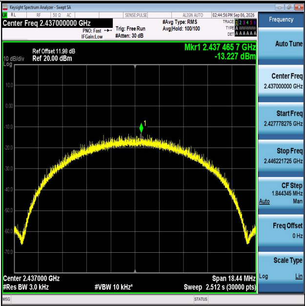
11B-Ant2-2437-PASS
