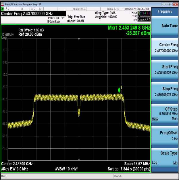
11N40MIMO-Ant2-2437-PASS
