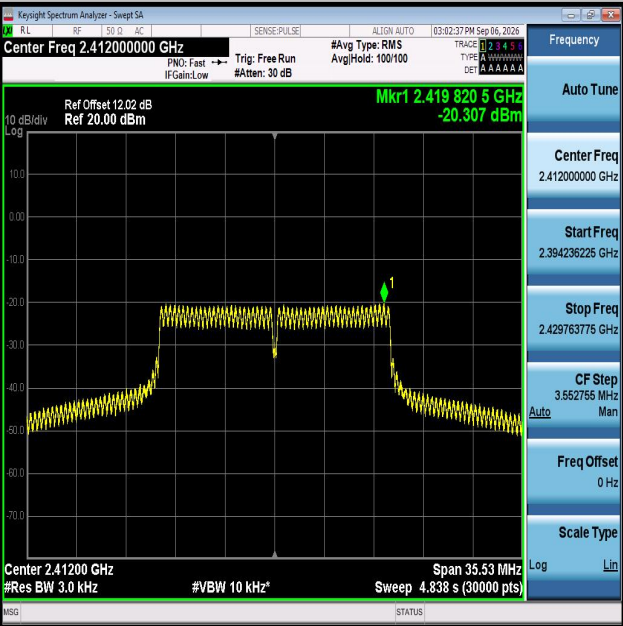
11G-Ant2-2412-PASS
