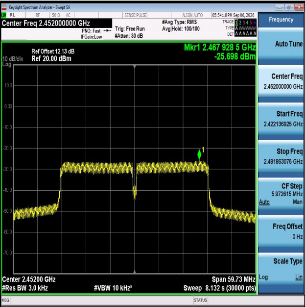
11N40MIMO-Ant2-2452-PASS
