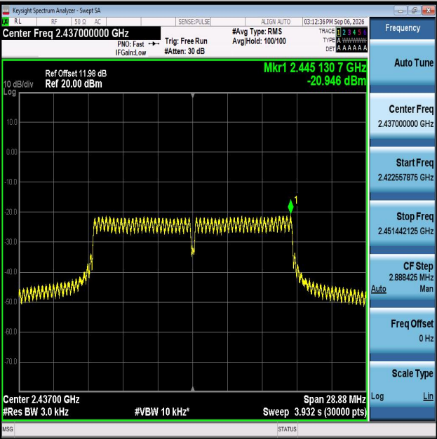
11G-Ant2-2437-PASS
