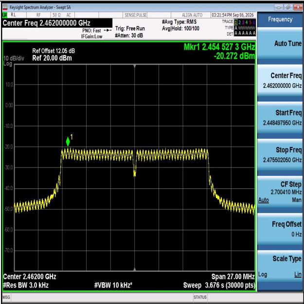
11G-Ant2-2462-PASS
