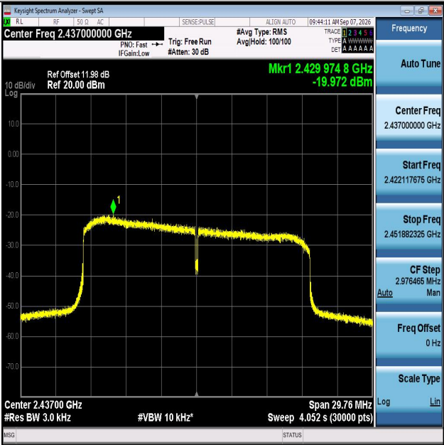
11AX20MIMO-Ant2-2437-PASS
