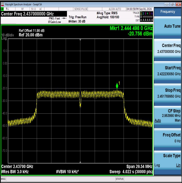
11N20MIMO-Ant2-2437-PASS
