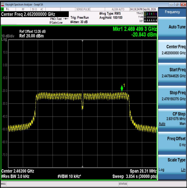
11N20MIMO-Ant2-2462-PASS
