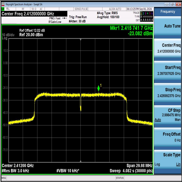
11AX20MIMO-Ant2-2412-PASS
