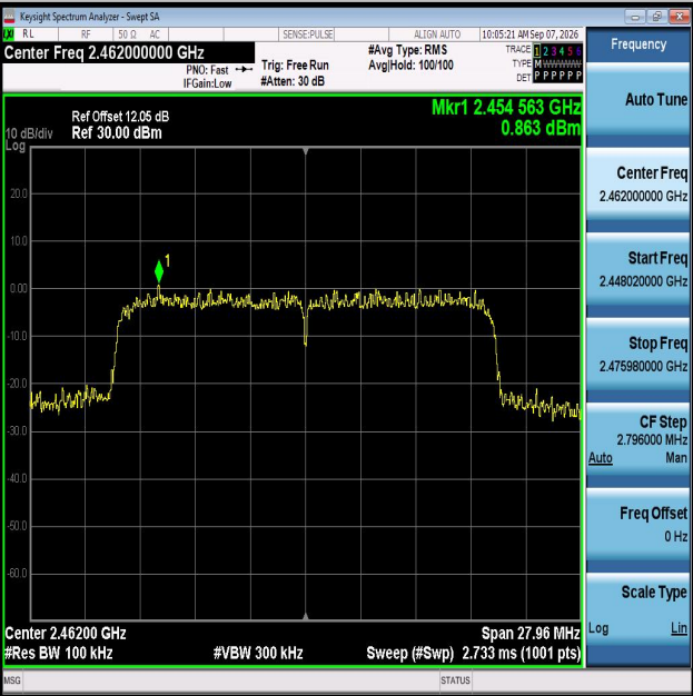
11AX20MIMO-Ant2-2462-PASS
