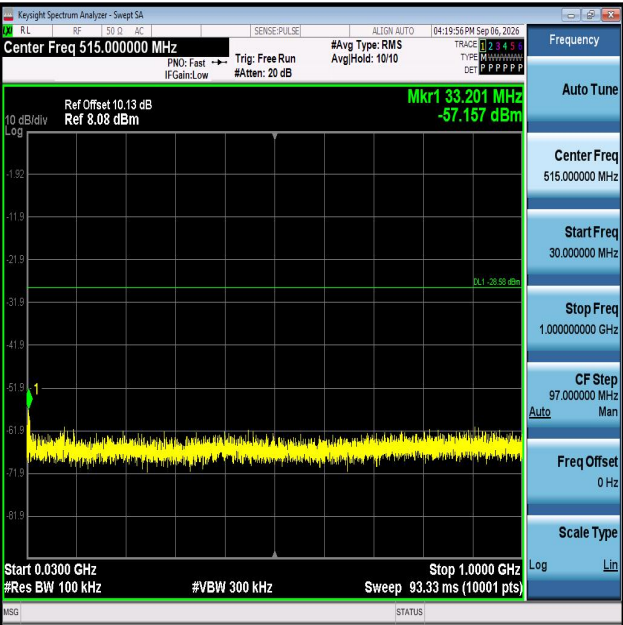
11N20MIMO-Ant2-2462-30~1000-PASS
