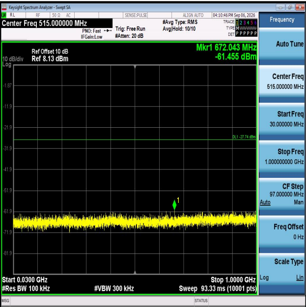
11N20MIMO-Ant1-2462-30~1000-PASS
