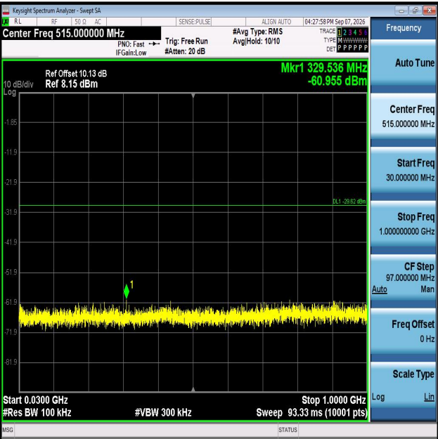
11AX40MIMO-Ant2-2437-30~1000-PASS
