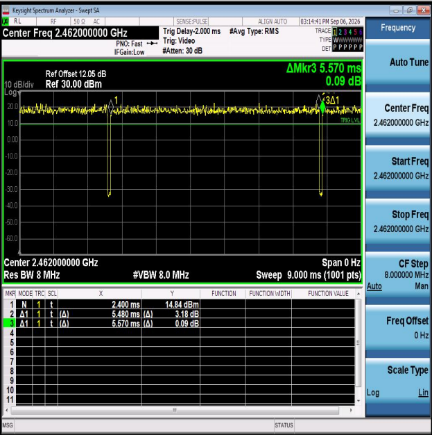
NTNV-11G-Ant2-2462
