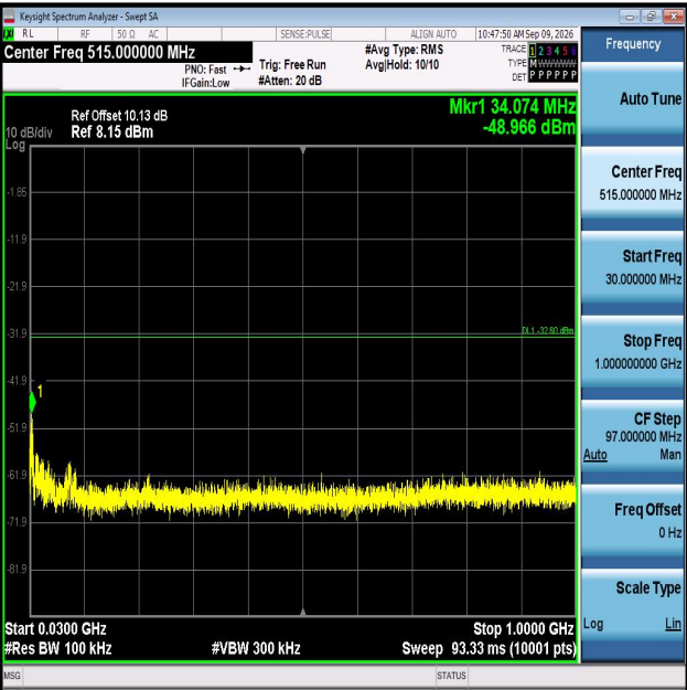
11AX40MIMO-Ant2-2422-30~1000-PASS
