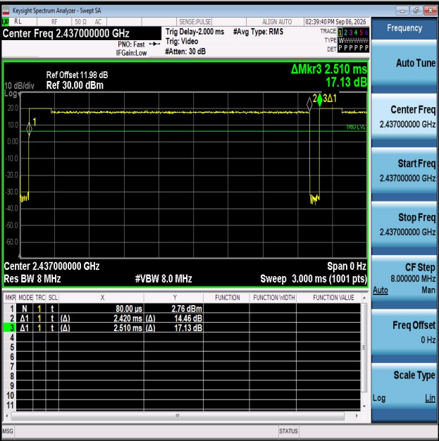
NTNV-11B-Ant2-2437
