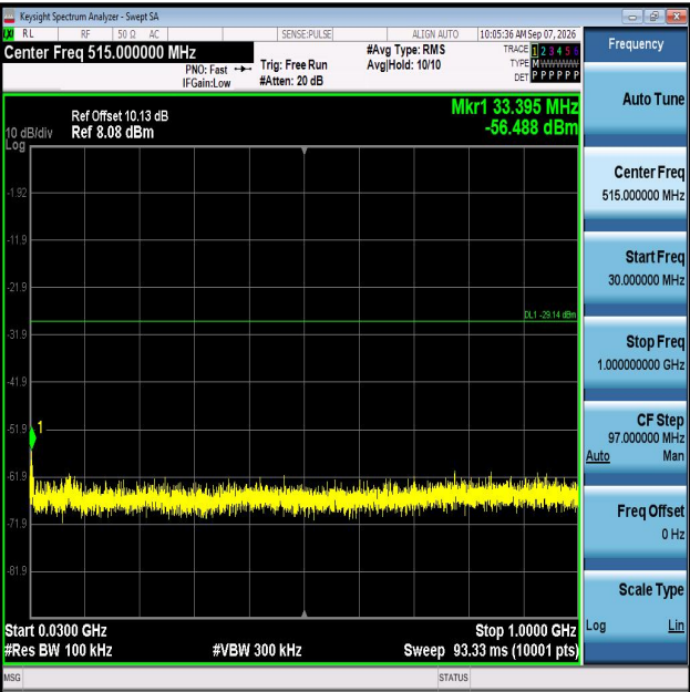
11AX20MIMO-Ant2-2462-30~1000-PASS
