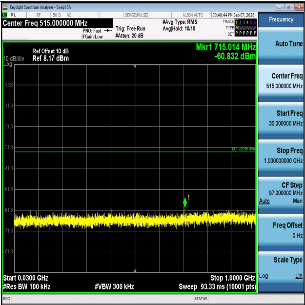
11AX40MIMO-Ant1-2422-30~1000-PASS
