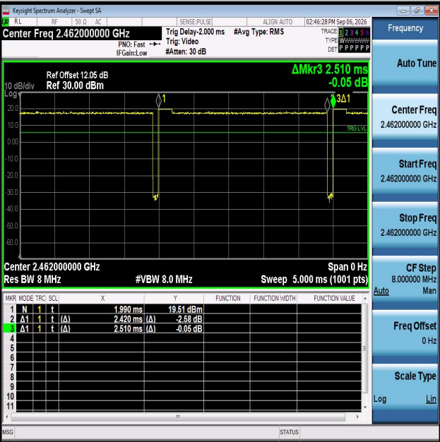
NTNV-11B-Ant2-2462
