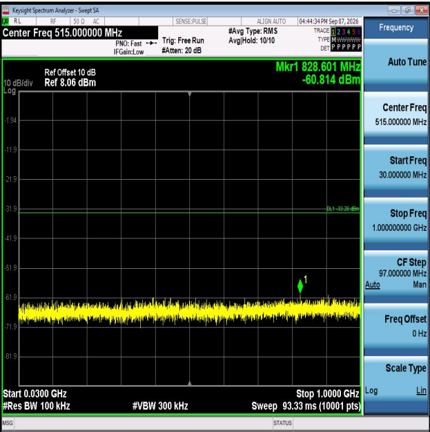
11AX40MIMO-Ant1-2452-30~1000-PASS
