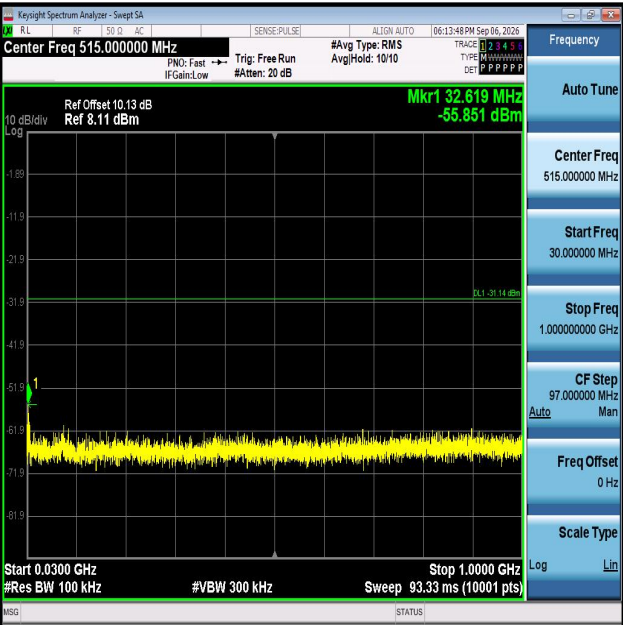
11AX20MIMO-Ant2-2412-30~1000-PASS
