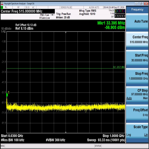
11AX20MIMO-Ant2-2437-30~1000-PASS
