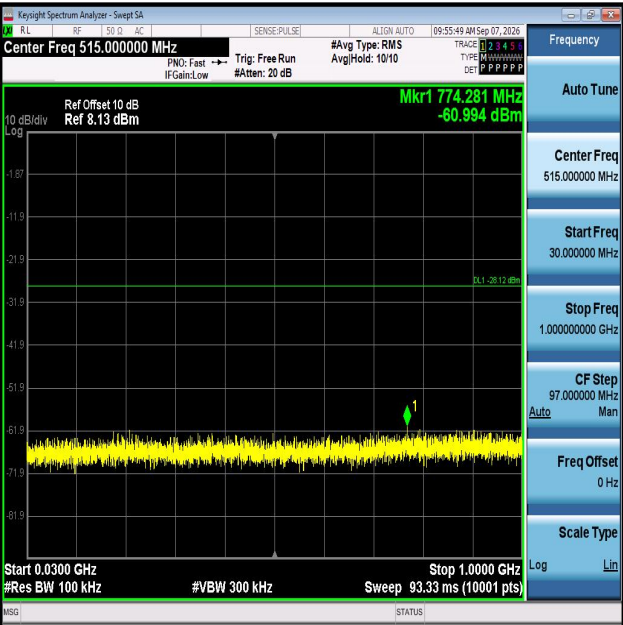
11AX20MIMO-Ant1-2462-30~1000-PASS
