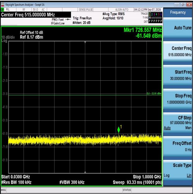
11AX40MIMO-Ant1-2437-30~1000-PASS
