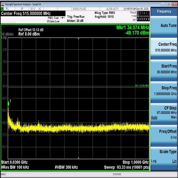
11AX40MIMO-Ant2-2452-30~1000-PASS
