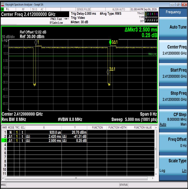
NTNV-11B-Ant2-2412
