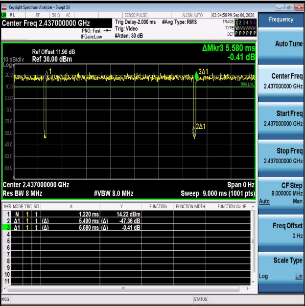
NTNV-11G-Ant2-2437
