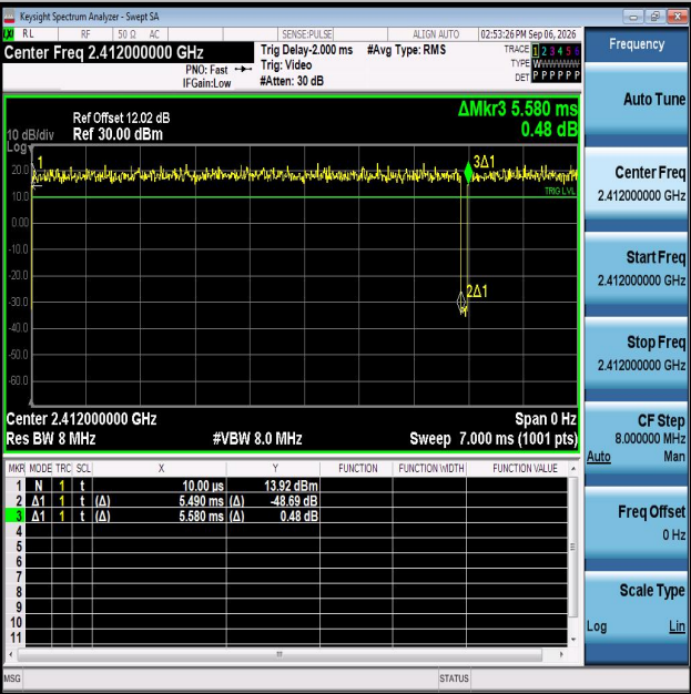
NTNV-11G-Ant2-2412
