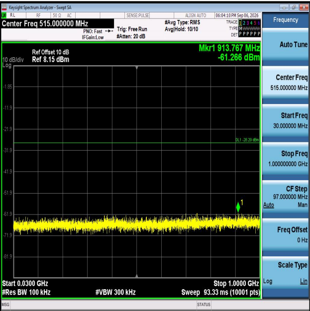
11AX20MIMO-Ant1-2412-30~1000-PASS
