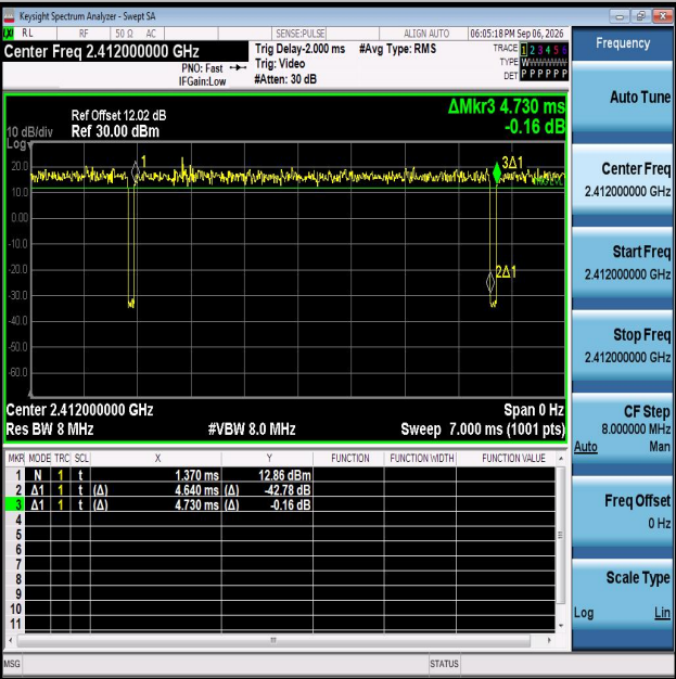
NTNV-11AX20MIMO-Ant2-2412
