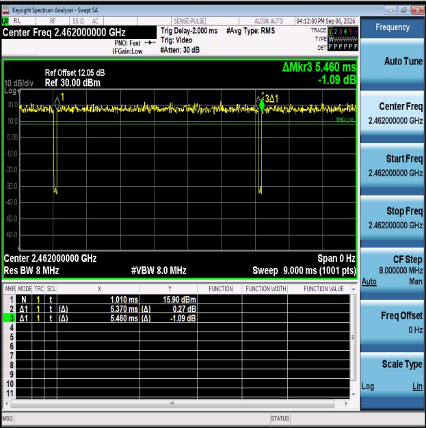
NTNV-11N20MIMO-Ant2-2462
