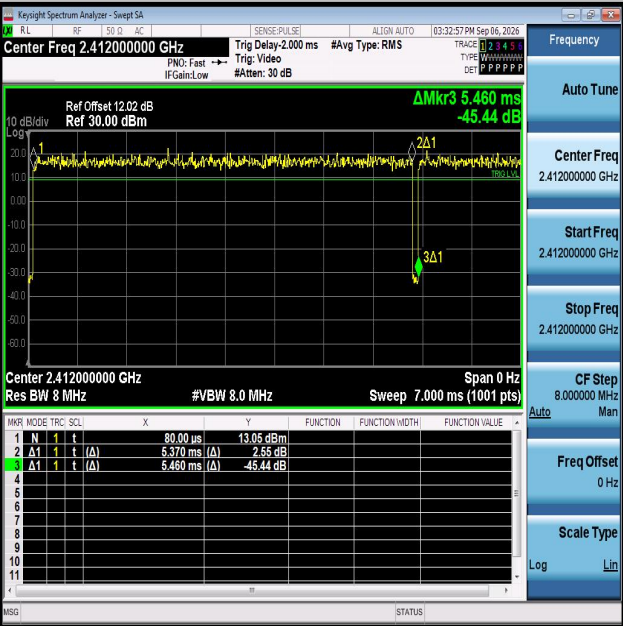
NTNV-11N20MIMO-Ant2-2412
