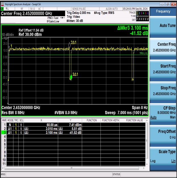
NTNV-11N40MIMO-Ant1-2452
