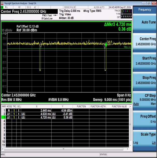
NTNV-11AX40MIMO-Ant2-2452
