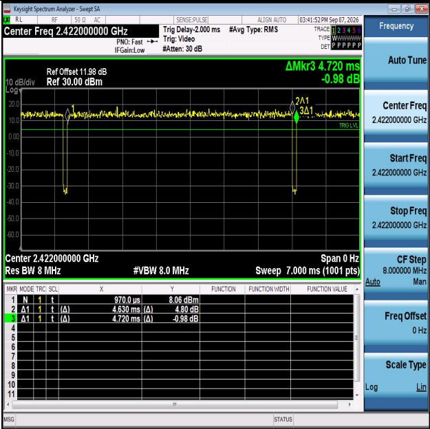
NTNV-11AX40MIMO-Ant2-2422
