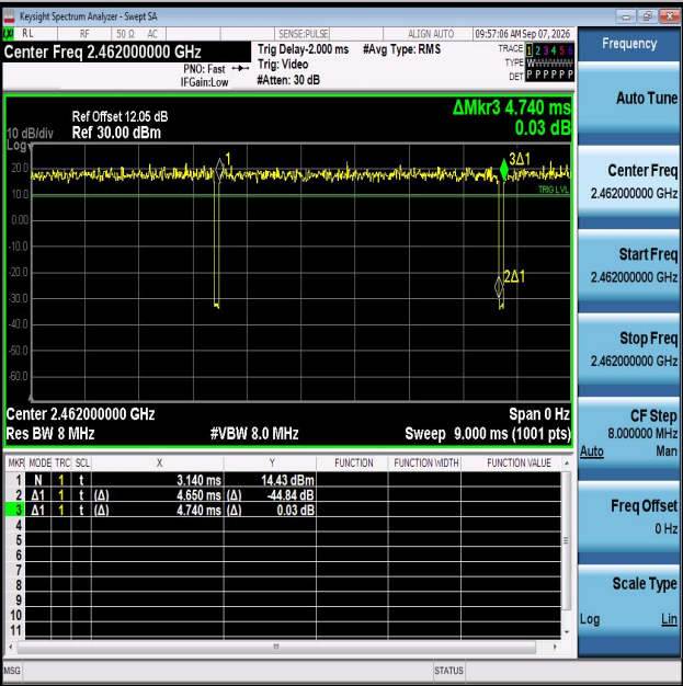
NTNV-11AX20MIMO-Ant2-2462
