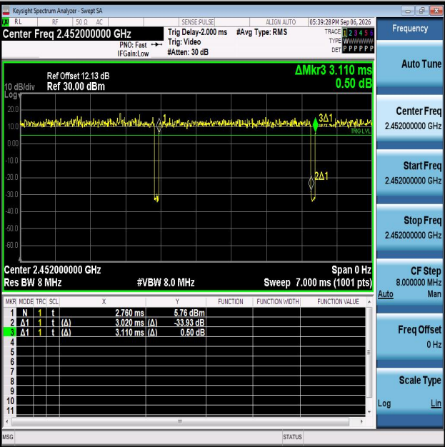
NTNV-11N40MIMO-Ant2-2452
