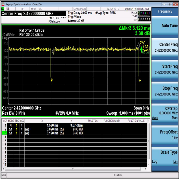
NTNV-11N40MIMO-Ant2-2422
