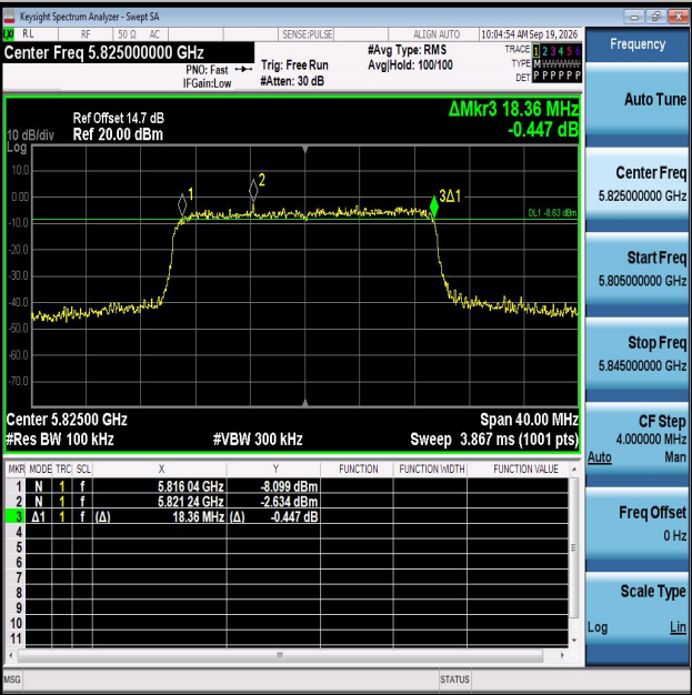
11AX20MIMO-Ant2-5825-PASS
