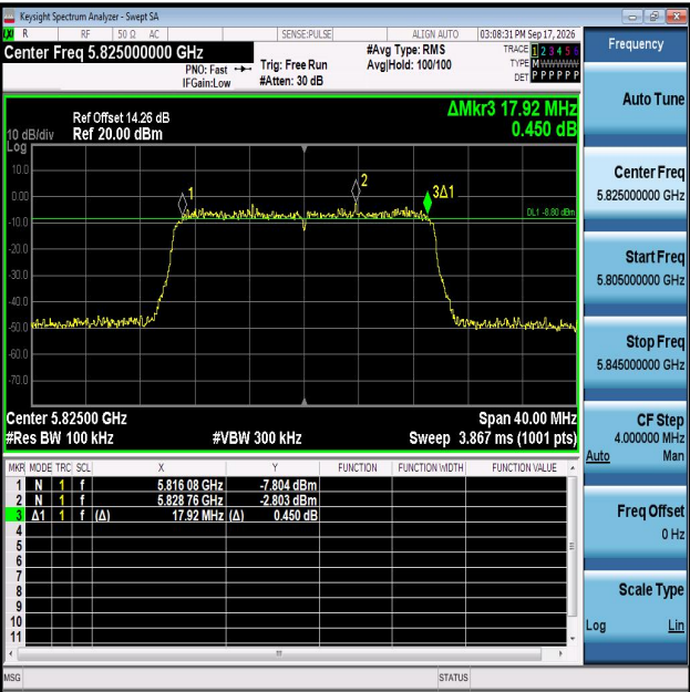
11AX20MIMO-Ant1-5825-PASS
