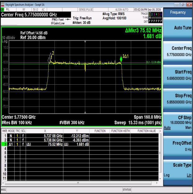
11AC80MIMO-Ant2-5775-PASS
