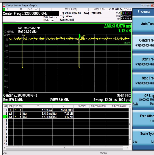
NTNV-11A-Ant2-5320
