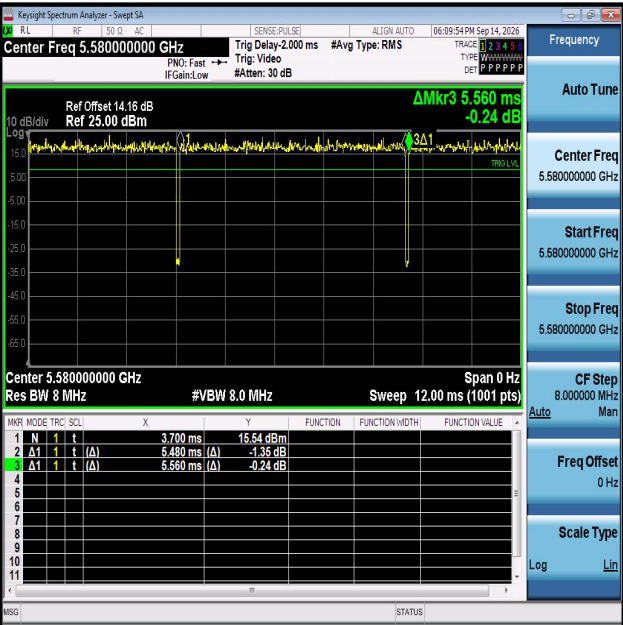
NTNV-11A-Ant1-5580
