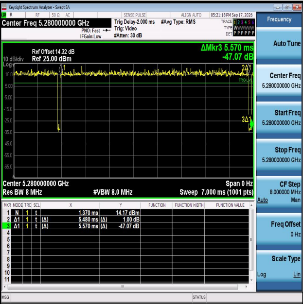
NTNV-11A-Ant2-5280
