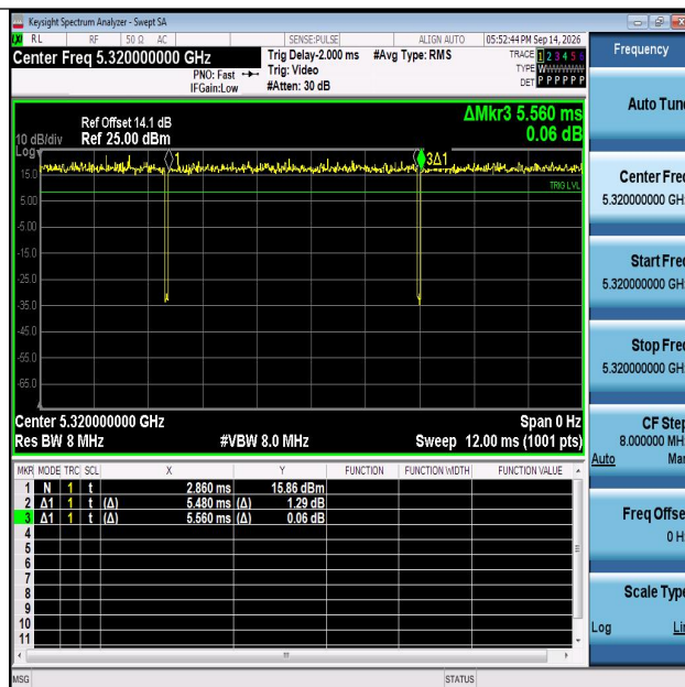
NTNV-11A-Ant1-5320
