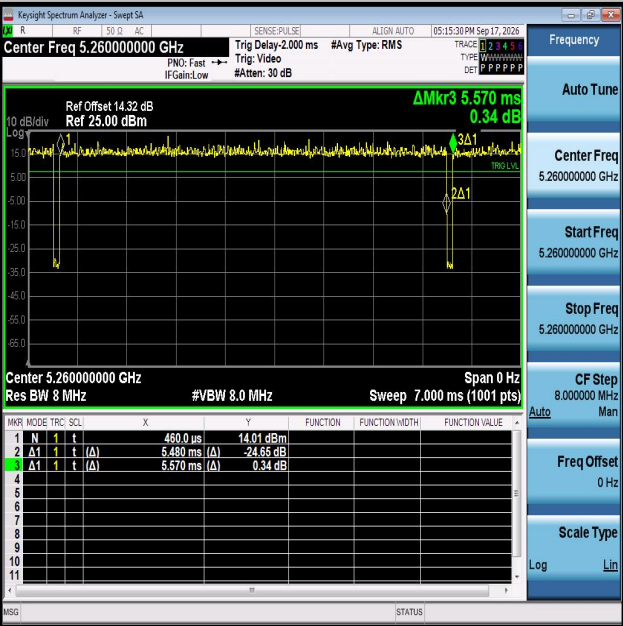
NTNV-11A-Ant2-5260
