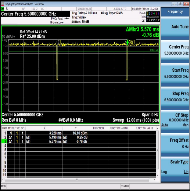
NTNV-11A-Ant2-5500
