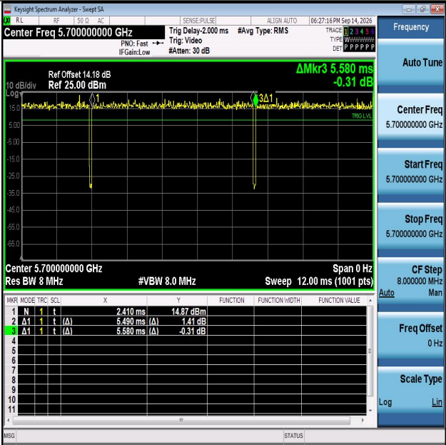
NTNV-11A-Ant1-5700
