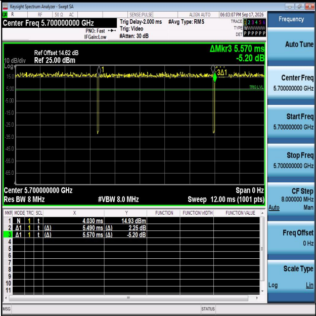
NTNV-11A-Ant2-5700
