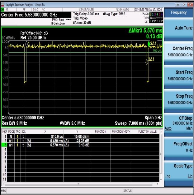
NTNV-11A-Ant2-5580
