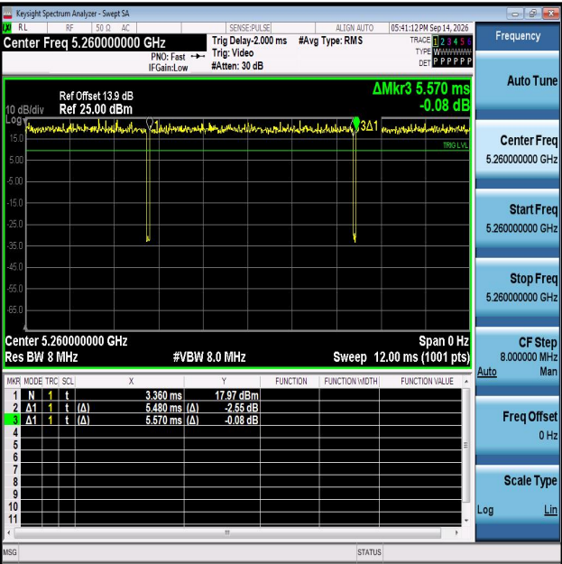
NTNV-11A-Ant1-5260
