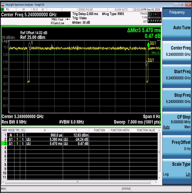
NTNV-11AC20MIMO-Ant2-5240
