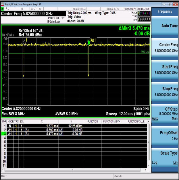
NTNV-11AC20MIMO-Ant2-5825
