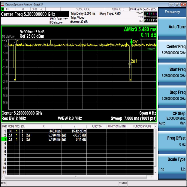
NTNV-11AC20MIMO-Ant1-5280
