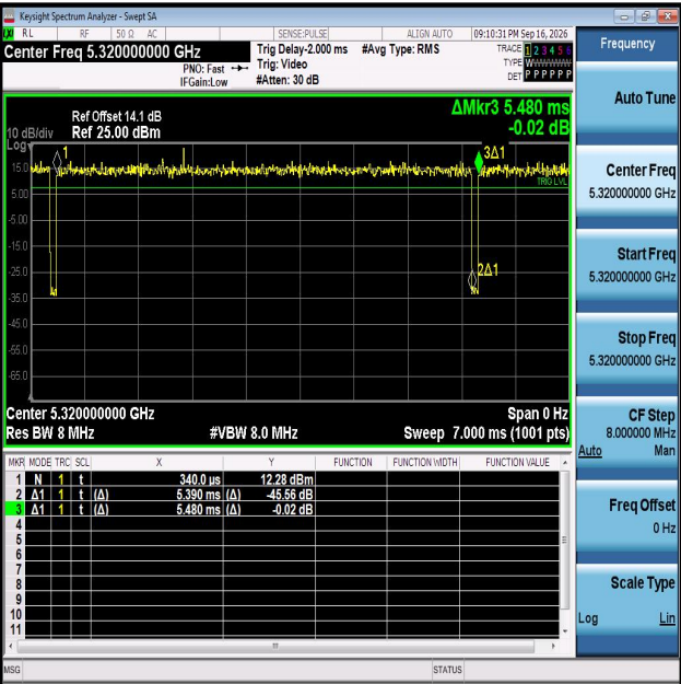
NTNV-11AC20MIMO-Ant1-5320
