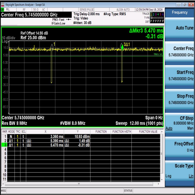
NTNV-11AC20MIMO-Ant2-5745
