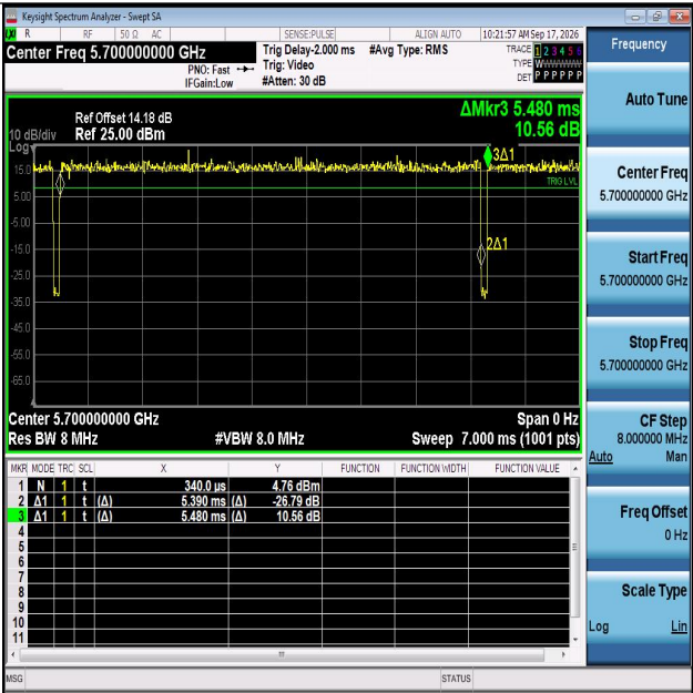
NTNV-11AC20MIMO-Ant1-5700
