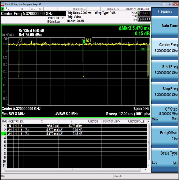
NTNV-11AC20MIMO-Ant2-5320
