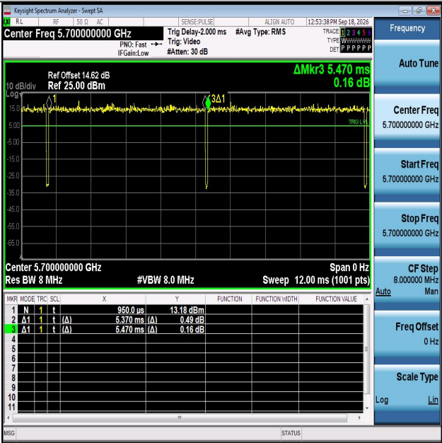
NTNV-11AC20MIMO-Ant2-5700
