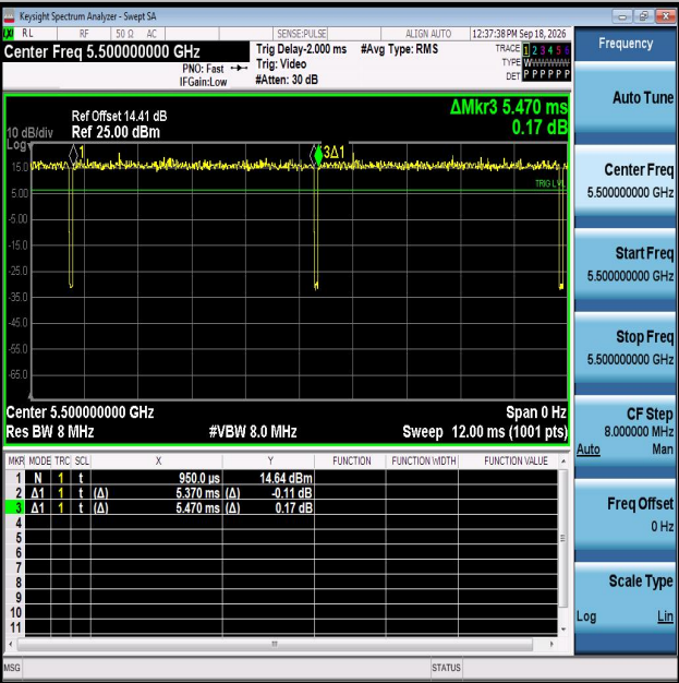
NTNV-11AC20MIMO-Ant2-5500
