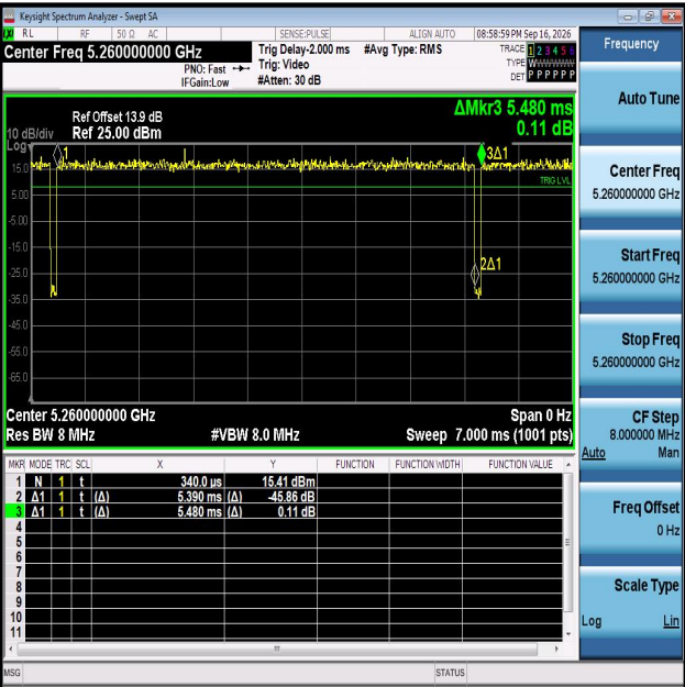
NTNV-11AC20MIMO-Ant1-5260
