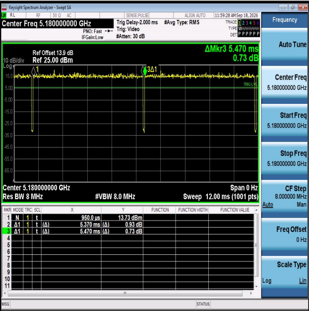
NTNV-11AC20MIMO-Ant2-5180
