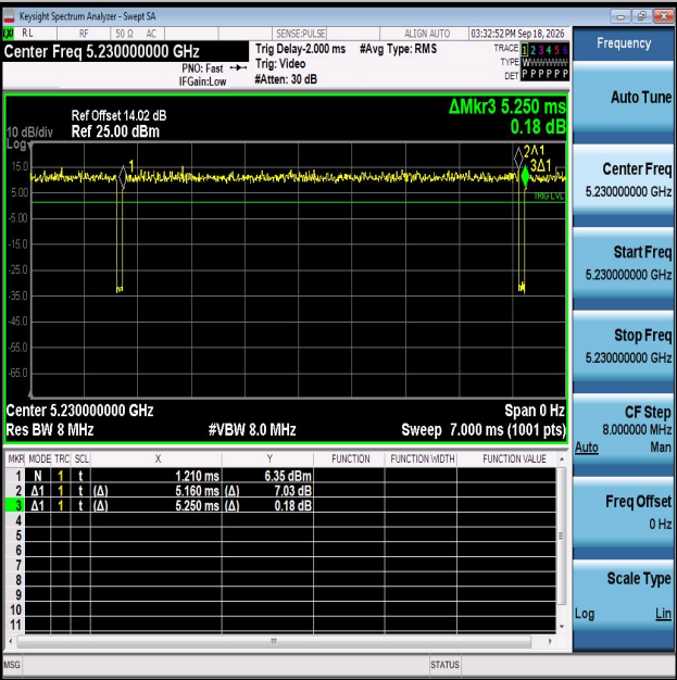
NTNV-11AC40MIMO-Ant2-5230
