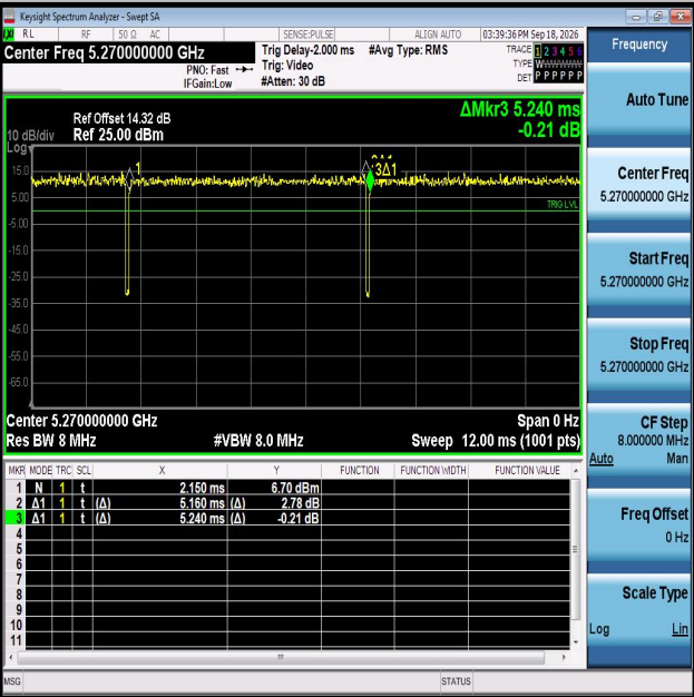
NTNV-11AC40MIMO-Ant2-5270
