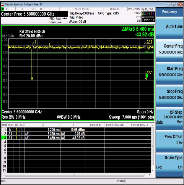
NTNV-11AC20MIMO-Ant1-5500
