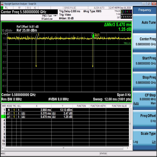
NTNV-11AC20MIMO-Ant2-5580
