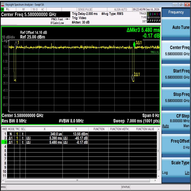
NTNV-11AC20MIMO-Ant1-5580
