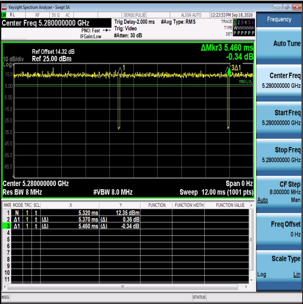
NTNV-11AC20MIMO-Ant2-5280
