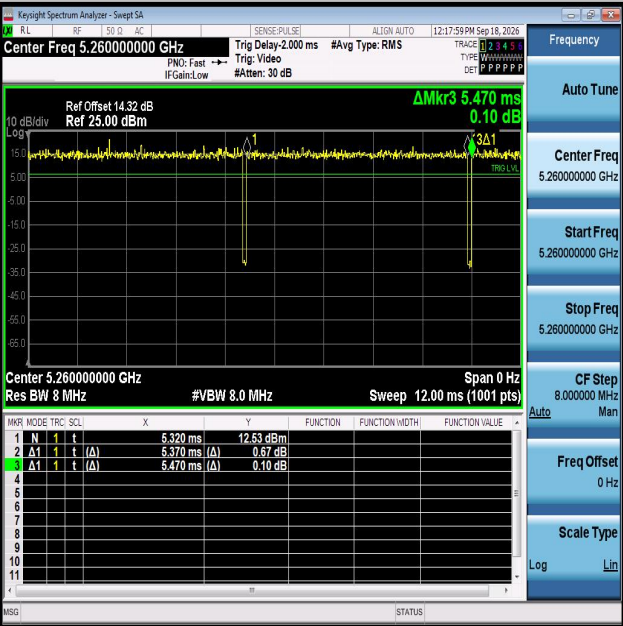
NTNV-11AC20MIMO-Ant2-5260
