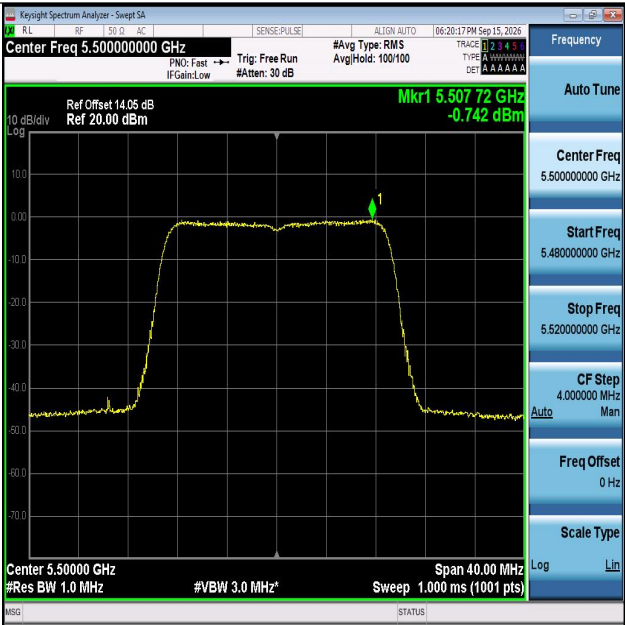
11N20MIMO-Ant1-5500-PASS
