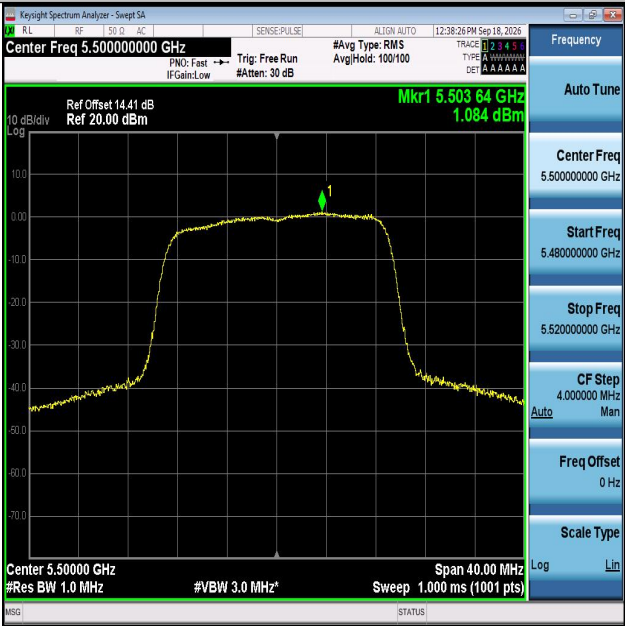
11AC20MIMO-Ant2-5500-PASS
