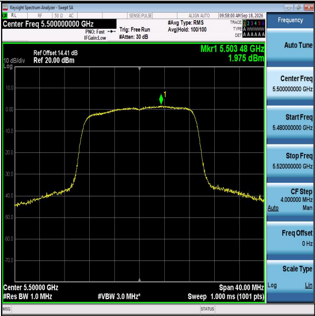
11N20MIMO-Ant2-5500-PASS
