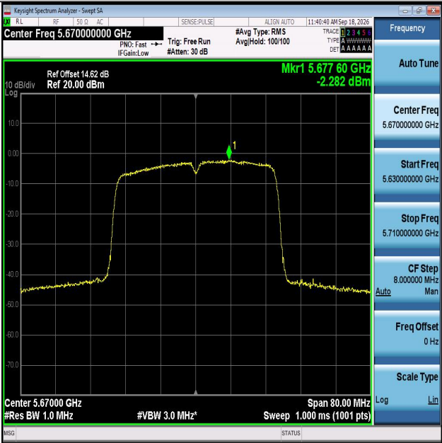
11N40MIMO-Ant2-5670-PASS
