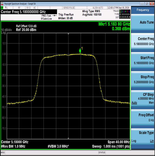
11AC20MIMO-Ant2-5180-PASS
