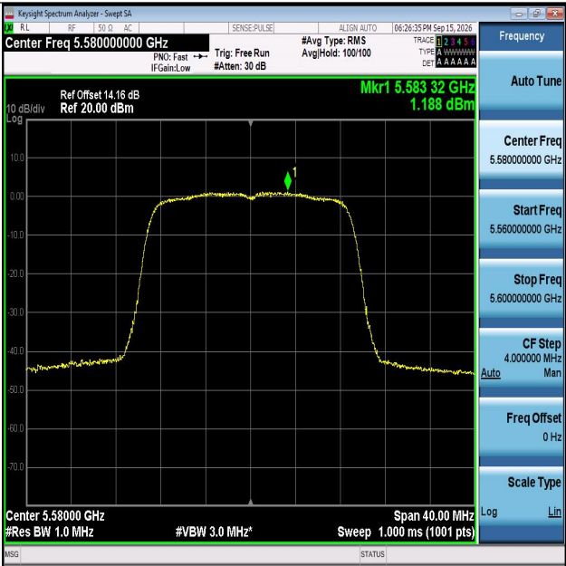
11N20MIMO-Ant1-5580-PASS
