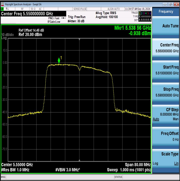
11N40MIMO-Ant2-5550-PASS
