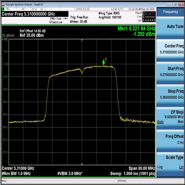
11N40MIMO-Ant2-5310-PASS
