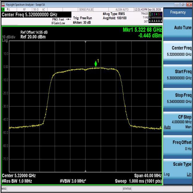
11AC20MIMO-Ant2-5320-PASS
