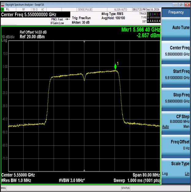
11N40MIMO-Ant1-5550-PASS
