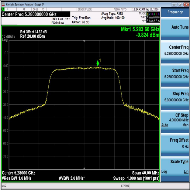
11AC20MIMO-Ant2-5280-PASS
