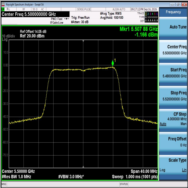
11AC20MIMO-Ant1-5500-PASS
