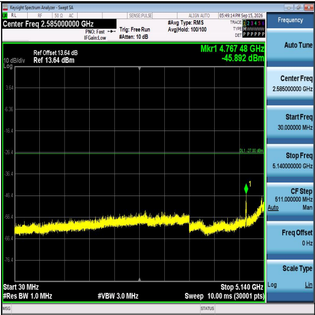
11N20MIMO-Ant1-5240-30~5140-PASS
