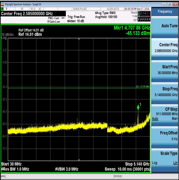
11N20MIMO-Ant2-5180-30~5140-PASS
