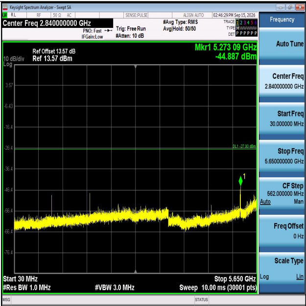
11A-Ant1-5745-30~5650-PASS
