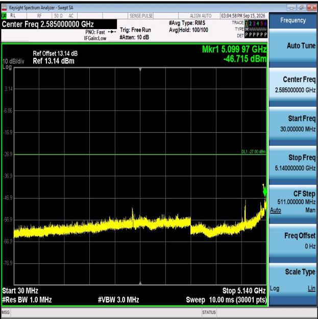
11N20MIMO-Ant1-5180-30~5140-PASS
