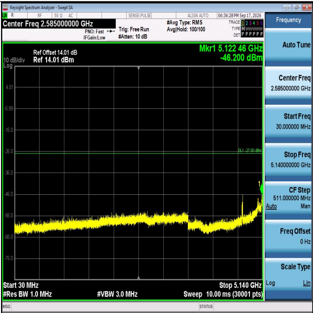
11N20MIMO-Ant2-5200-30~5140-PASS
