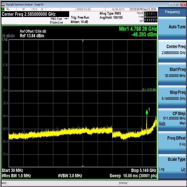
11N20MIMO-Ant1-5260-30~5140-PASS
