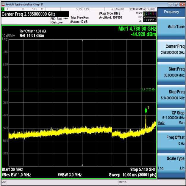
11N20MIMO-Ant2-5260-30~5140-PASS
