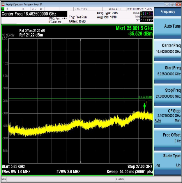
11A-Ant2-5745-5925~40000-PASS
