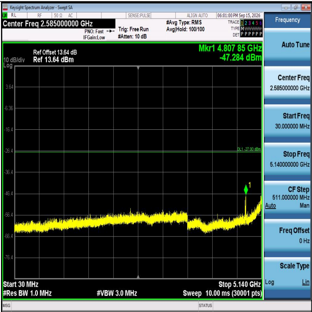
11N20MIMO-Ant1-5280-30~5140-PASS
