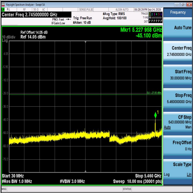
11A-Ant1-5700-30~5460-PASS
