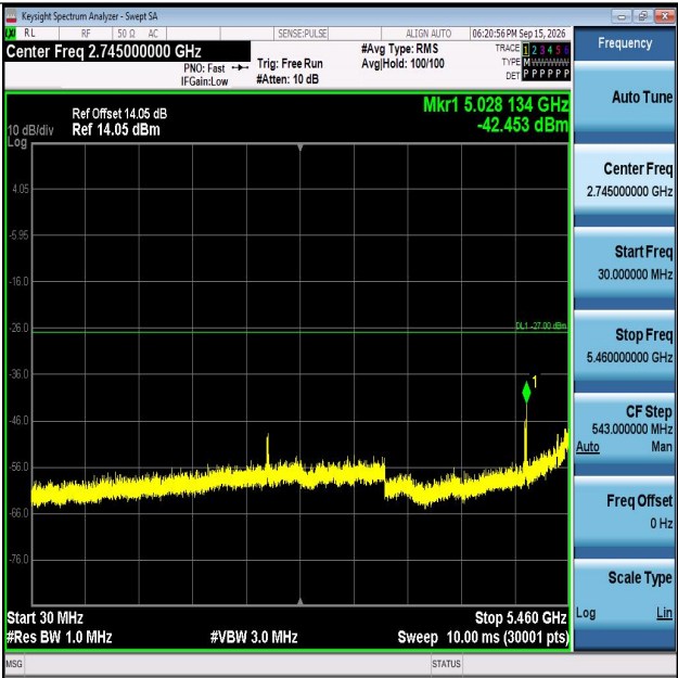
11N20MIMO-Ant1-5500-30~5460-PASS
