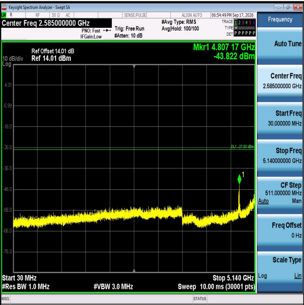
11N20MIMO-Ant2-5280-30~5140-PASS
