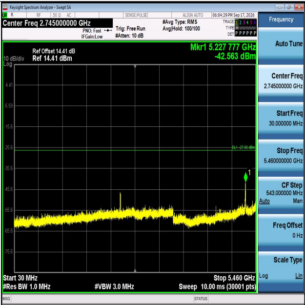
11A-Ant2-5700-30~5460-PASS
