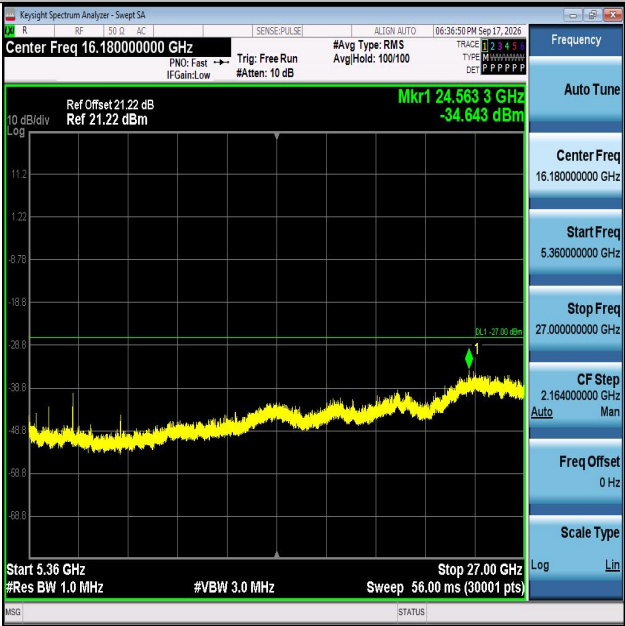
11N20MIMO-Ant2-5200-5360~40000-PASS
