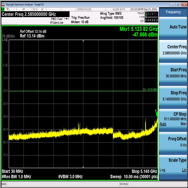
11N20MIMO-Ant1-5200-30~5140-PASS
