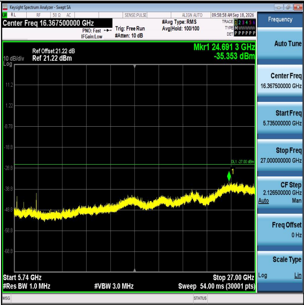
11N20MIMO-Ant2-5500-5735~40000-PASS
