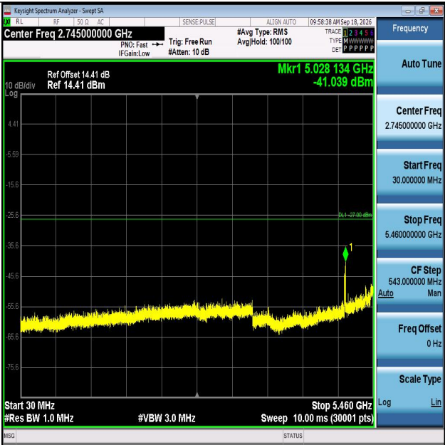
11N20MIMO-Ant2-5500-30~5460-PASS
