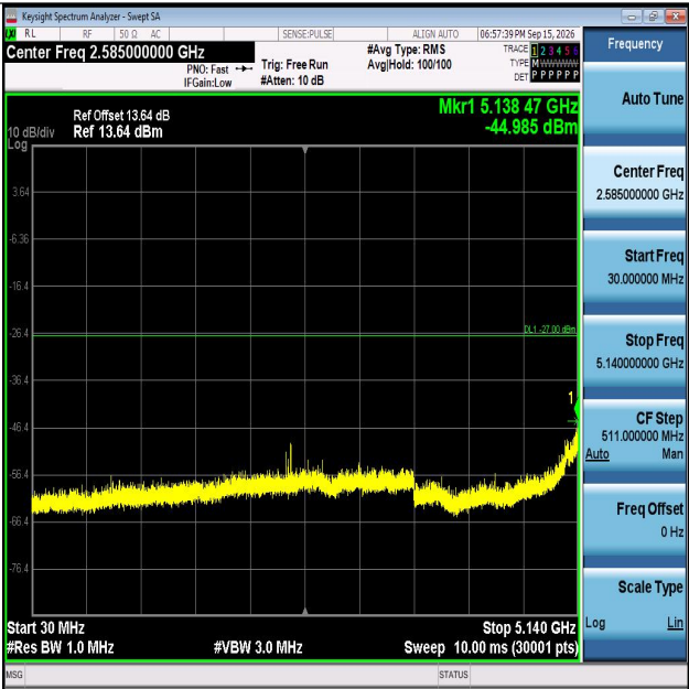
11N40MIMO-Ant1-5190-30~5140-PASS
