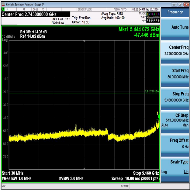
11N40MIMO-Ant1-5510-30~5460-PASS
