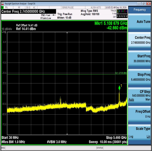
11N20MIMO-Ant2-5580-30~5460-PASS
