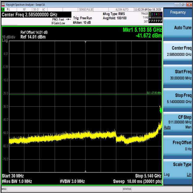
11N40MIMO-Ant2-5190-30~5140-PASS
