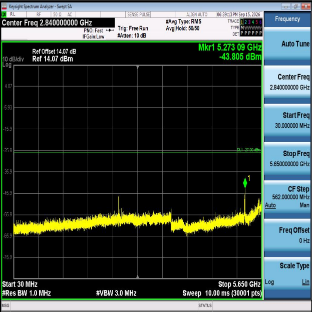
11N20MIMO-Ant1-5745-30~5650-PASS
