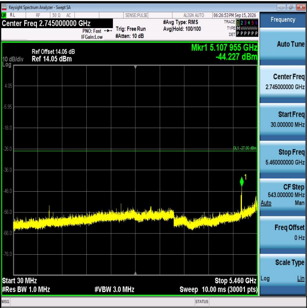
11N20MIMO-Ant1-5580-30~5460-PASS
