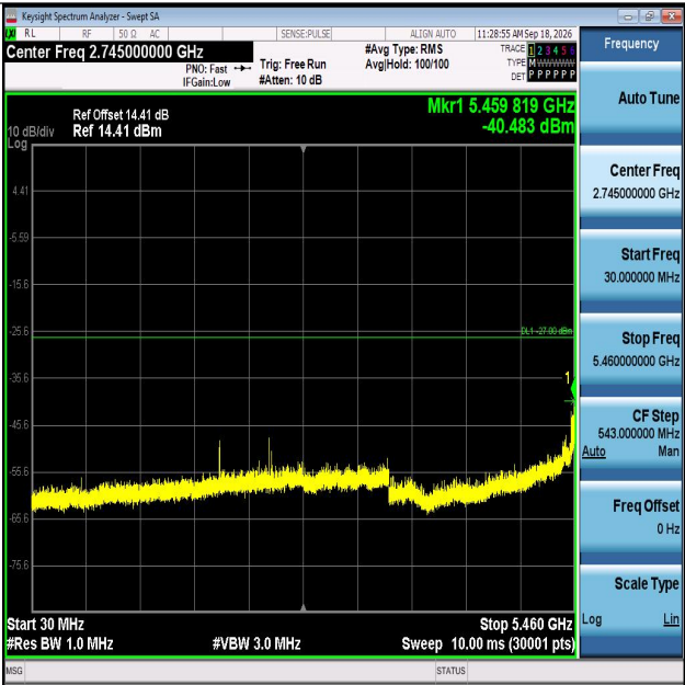
11N40MIMO-Ant2-5510-30~5460-PASS
