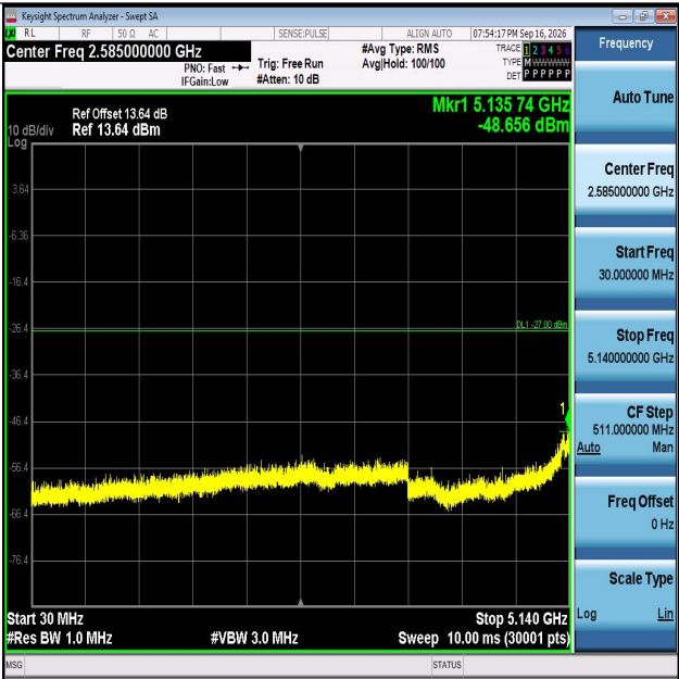
11N40MIMO-Ant1-5230-30~5140-PASS
