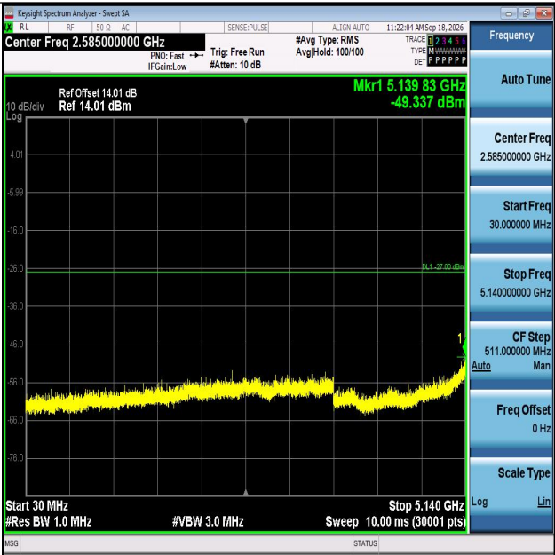
11N40MIMO-Ant2-5310-30~5140-PASS
