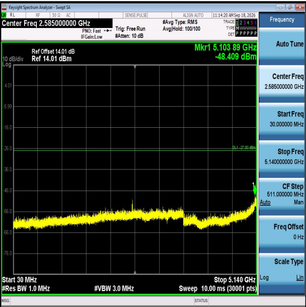
11N40MIMO-Ant2-5270-30~5140-PASS
