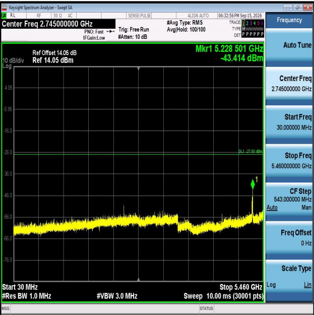
11N20MIMO-Ant1-5700-30~5460-PASS
