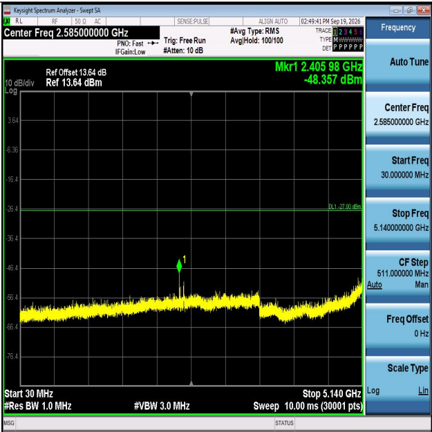
11N40MIMO-Ant1-5310-30~5140-PASS
