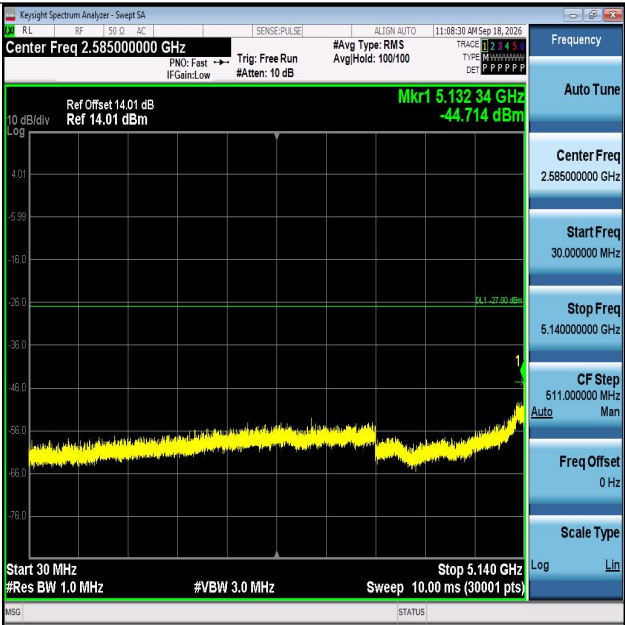
11N40MIMO-Ant2-5230-30~5140-PASS
