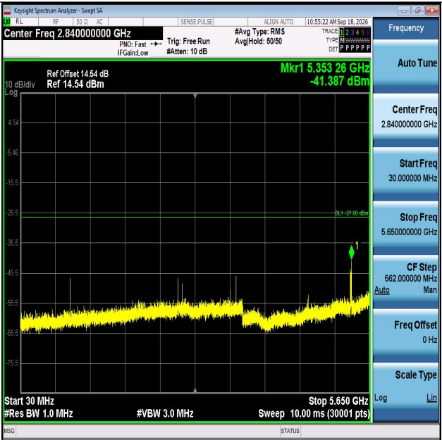
11N20MIMO-Ant2-5825-30~5650-PASS
