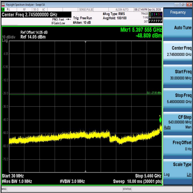
11N40MIMO-Ant1-5550-30~5460-PASS
