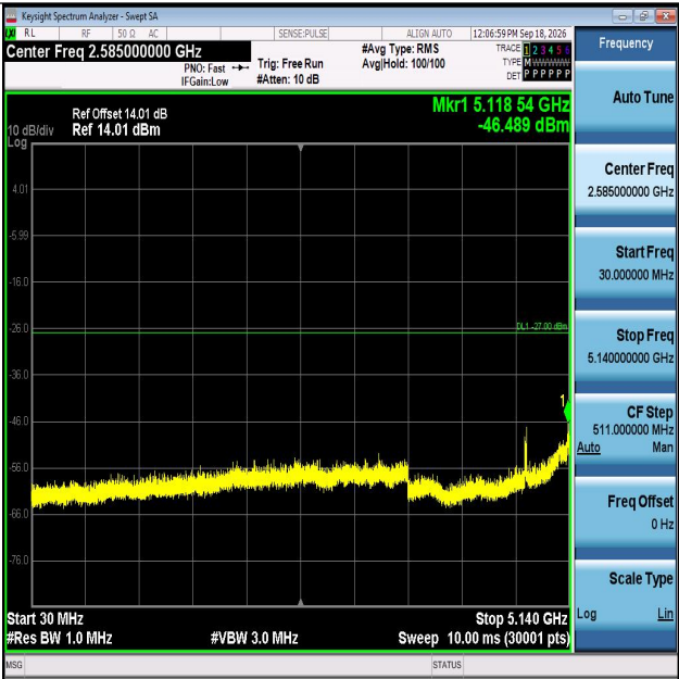
11AC20MIMO-Ant2-5200-30~5140-PASS
