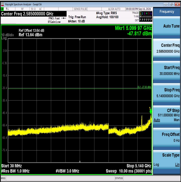
11AC20MIMO-Ant1-5260-30~5140-PASS
