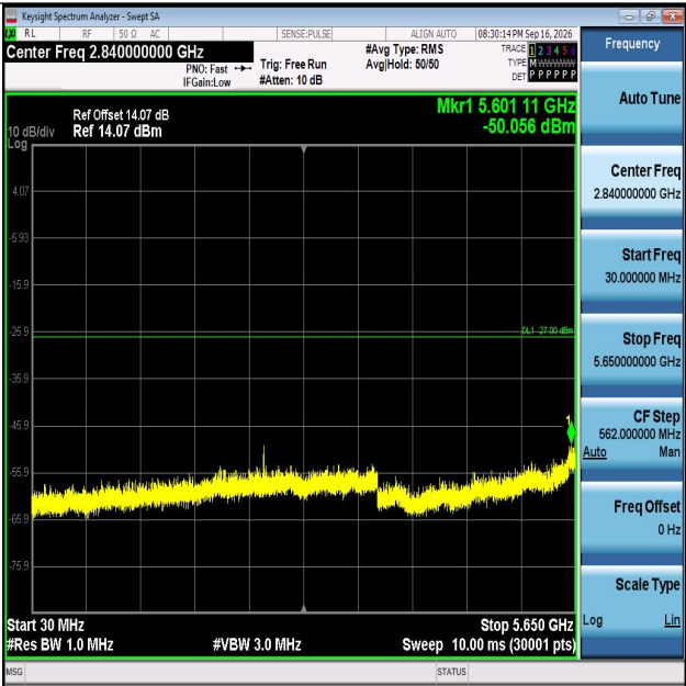
11N40MIMO-Ant1-5755-30~5650-PASS
