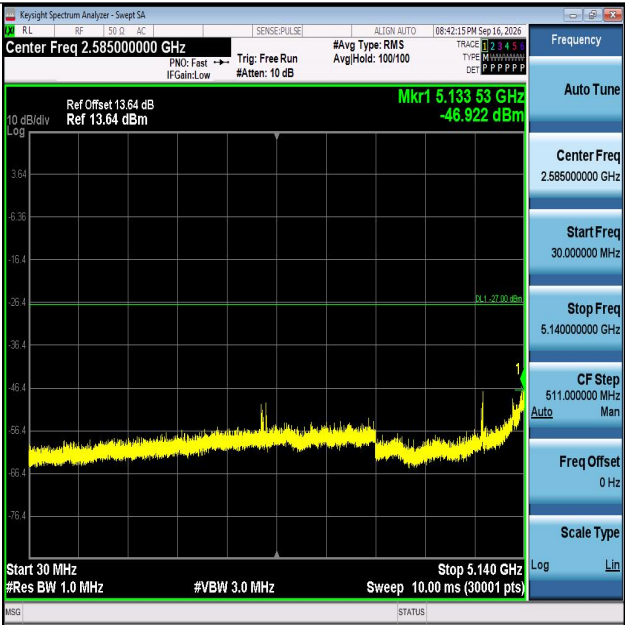
11AC20MIMO-Ant1-5180-30~5140-PASS
