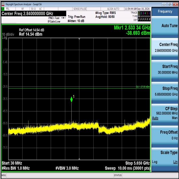
11N40MIMO-Ant2-5795-30~5650-PASS
