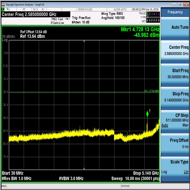
11AC20MIMO-Ant1-5200-30~5140-PASS
