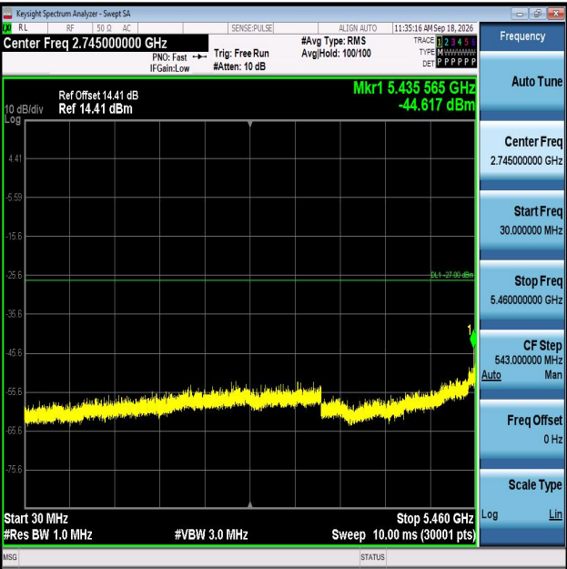
11N40MIMO-Ant2-5550-30~5460-PASS
