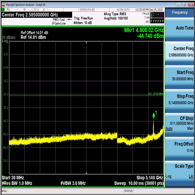
11AC20MIMO-Ant2-5280-30~5140-PASS
