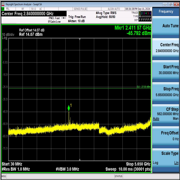
11N40MIMO-Ant1-5795-30~5650-PASS
