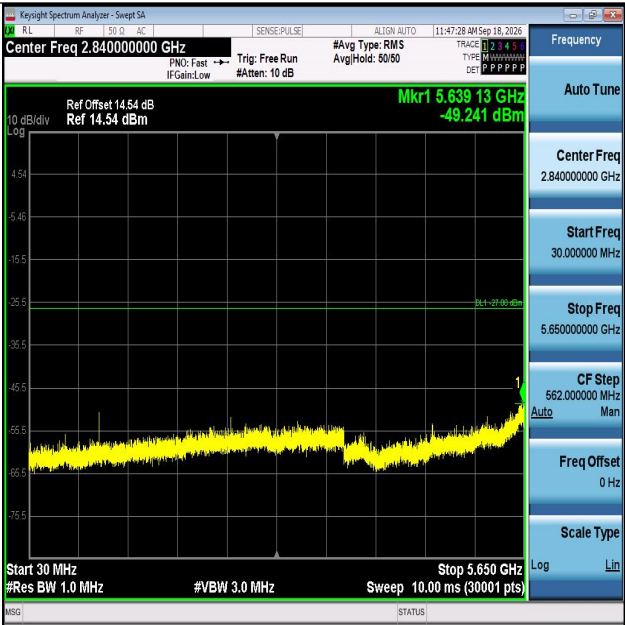
11N40MIMO-Ant2-5755-30~5650-PASS
