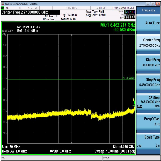
11N40MIMO-Ant2-5670-30~5460-PASS
