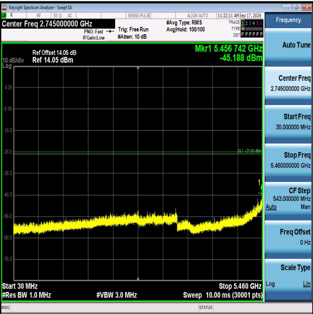
11AC40MIMO-Ant1-5510-30~5460-PASS
