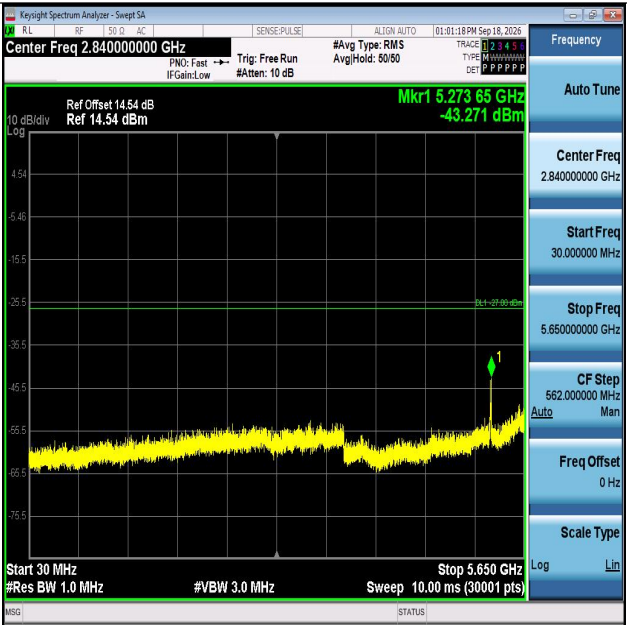
11AC20MIMO-Ant2-5745-30~5650-PASS
