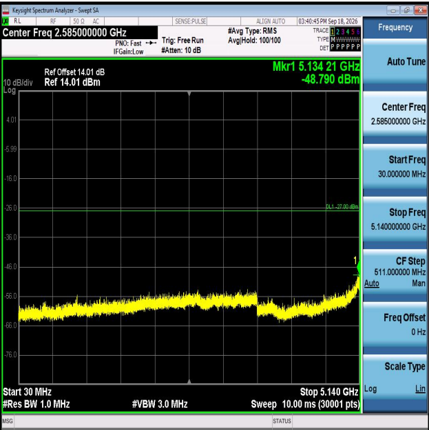
11AC40MIMO-Ant2-5270-30~5140-PASS
