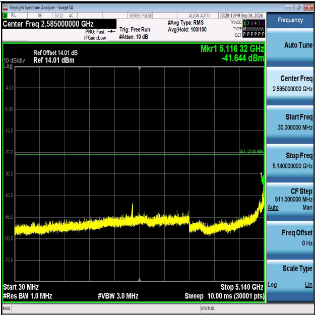
11AC40MIMO-Ant2-5190-30~5140-PASS
