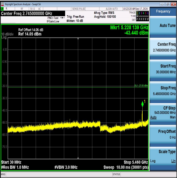
11AC20MIMO-Ant1-5700-30~5460-PASS
