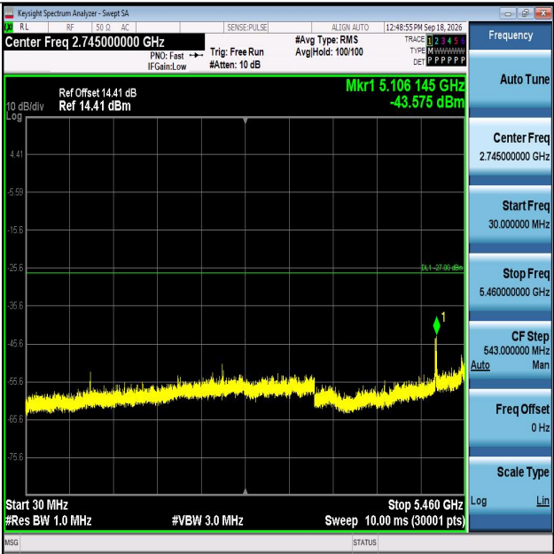
11AC20MIMO-Ant2-5580-30~5460-PASS
