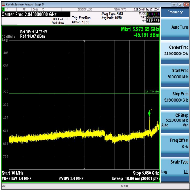
11AC20MIMO-Ant1-5745-30~5650-PASS
