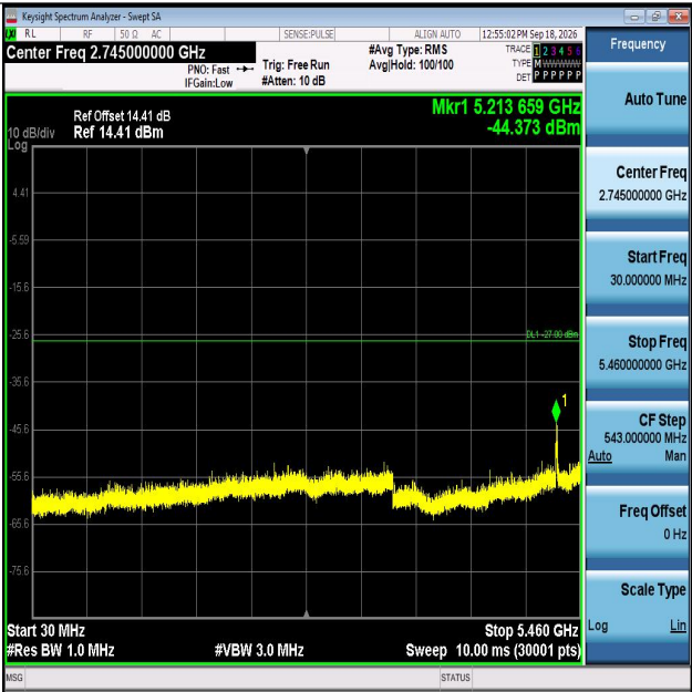
11AC20MIMO-Ant2-5700-30~5460-PASS
