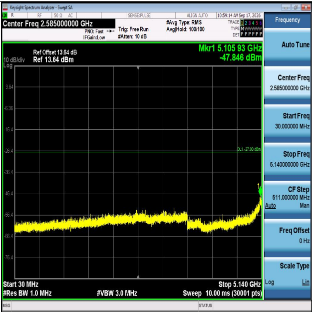
11AC40MIMO-Ant1-5270-30~5140-PASS
