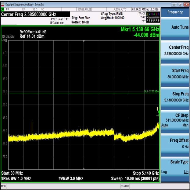
11AC40MIMO-Ant2-5230-30~5140-PASS
