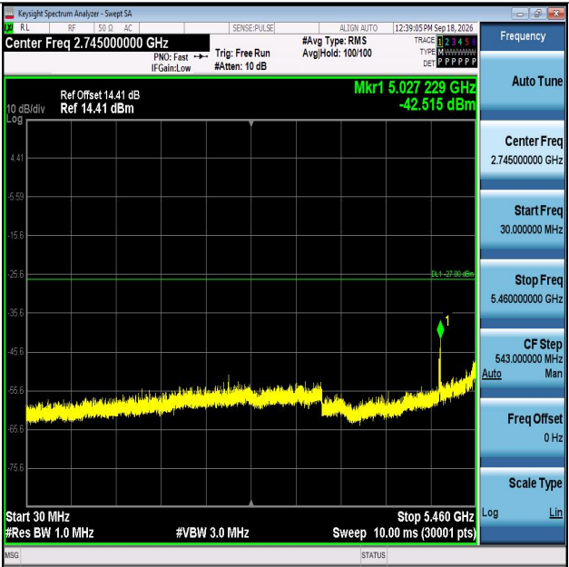
11AC20MIMO-Ant2-5500-30~5460-PASS
