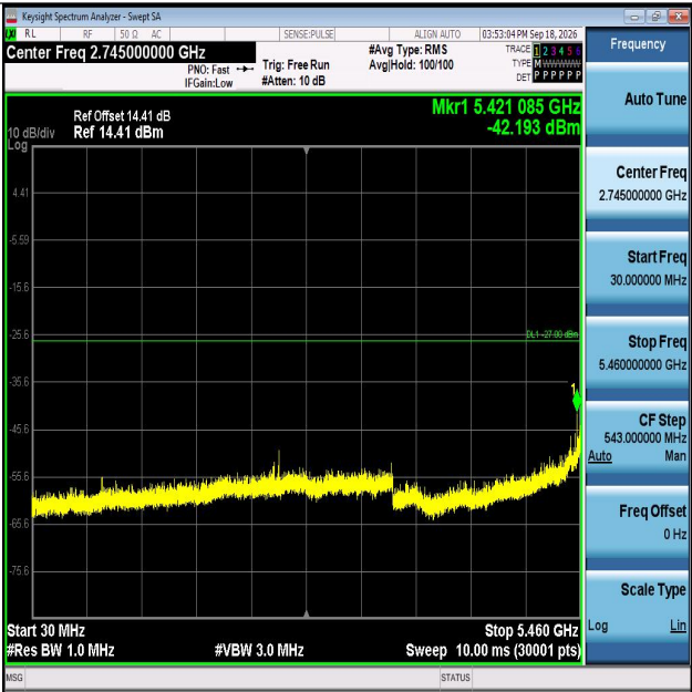
11AC40MIMO-Ant2-5510-30~5460-PASS
