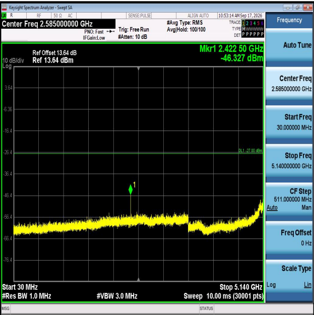
11AC40MIMO-Ant1-5230-30~5140-PASS
