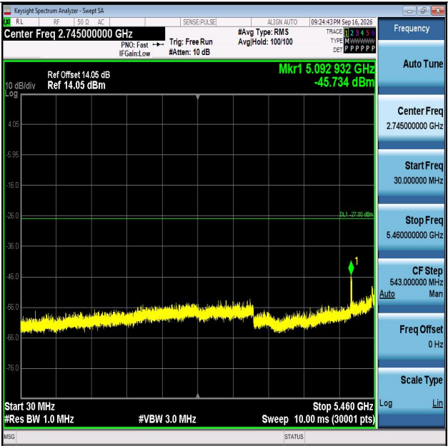
11AC20MIMO-Ant1-5580-30~5460-PASS
