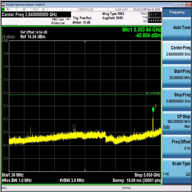
11AC20MIMO-Ant2-5825-30~5650-PASS
