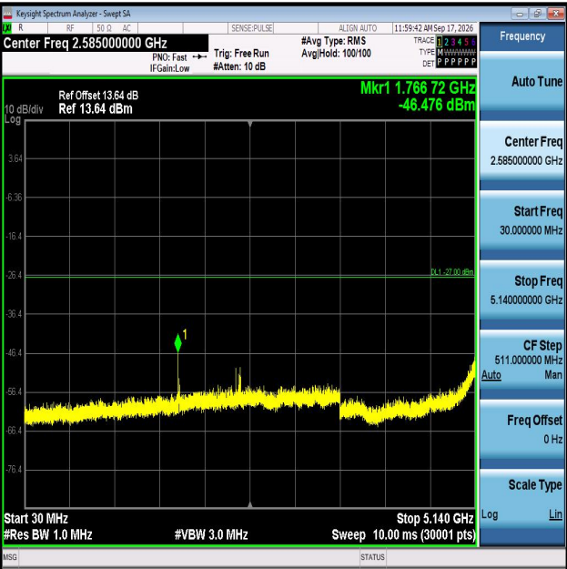
11AC80MIMO-Ant1-5290-30~5140-PASS
