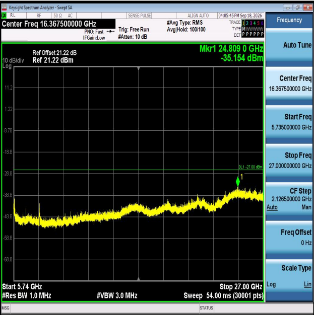
11AC40MIMO-Ant2-5670-5735~40000-PASS
