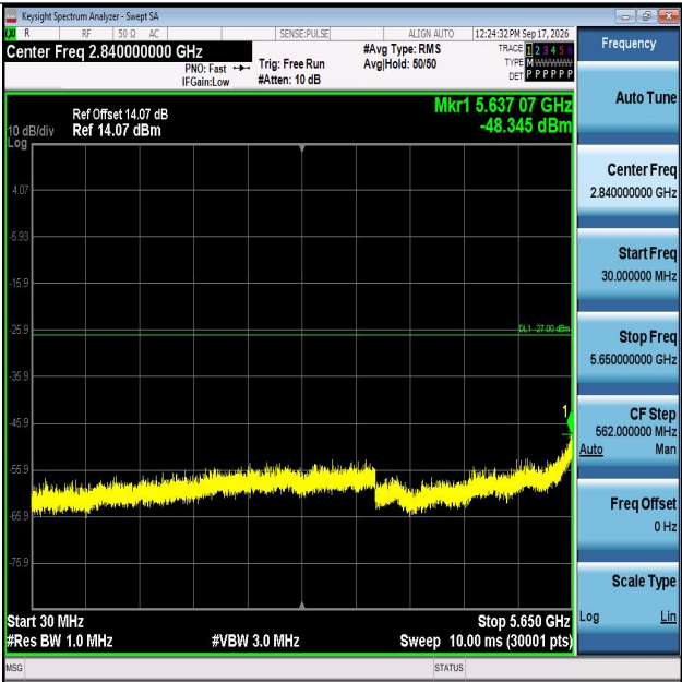
11AC80MIMO-Ant1-5775-30~5650-PASS
