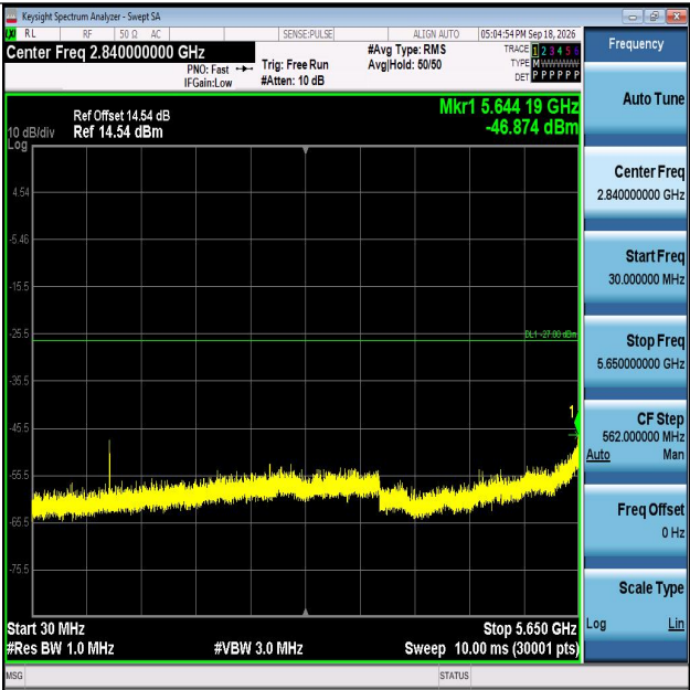
11AC80MIMO-Ant2-5775-30~5650-PASS
