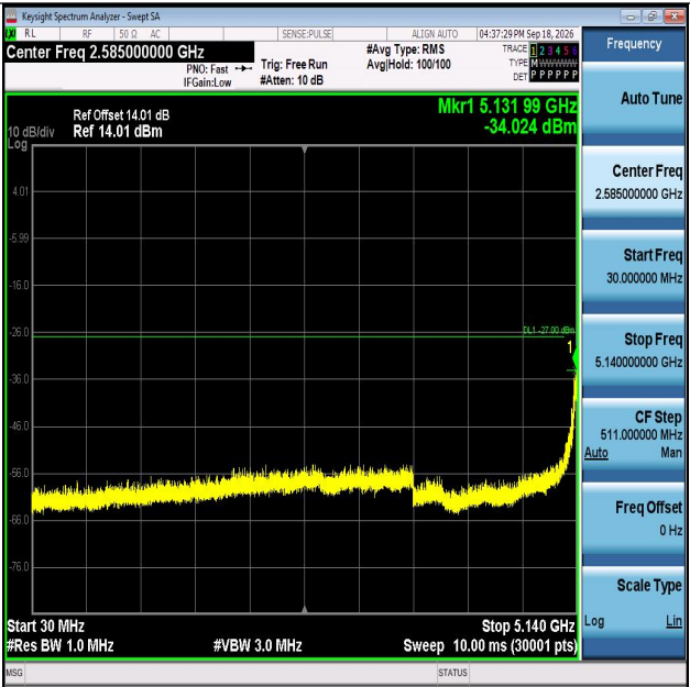
11AC80MIMO-Ant2-5210-30~5140-PASS
