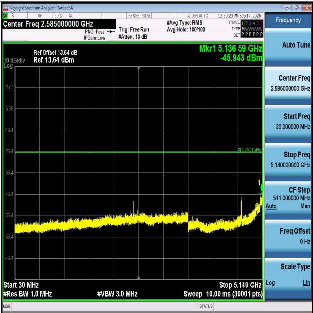
11AX20MIMO-Ant1-5180-30~5140-PASS
