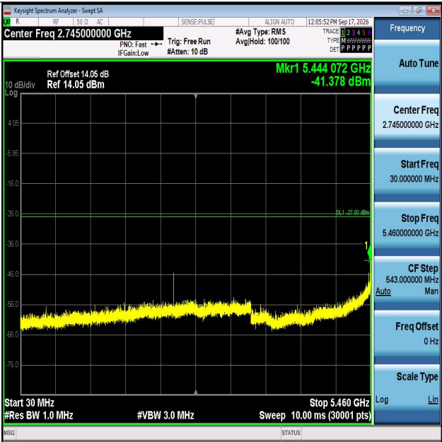
11AC80MIMO-Ant1-5530-30~5460-PASS
