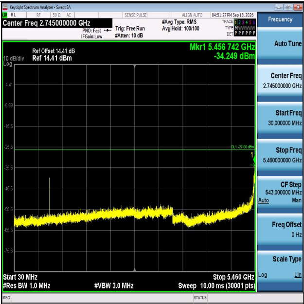
11AC80MIMO-Ant2-5530-30~5460-PASS
