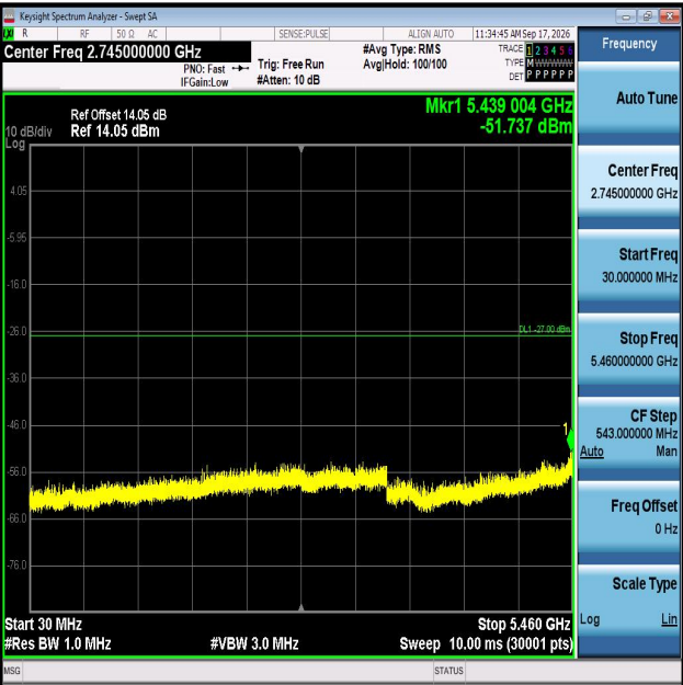
11AC40MIMO-Ant1-5670-30~5460-PASS
