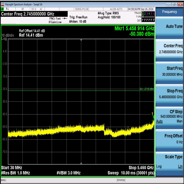
11AC80MIMO-Ant2-5610-30~5460-PASS
