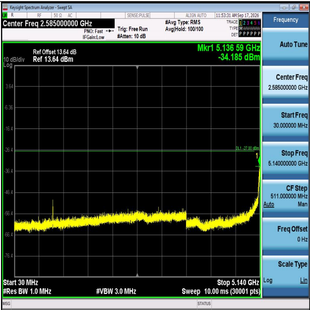
11AC80MIMO-Ant1-5210-30~5140-PASS
