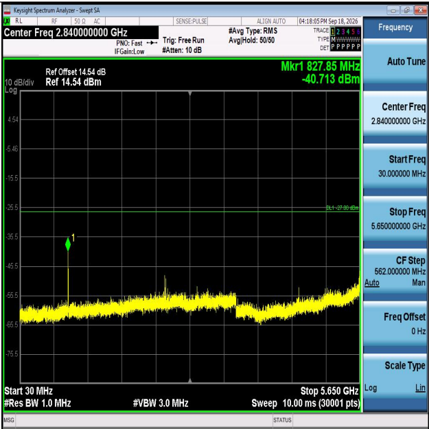
11AC40MIMO-Ant2-5795-30~5650-PASS
