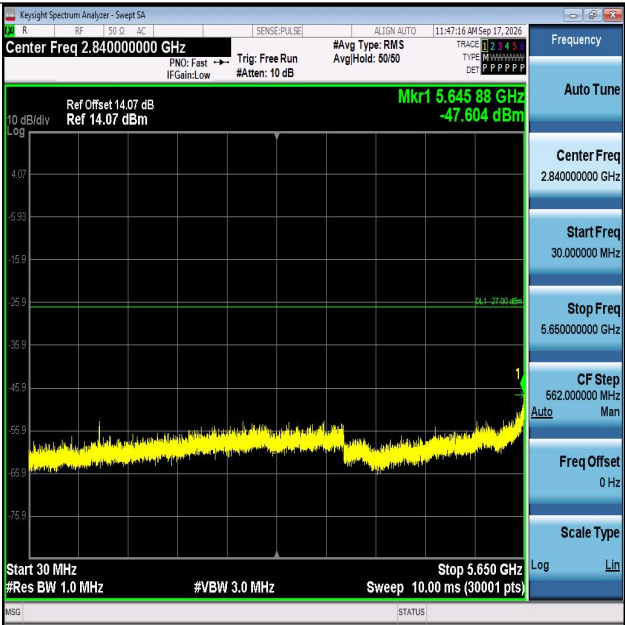
11AC40MIMO-Ant1-5795-30~5650-PASS
