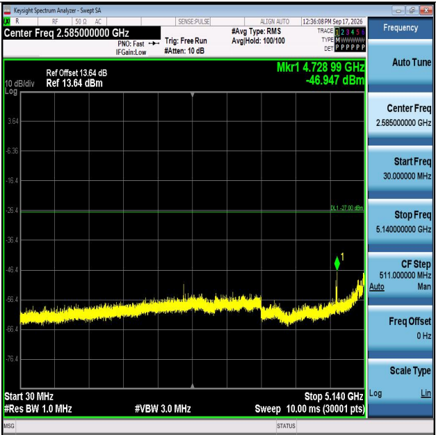
11AX20MIMO-Ant1-5200-30~5140-PASS
