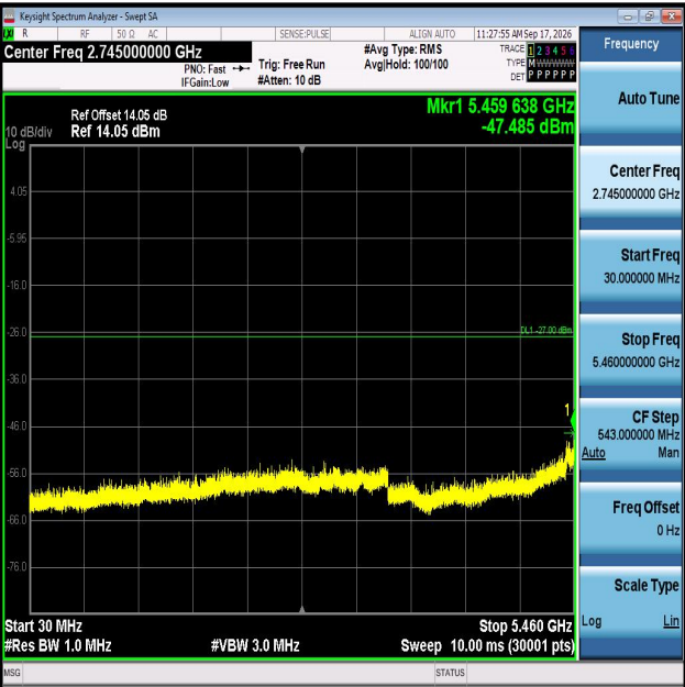
11AC40MIMO-Ant1-5550-30~5460-PASS
