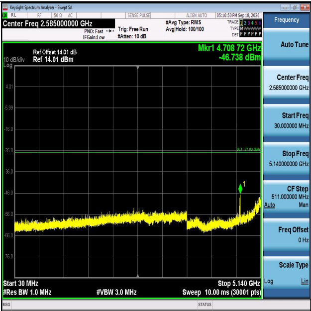
11AX20MIMO-Ant2-5180-30~5140-PASS
