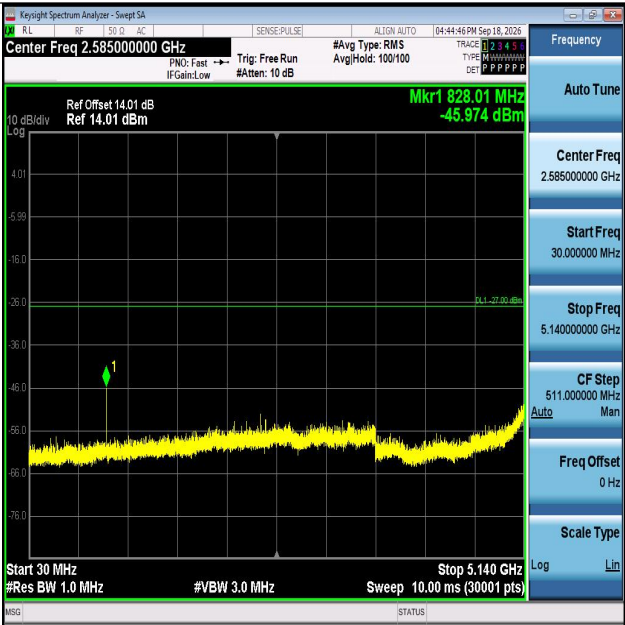
11AC80MIMO-Ant2-5290-30~5140-PASS
