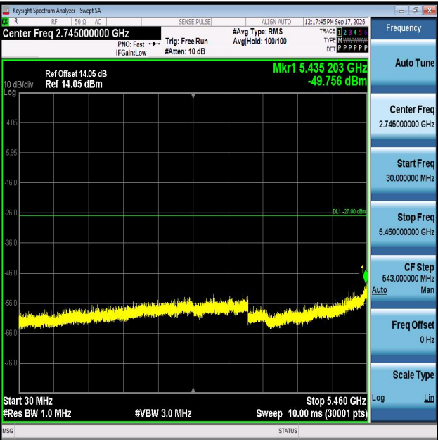
11AC80MIMO-Ant1-5610-30~5460-PASS
