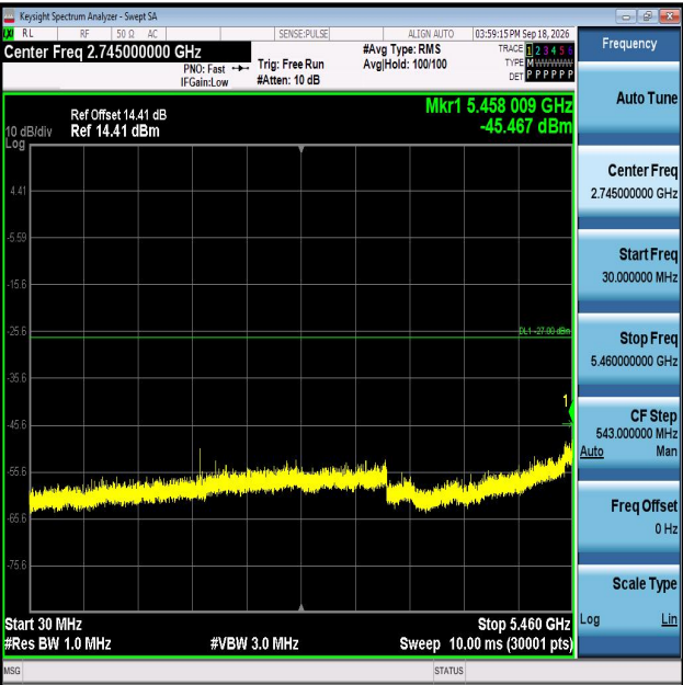
11AC40MIMO-Ant2-5550-30~5460-PASS
