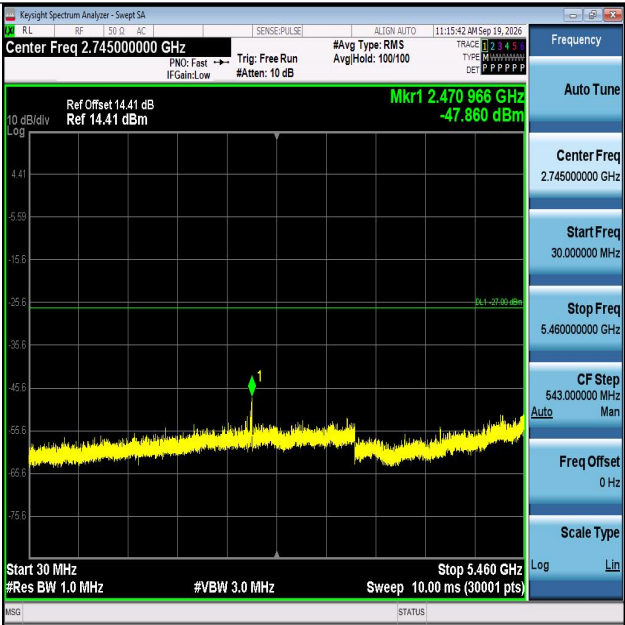
11AX40MIMO-Ant2-5670-30~5460-PASS
