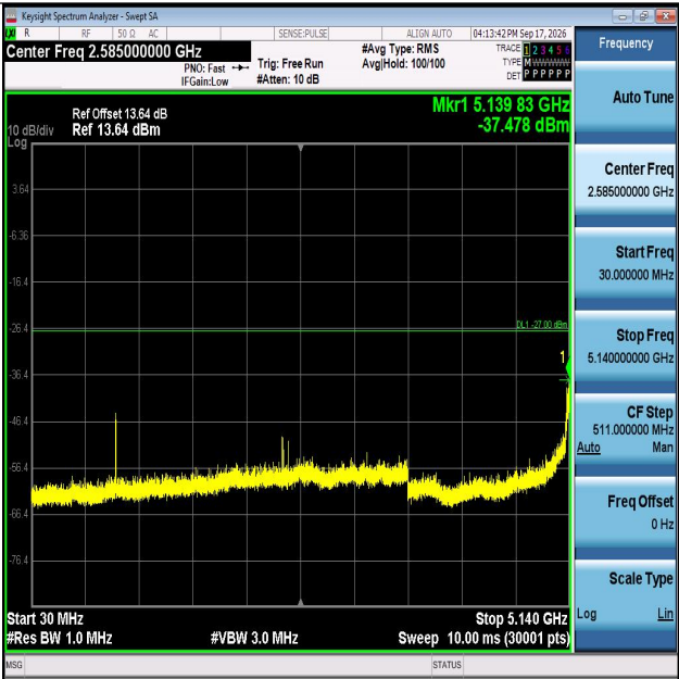
11AX80MIMO-Ant1-5210-30~5140-PASS
