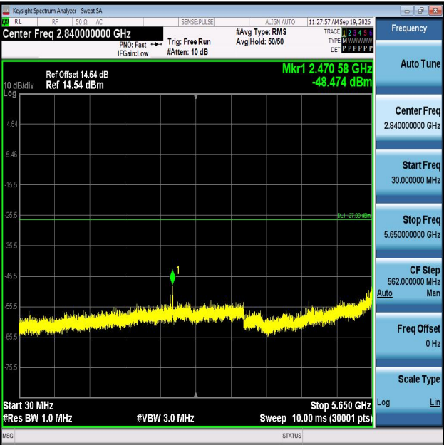
11AX40MIMO-Ant2-5795-30~5650-PASS
