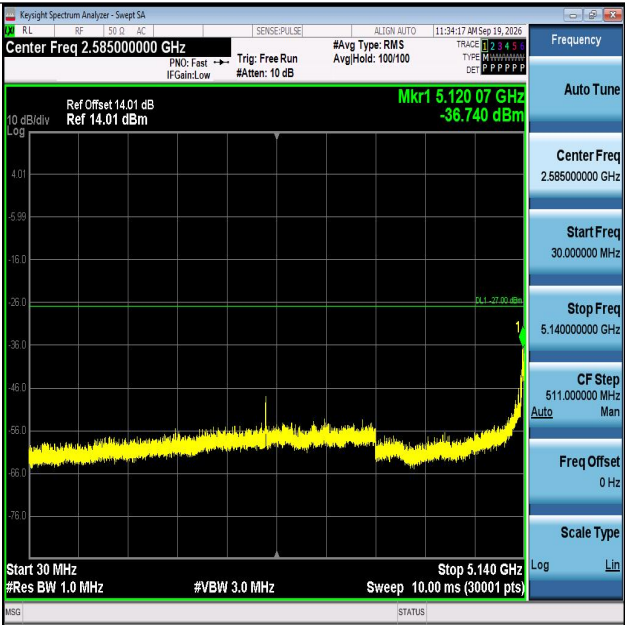
11AX80MIMO-Ant2-5210-30~5140-PASS
