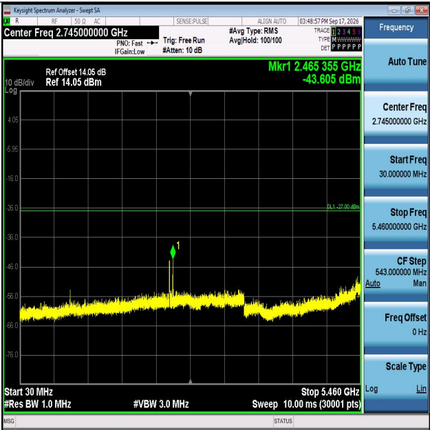
11AX40MIMO-Ant1-5550-30~5460-PASS
