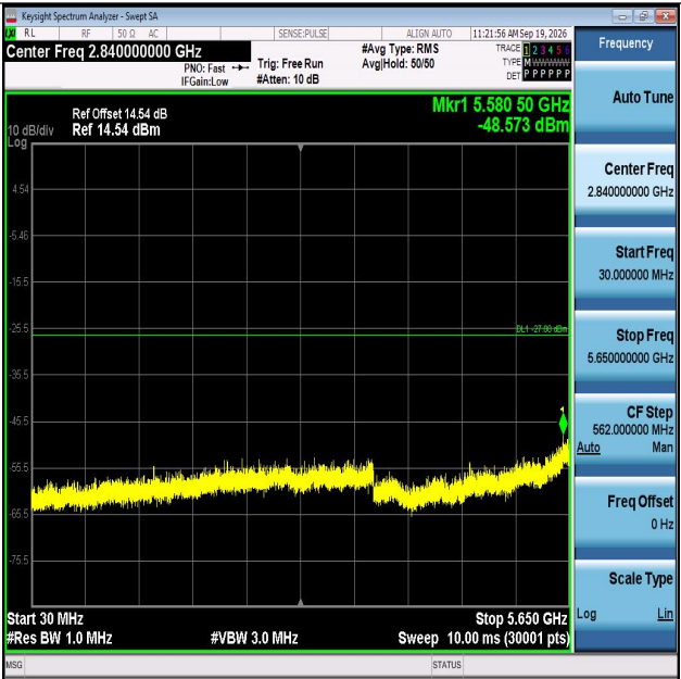
11AX40MIMO-Ant2-5755-30~5650-PASS
