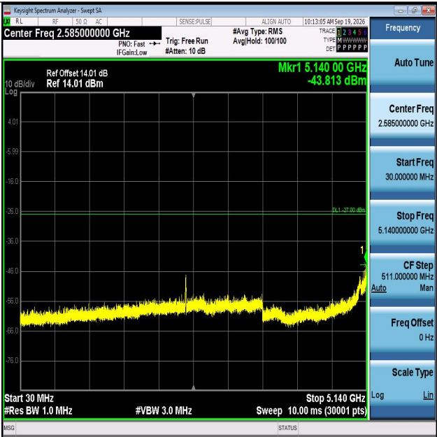
11AX40MIMO-Ant2-5190-30~5140-PASS
