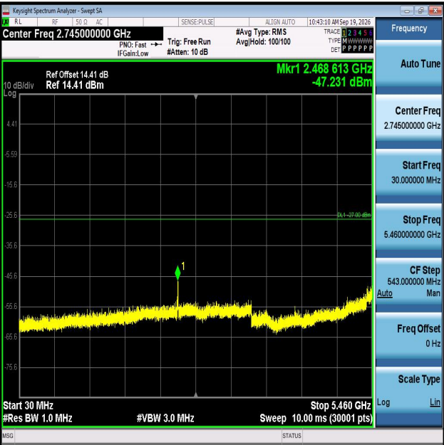
11AX40MIMO-Ant2-5550-30~5460-PASS
