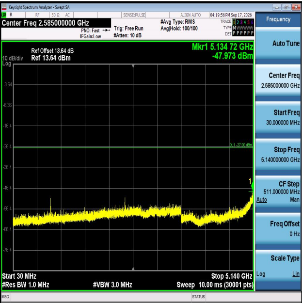
11AX80MIMO-Ant1-5290-30~5140-PASS
