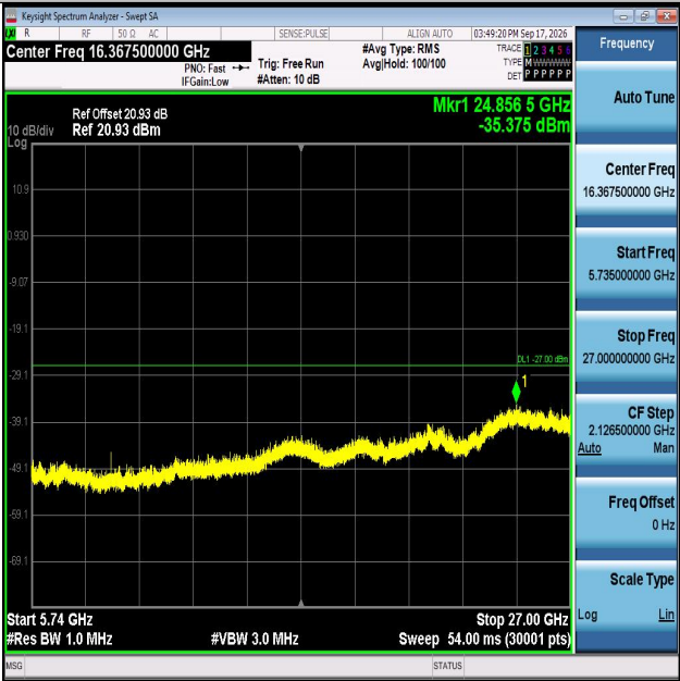
11AX40MIMO-Ant1-5550-5735~40000-PASS
