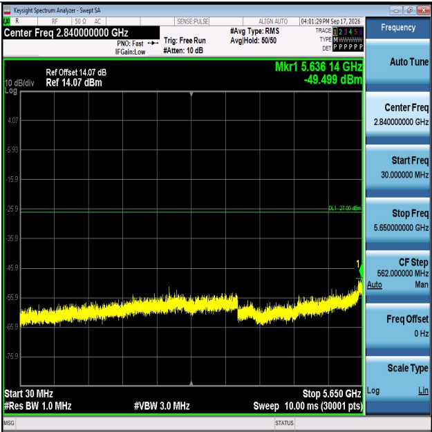
11AX40MIMO-Ant1-5755-30~5650-PASS
