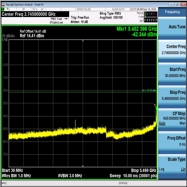
11AX40MIMO-Ant2-5510-30~5460-PASS
