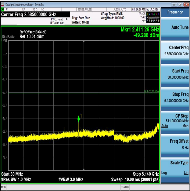
11AX40MIMO-Ant1-5230-30~5140-PASS
