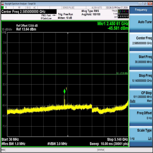
11AX40MIMO-Ant1-5310-30~5140-PASS
