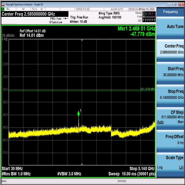
11AX40MIMO-Ant2-5310-30~5140-PASS
