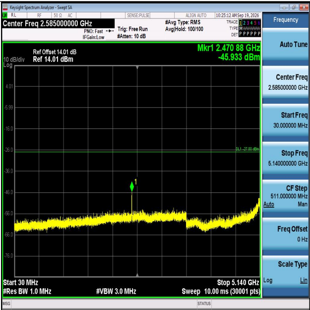
11AX40MIMO-Ant2-5270-30~5140-PASS
