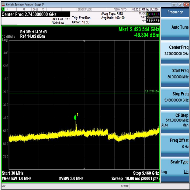
11AX40MIMO-Ant1-5670-30~5460-PASS
