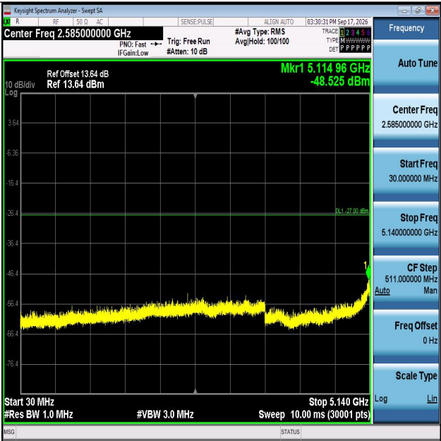
11AX40MIMO-Ant1-5270-30~5140-PASS
