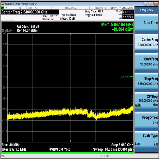
11AX40MIMO-Ant1-5795-30~5650-PASS
