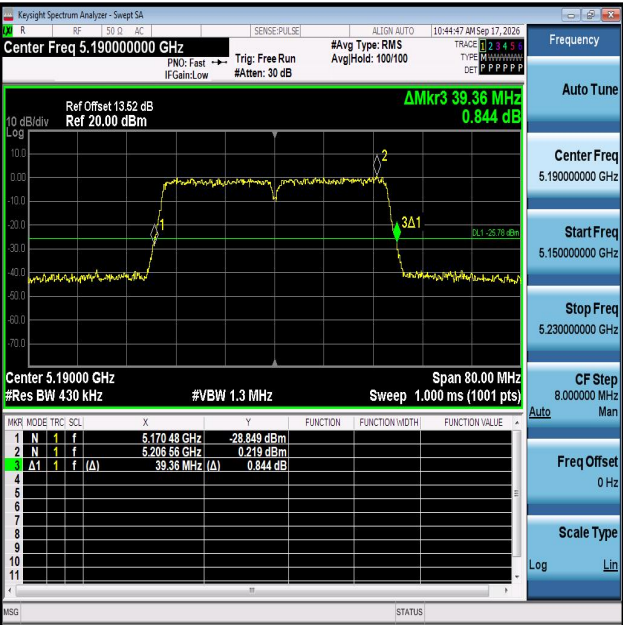
11AC40MIMO-Ant1-5190
