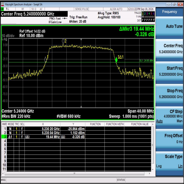
11AC20MIMO-Ant2-5240
