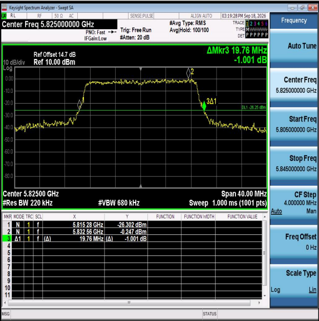
11AC20MIMO-Ant2-5825
