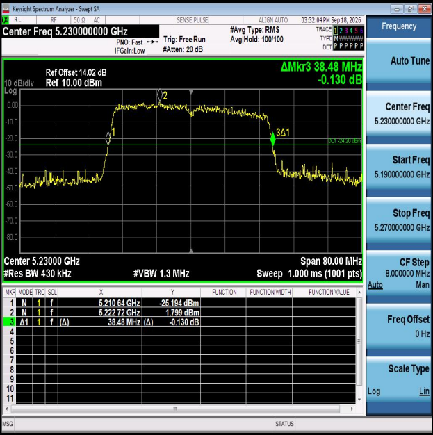
11AC40MIMO-Ant2-5230
