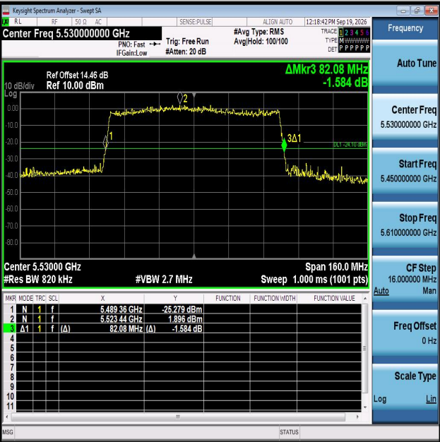
11AX80MIMO-Ant2-5530
