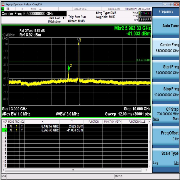
11AX20MIMO-Ant2-6435-3000~10000-PASS
