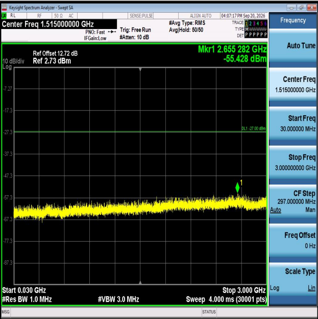
11AX20MIMO-Ant2-6175-30~3000-PASS
