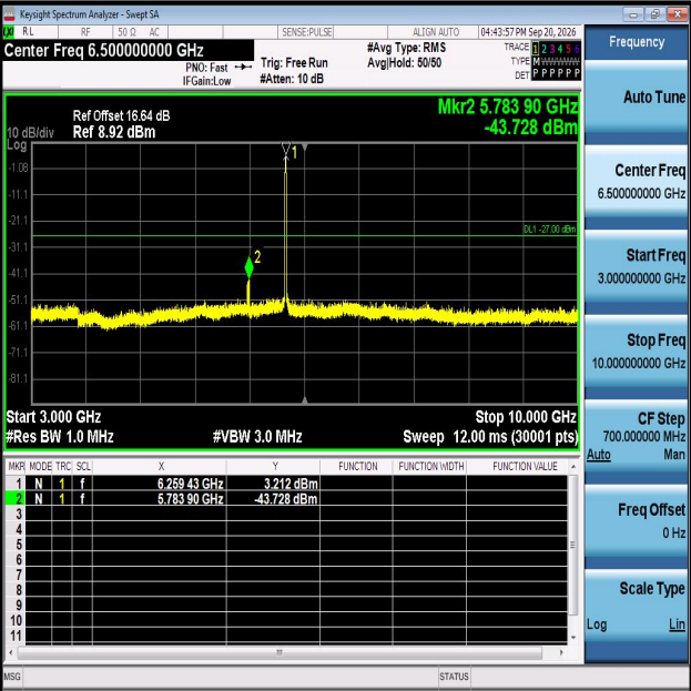
11AX20MIMO-Ant2-6255-3000~10000-PASS
