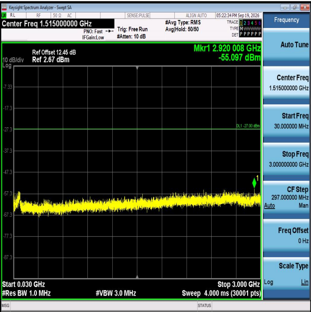
11AX20MIMO-Ant1-6255-30~3000-PASS
