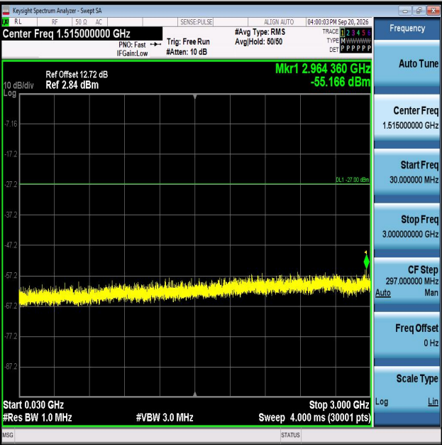
11AX20MIMO-Ant2-5955-30~3000-PASS
