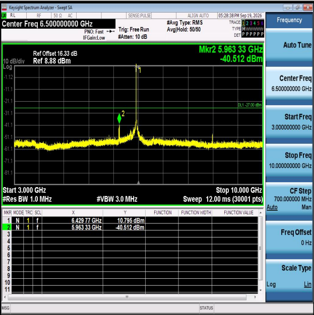
11AX20MIMO-Ant1-6435-3000~10000-PASS
