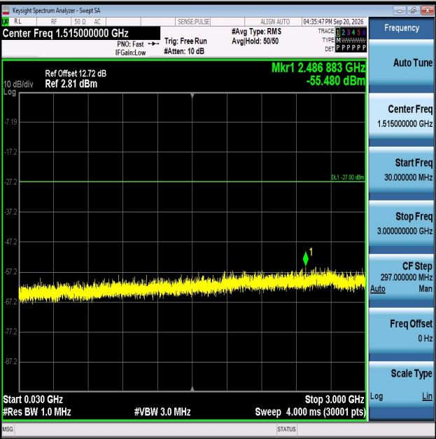
11AX20MIMO-Ant2-6115-30~3000-PASS
