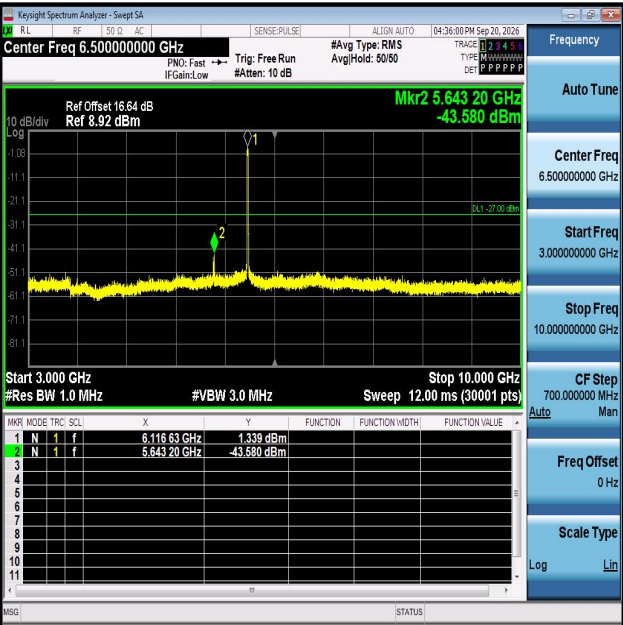
11AX20MIMO-Ant2-6115-3000~10000-PASS
