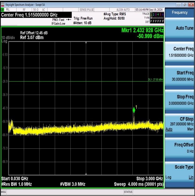
11AX20MIMO-Ant1-6115-30~3000-PASS
