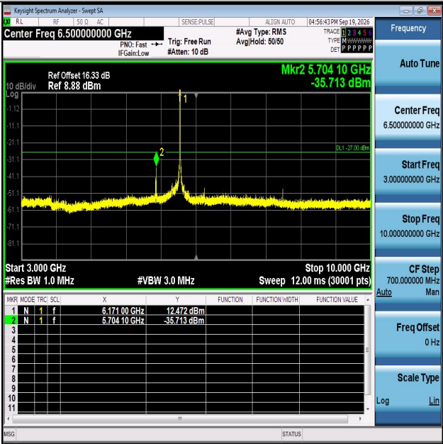
11AX20MIMO-Ant1-6175-3000~10000-PASS
