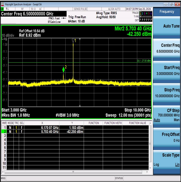
11AX20MIMO-Ant2-6175-3000~10000-PASS
