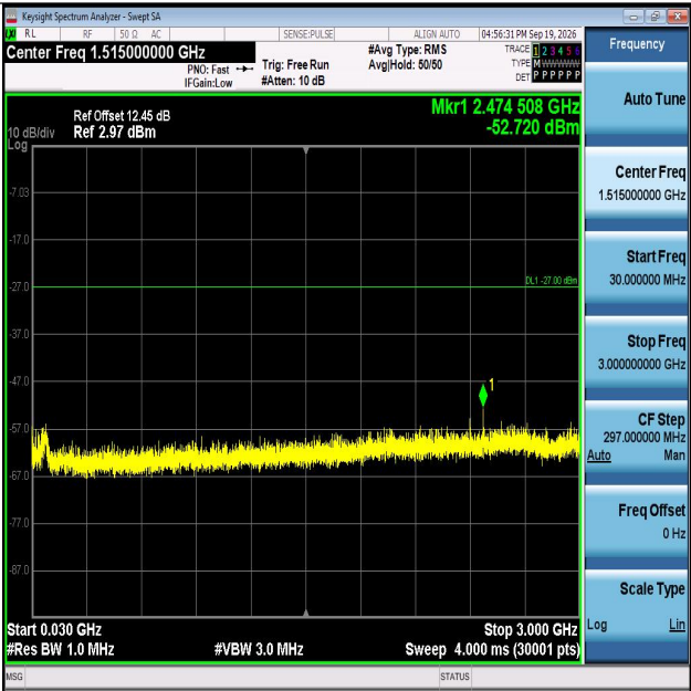
11AX20MIMO-Ant1-6175-30~3000-PASS
