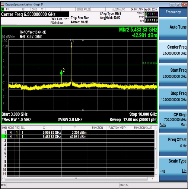
11AX20MIMO-Ant2-5955-3000~10000-PASS
