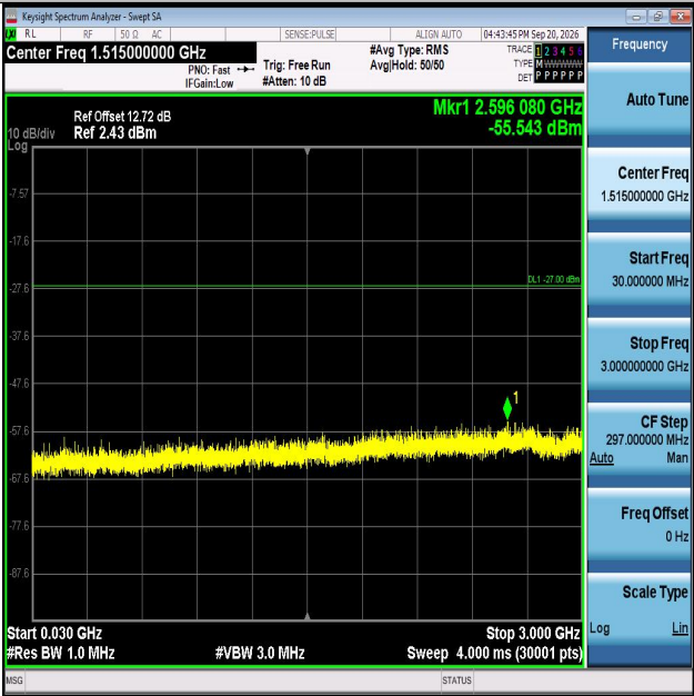
11AX20MIMO-Ant2-6255-30~3000-PASS
