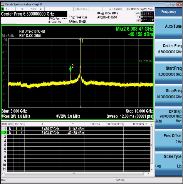
11AX20MIMO-Ant1-6475-3000~10000-PASS
