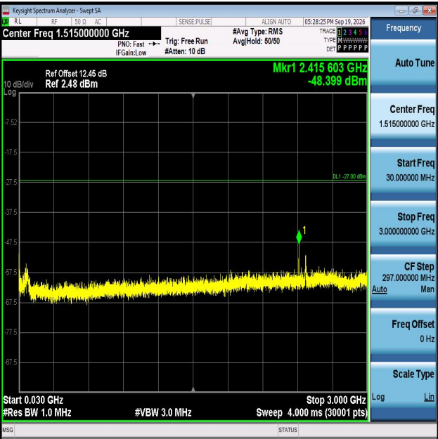
11AX20MIMO-Ant1-6435-30~3000-PASS
