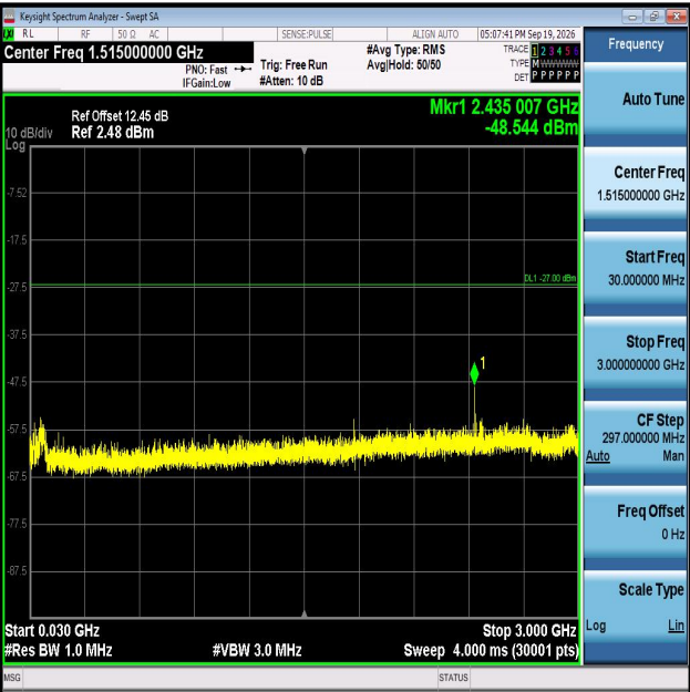
11AX20MIMO-Ant1-6415-30~3000-PASS
