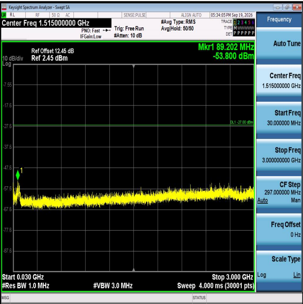
11AX20MIMO-Ant1-6475-30~3000-PASS
