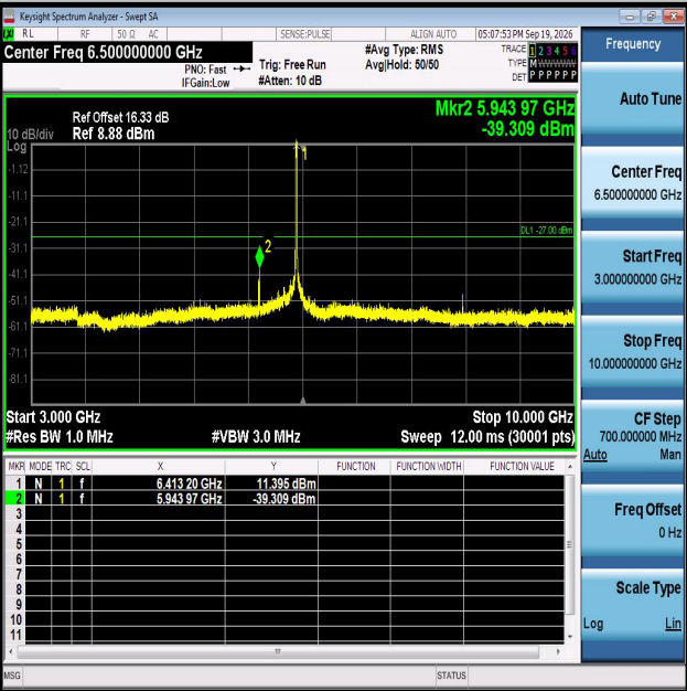
11AX20MIMO-Ant1-6415-3000~10000-PASS
