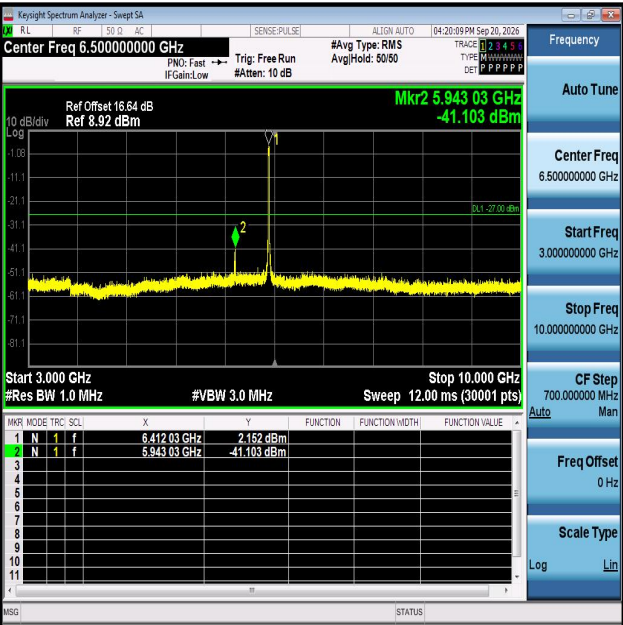
11AX20MIMO-Ant2-6415-3000~10000-PASS
