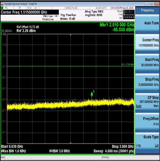
11AX20MIMO-Ant2-6415-30~3000-PASS
