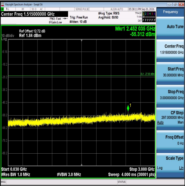
11AX20MIMO-Ant2-6895-30~3000-PASS
