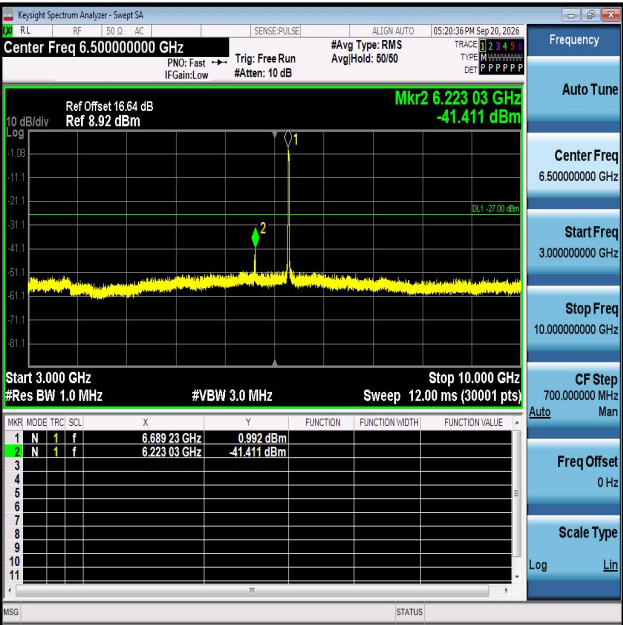
11AX20MIMO-Ant2-6695-3000~10000-PASS
