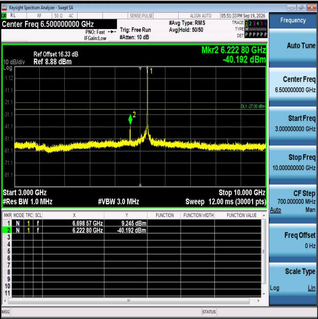
11AX20MIMO-Ant1-6695-3000~10000-PASS
