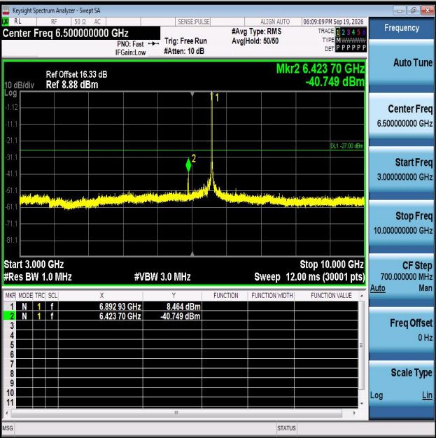
11AX20MIMO-Ant1-6895-3000~10000-PASS
