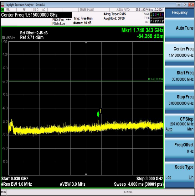
11AX20MIMO-Ant1-6695-30~3000-PASS
