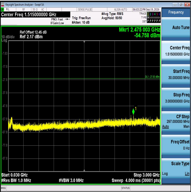
11AX20MIMO-Ant1-6875-30~3000-PASS
