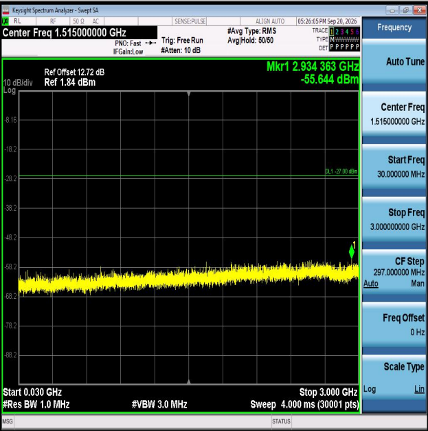
11AX20MIMO-Ant2-6855-30~3000-PASS
