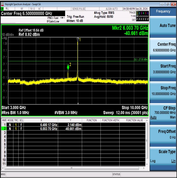
11AX20MIMO-Ant2-6475-3000~10000-PASS
