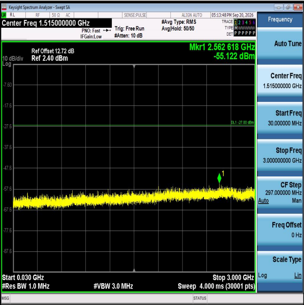
11AX20MIMO-Ant2-6535-30~3000-PASS
