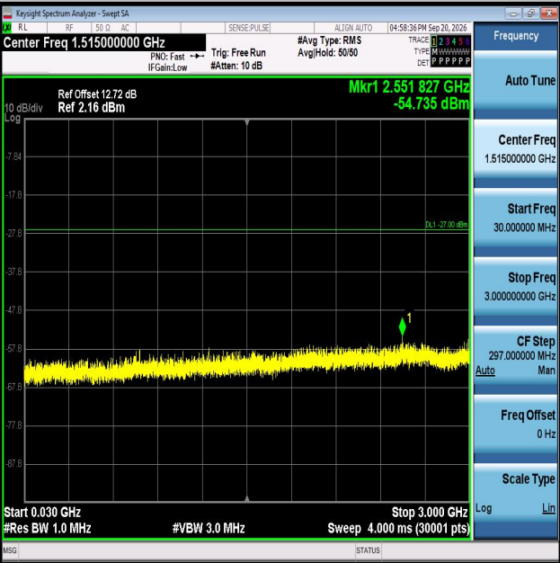
11AX20MIMO-Ant2-6475-30~3000-PASS
