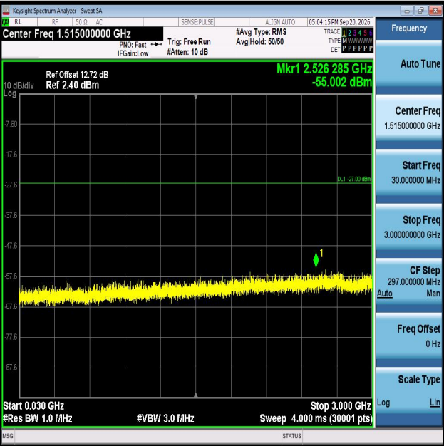
11AX20MIMO-Ant2-6515-30~3000-PASS
