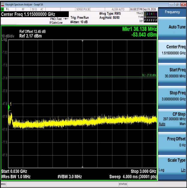
11AX20MIMO-Ant1-6895-30~3000-PASS
