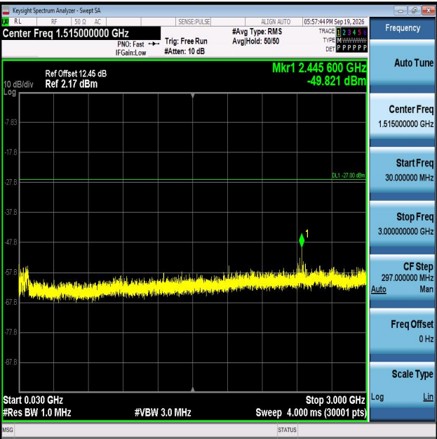
11AX20MIMO-Ant1-6855-30~3000-PASS
