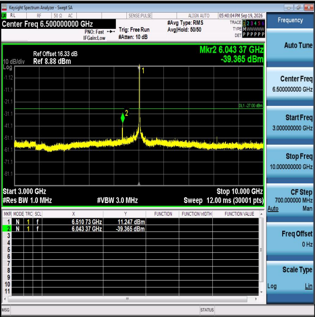
11AX20MIMO-Ant1-6515-3000~10000-PASS
