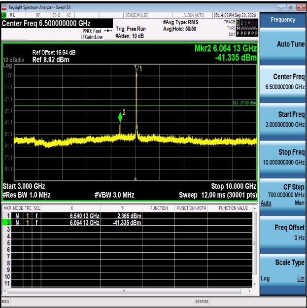
11AX20MIMO-Ant2-6535-3000~10000-PASS
