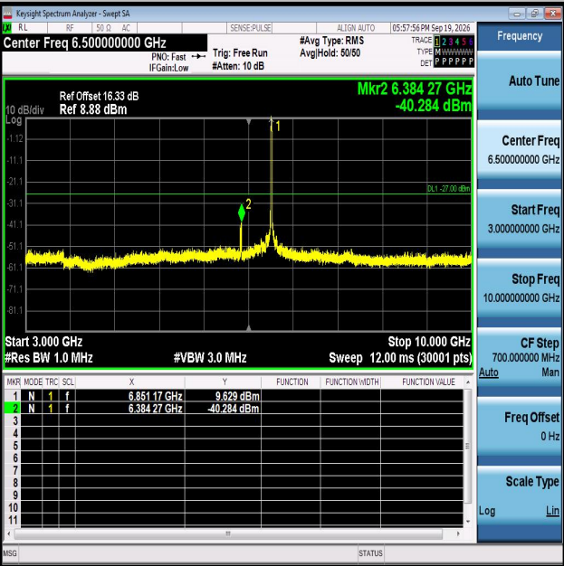
11AX20MIMO-Ant1-6855-3000~10000-PASS
