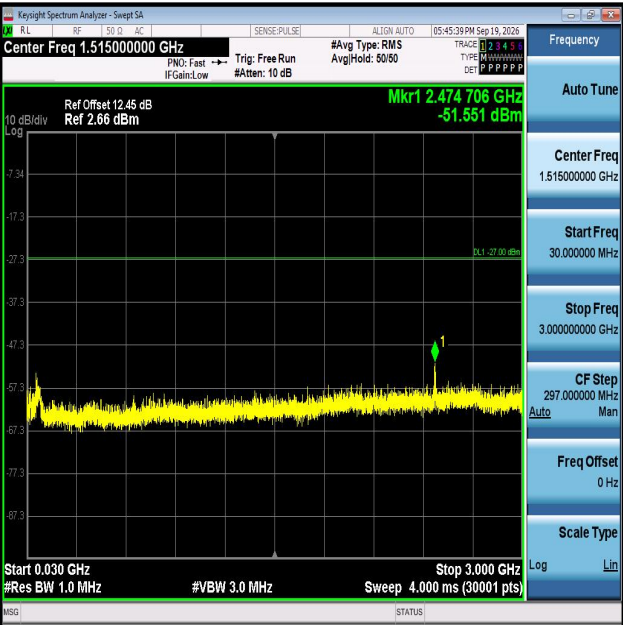
11AX20MIMO-Ant1-6535-30~3000-PASS
