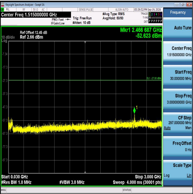
11AX20MIMO-Ant1-6515-30~3000-PASS
