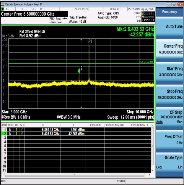
11AX20MIMO-Ant2-6875-3000~10000-PASS
