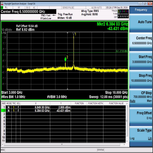
11AX20MIMO-Ant2-6855-3000~10000-PASS
