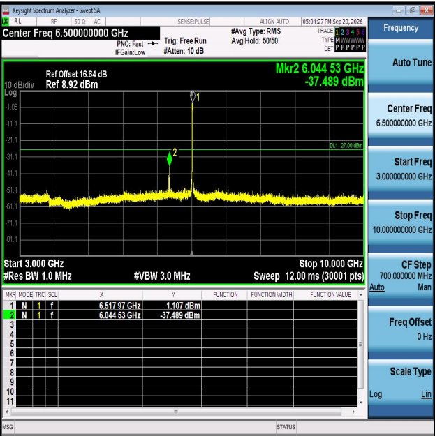
11AX20MIMO-Ant2-6515-3000~10000-PASS
