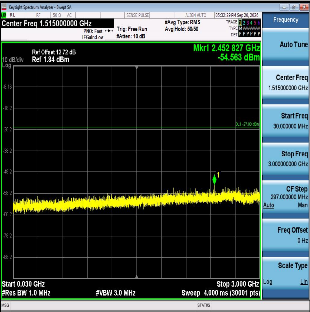
11AX20MIMO-Ant2-6875-30~3000-PASS
