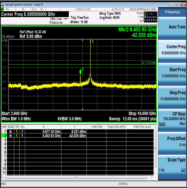
11AX20MIMO-Ant1-6875-3000~10000-PASS
