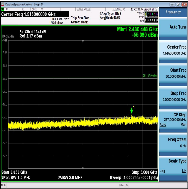
11AX40MIMO-Ant1-6885-30~3000-PASS
