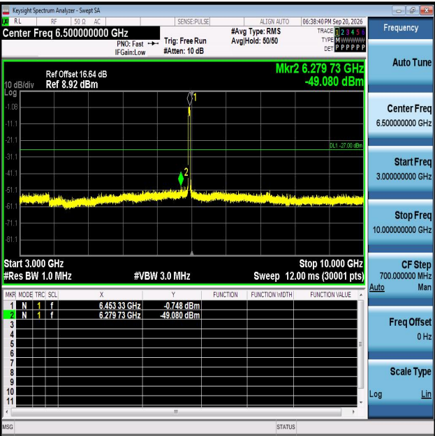
11AX40MIMO-Ant2-6445-3000~10000-PASS
