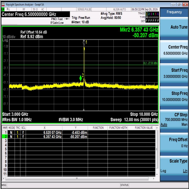
11AX40MIMO-Ant2-6525-3000~10000-PASS
