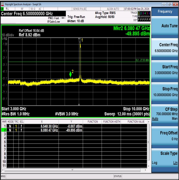
11AX40MIMO-Ant2-6565-3000~10000-PASS
