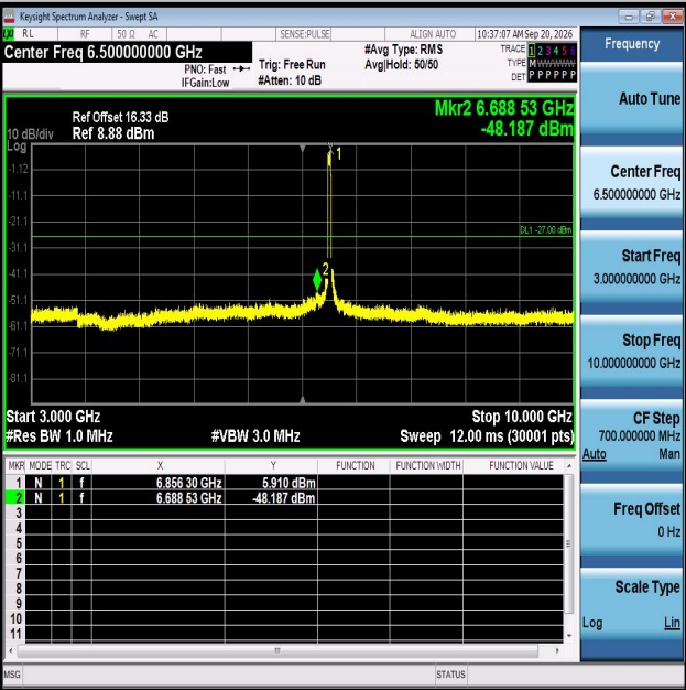
11AX40MIMO-Ant1-6845-3000~10000-PASS
