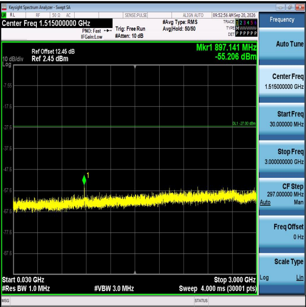
11AX40MIMO-Ant1-6485-30~3000-PASS
