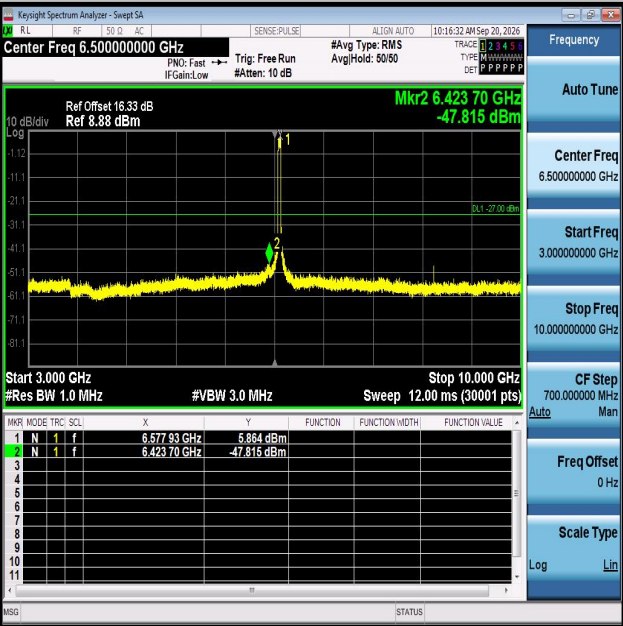
11AX40MIMO-Ant1-6565-3000~10000-PASS
