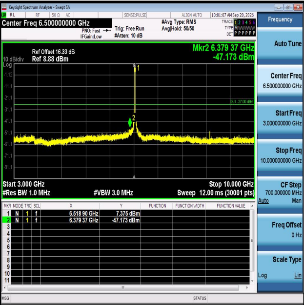
11AX40MIMO-Ant1-6525-3000~10000-PASS
