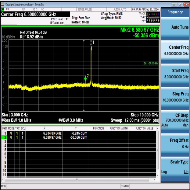
11AX40MIMO-Ant2-6845-3000~10000-PASS
