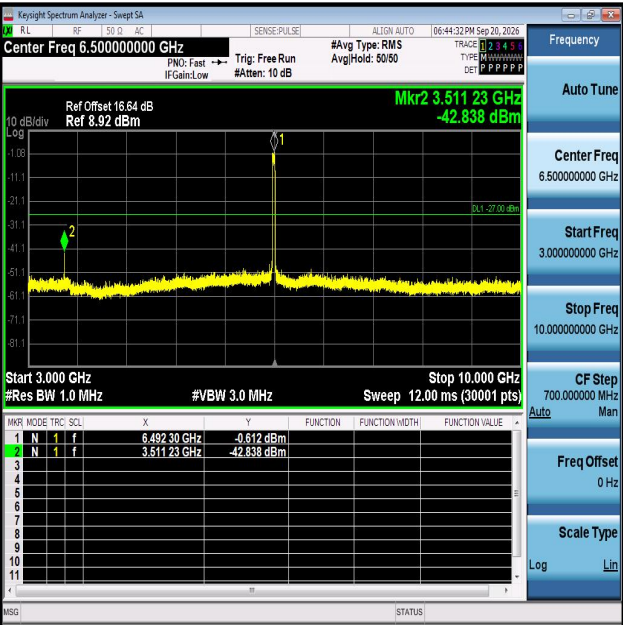
11AX40MIMO-Ant2-6485-3000~10000-PASS
