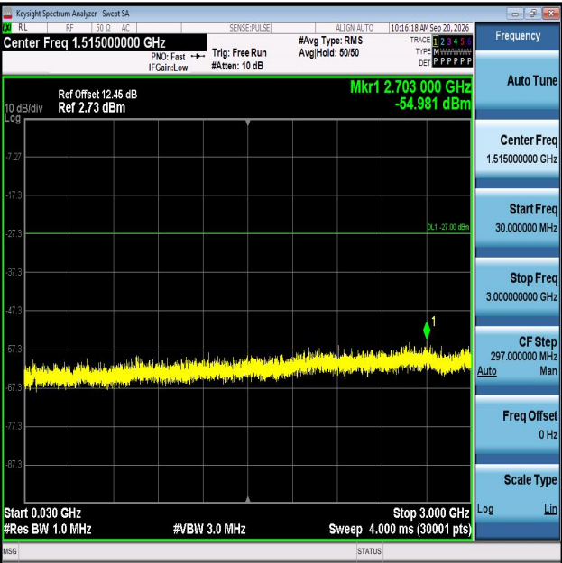
11AX40MIMO-Ant1-6565-30~3000-PASS
