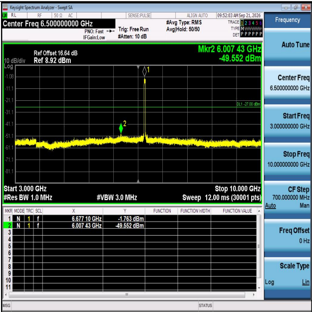
11AX40MIMO-Ant2-6685-3000~10000-PASS
