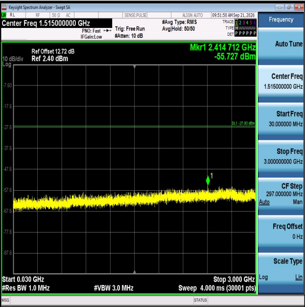
11AX40MIMO-Ant2-6685-30~3000-PASS
