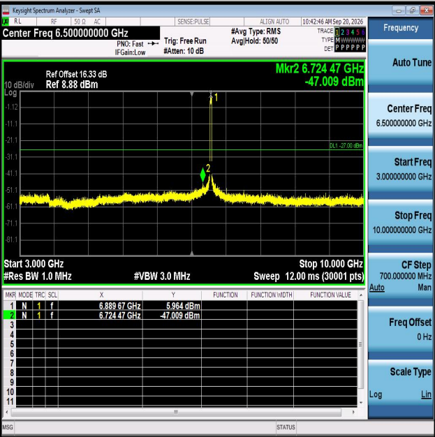
11AX40MIMO-Ant1-6885-3000~10000-PASS
