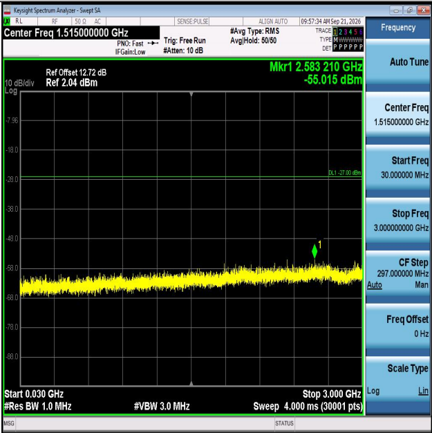
11AX40MIMO-Ant2-6845-30~3000-PASS
