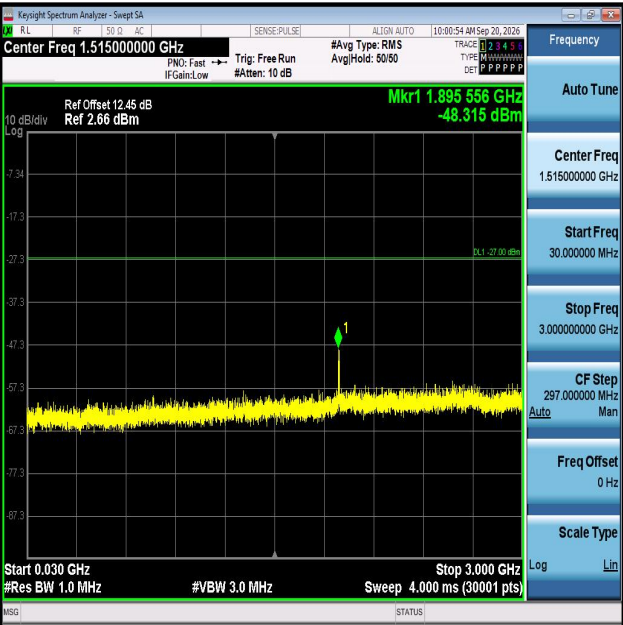
11AX40MIMO-Ant1-6525-30~3000-PASS
