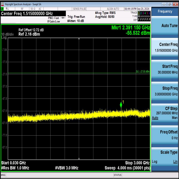
11AX40MIMO-Ant2-6485-30~3000-PASS
