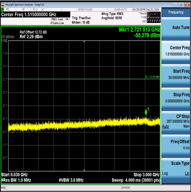
11AX40MIMO-Ant2-6445-30~3000-PASS
