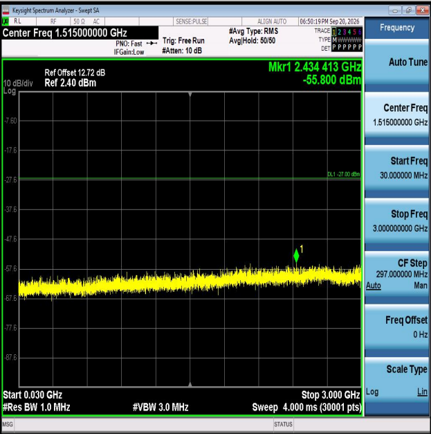
11AX40MIMO-Ant2-6525-30~3000-PASS
