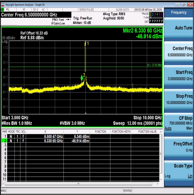
11AX40MIMO-Ant1-6485-3000~10000-PASS
