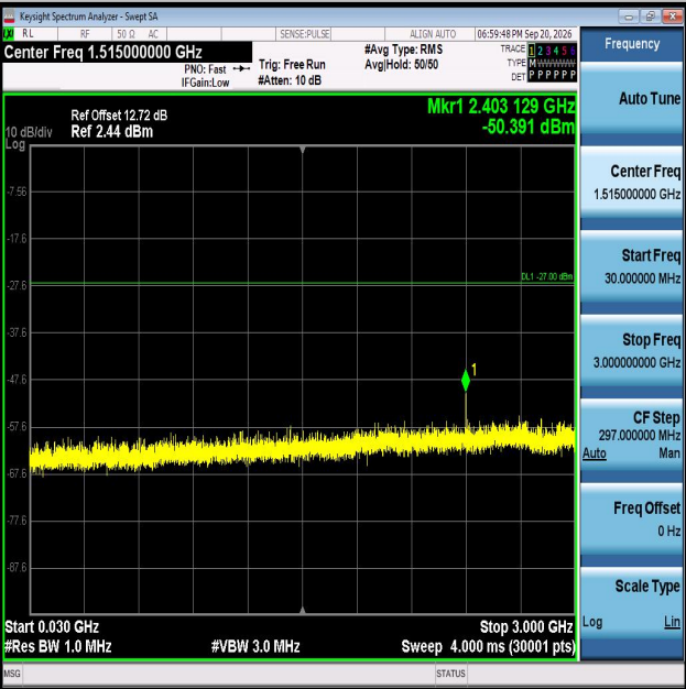
11AX40MIMO-Ant2-6565-30~3000-PASS
