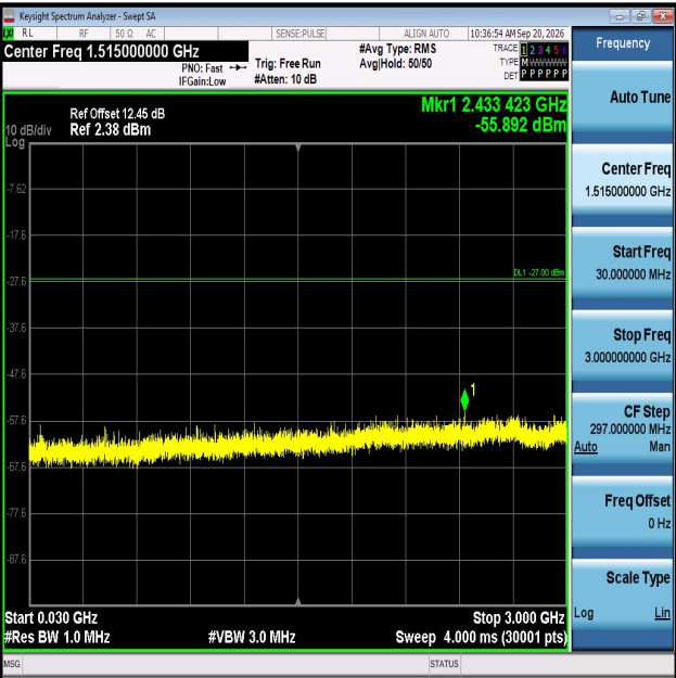
11AX40MIMO-Ant1-6845-30~3000-PASS
