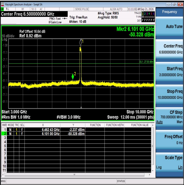
11AX80MIMO-Ant2-6465-3000~10000-PASS
