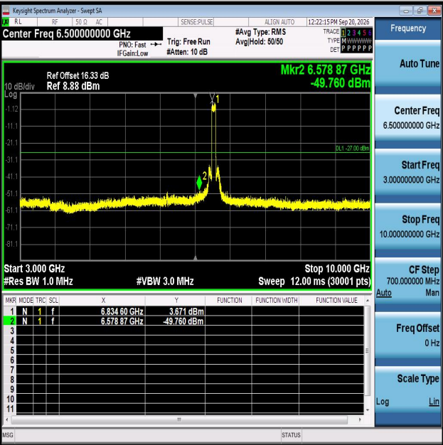
11AX80MIMO-Ant1-6865-3000~10000-PASS
