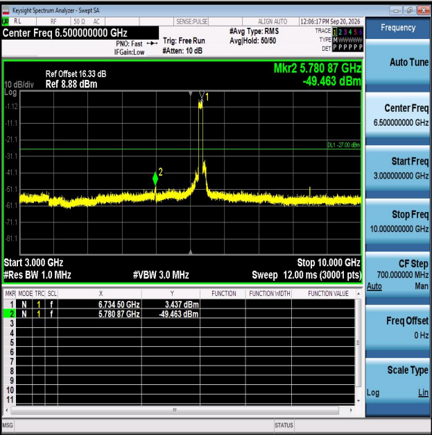
11AX80MIMO-Ant1-6705-3000~10000-PASS
