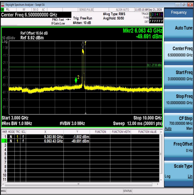
11AX80MIMO-Ant2-6385-3000~10000-PASS
