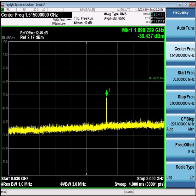
11AX80MIMO-Ant1-6865-30~3000-PASS
