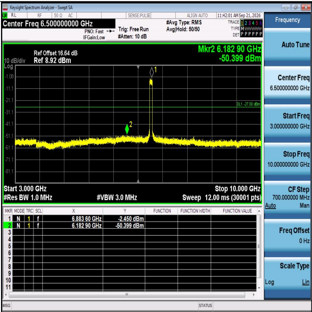
11AX80MIMO-Ant2-6865-3000~10000-PASS
