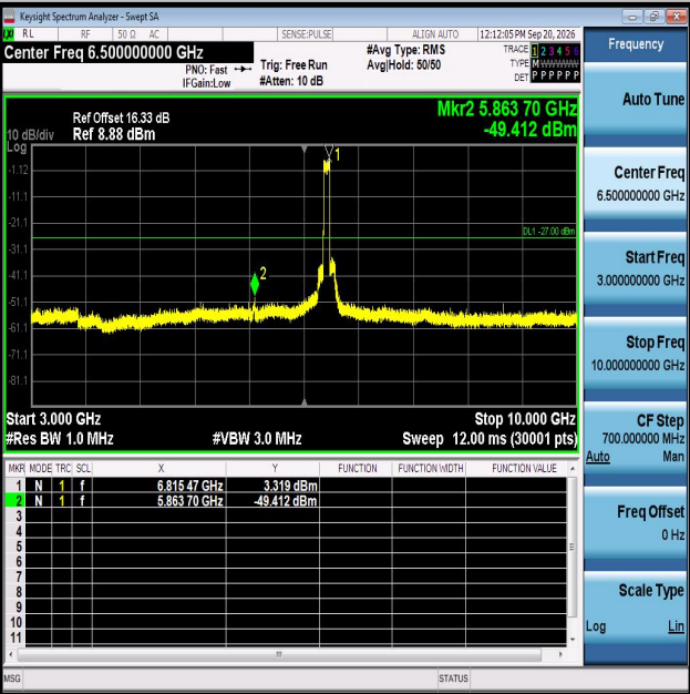
11AX80MIMO-Ant1-6785-3000~10000-PASS
