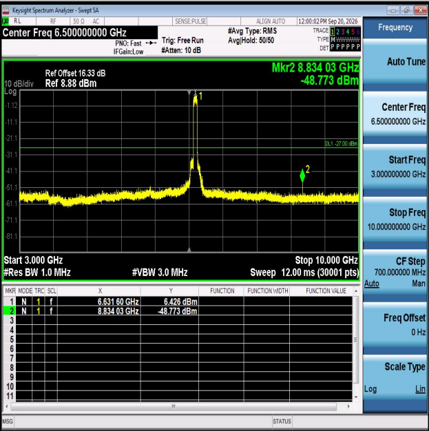
11AX80MIMO-Ant1-6625-3000~10000-PASS
