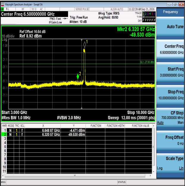
11AX80MIMO-Ant2-6625-3000~10000-PASS
