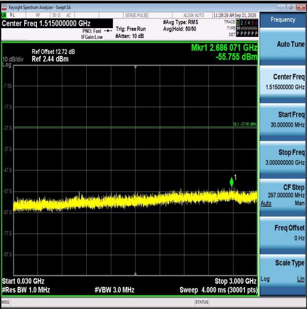
11AX80MIMO-Ant2-6705-30~3000-PASS
