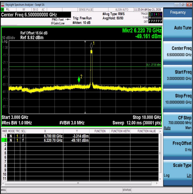
11AX80MIMO-Ant2-6785-3000~10000-PASS
