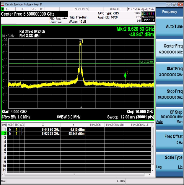
11AX80MIMO-Ant1-6465-3000~10000-PASS
