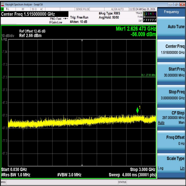
11AX80MIMO-Ant1-6545-30~3000-PASS
