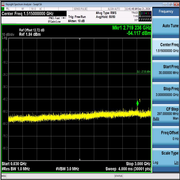
11AX80MIMO-Ant2-6865-30~3000-PASS
