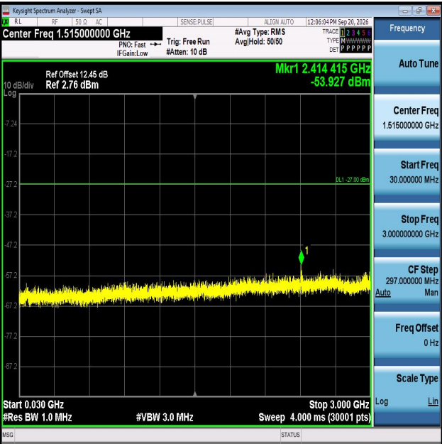
11AX80MIMO-Ant1-6705-30~3000-PASS
