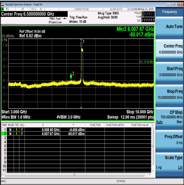
11AX80MIMO-Ant2-6545-3000~10000-PASS
