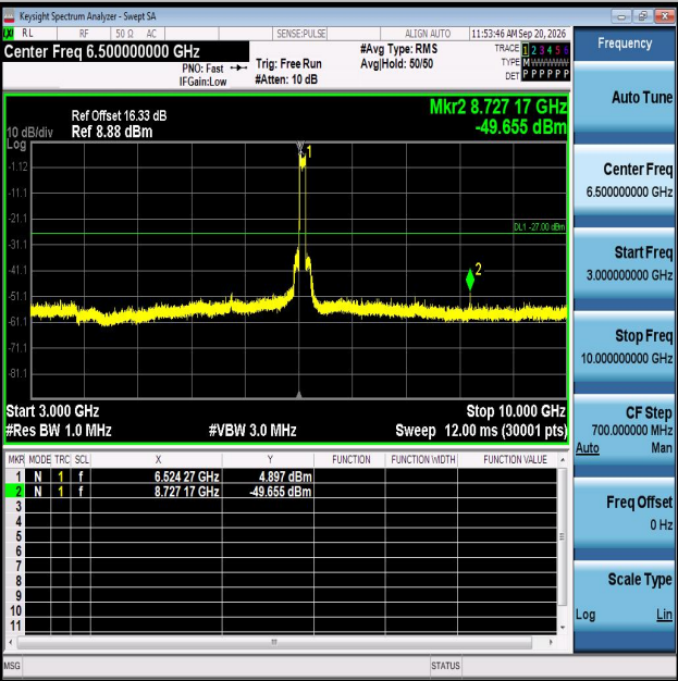
11AX80MIMO-Ant1-6545-3000~10000-PASS
