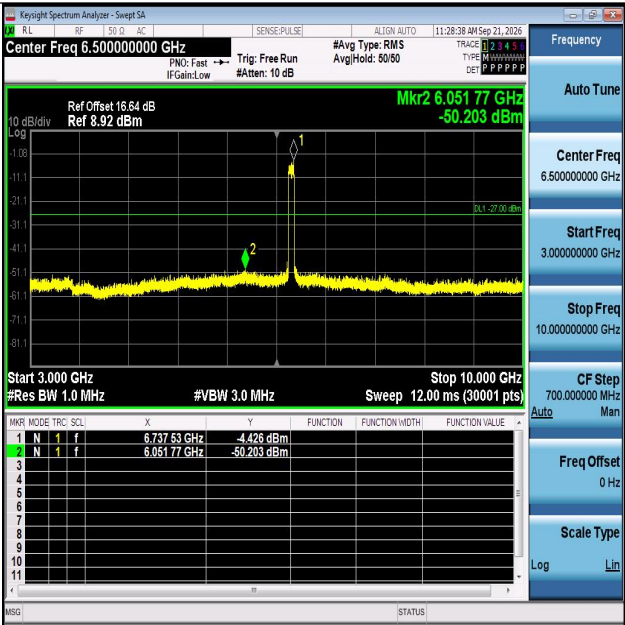
11AX80MIMO-Ant2-6705-3000~10000-PASS
