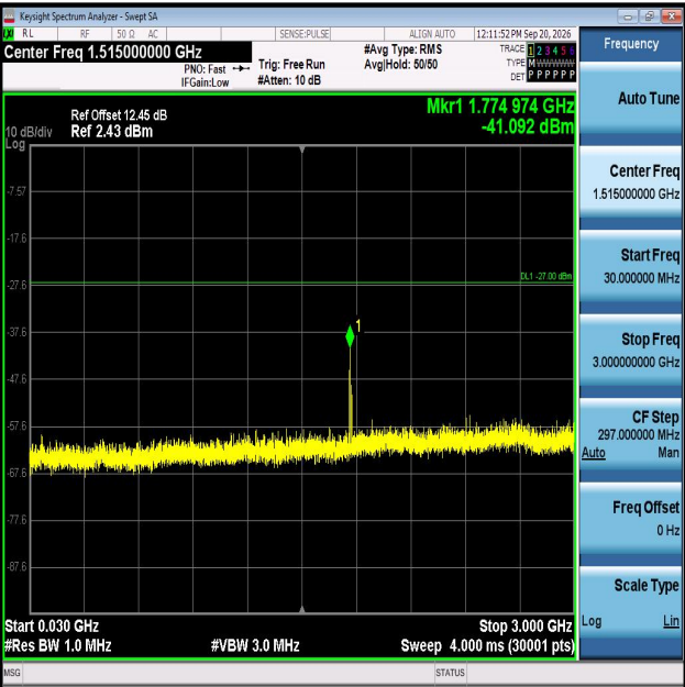
11AX80MIMO-Ant1-6785-30~3000-PASS
