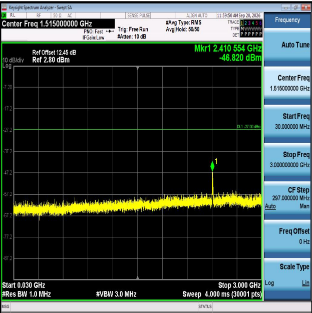
11AX80MIMO-Ant1-6625-30~3000-PASS
