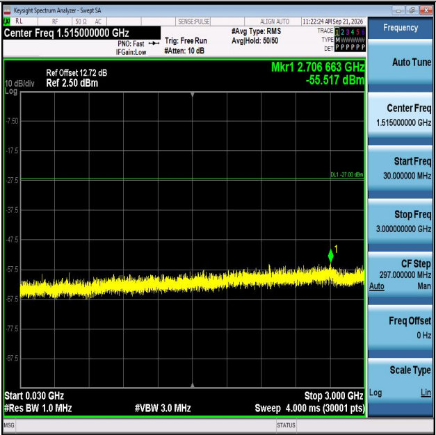
11AX80MIMO-Ant2-6625-30~3000-PASS
