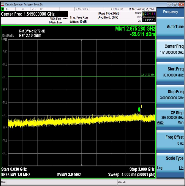
11AX80MIMO-Ant2-6545-30~3000-PASS
