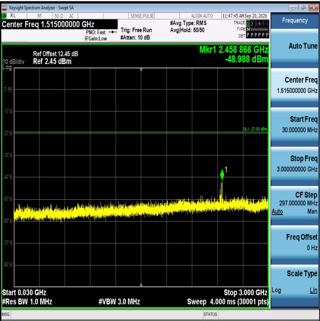
11AX80MIMO-Ant1-6465-30~3000-PASS
