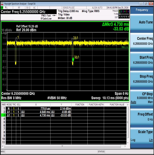
NTNV-11AX20MIMO-Ant2-6255
