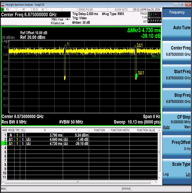
NTNV-11AX20MIMO-Ant2-6875
