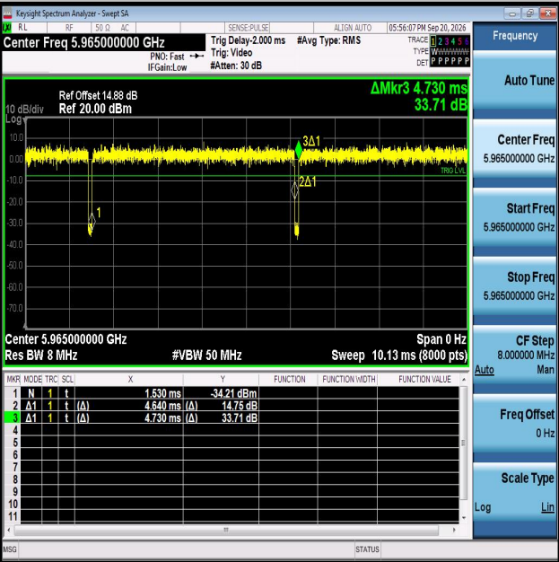
NTNV-11AX40MIMO-Ant2-5965
