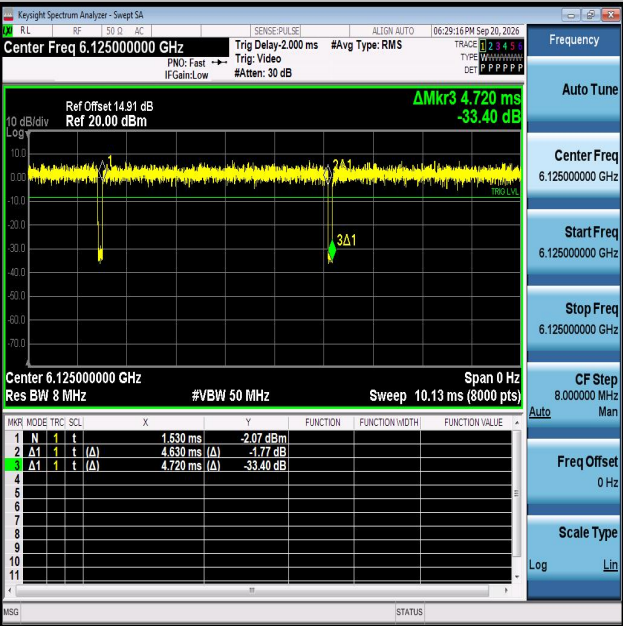
NTNV-11AX40MIMO-Ant2-6125
