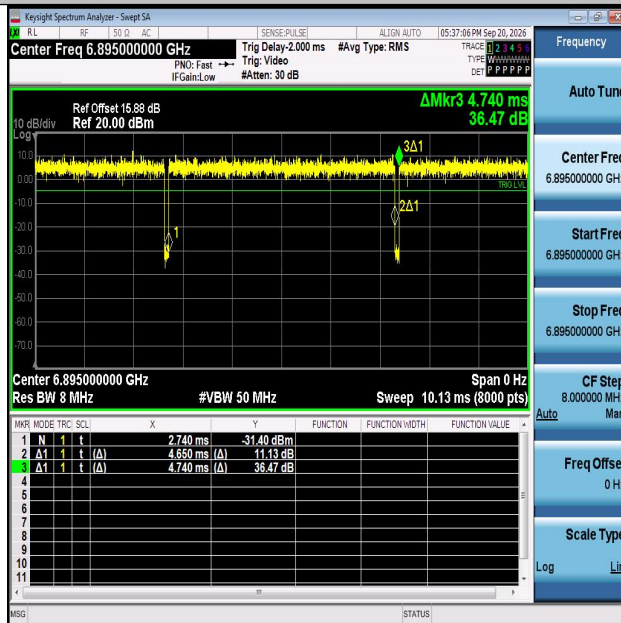
NTNV-11AX20MIMO-Ant2-6895
