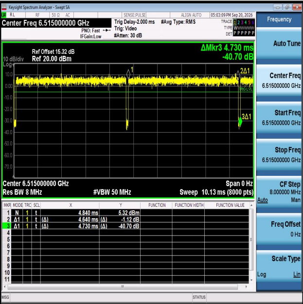
NTNV-11AX20MIMO-Ant2-6515
