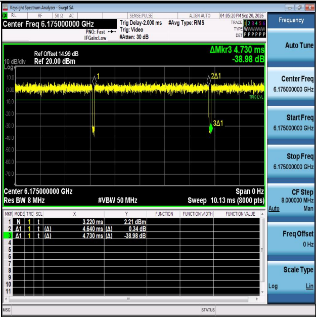
NTNV-11AX20MIMO-Ant2-6175
