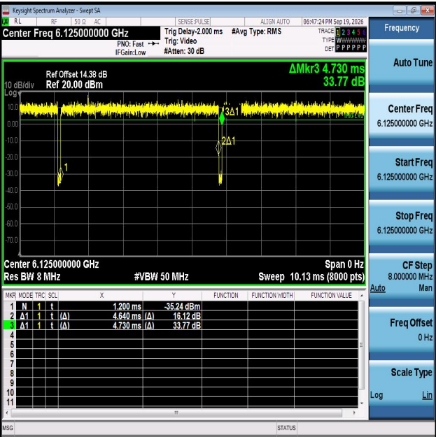
NTNV-11AX40MIMO-Ant1-6125
