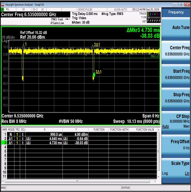
NTNV-11AX20MIMO-Ant2-6535
