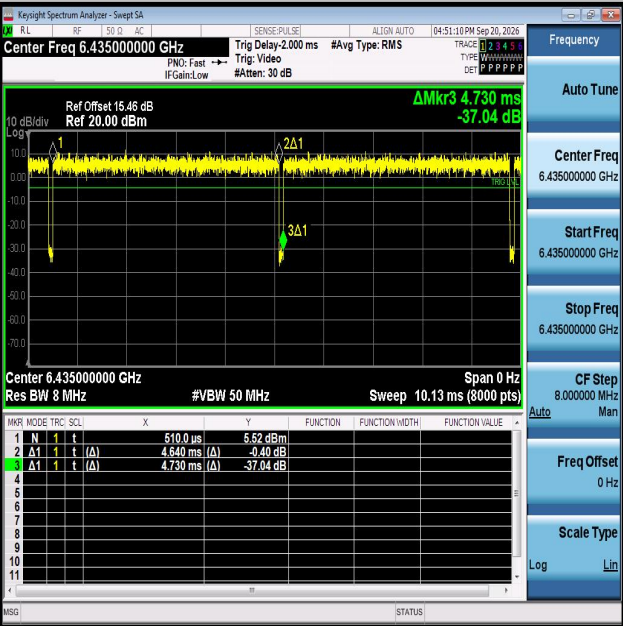
NTNV-11AX20MIMO-Ant2-6435
