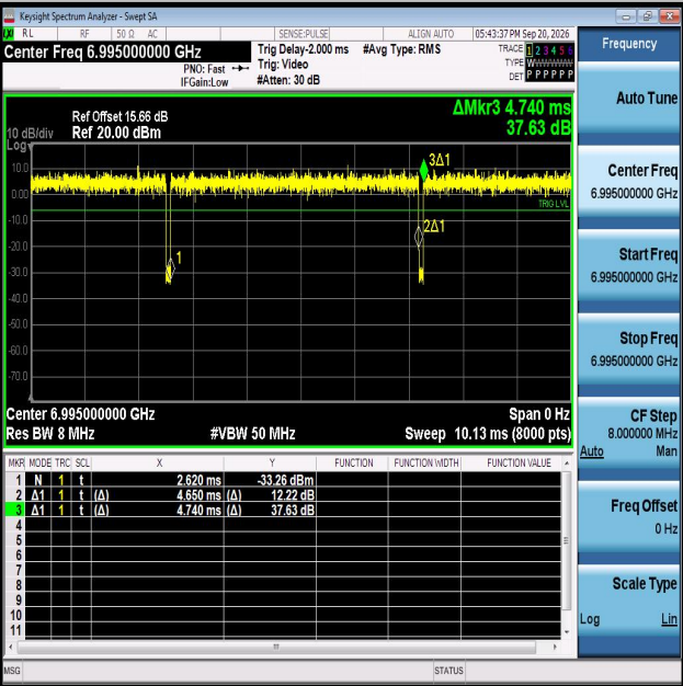
NTNV-11AX20MIMO-Ant2-6995
