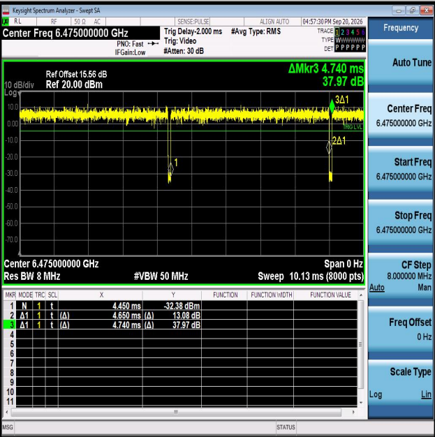
NTNV-11AX20MIMO-Ant2-6475
