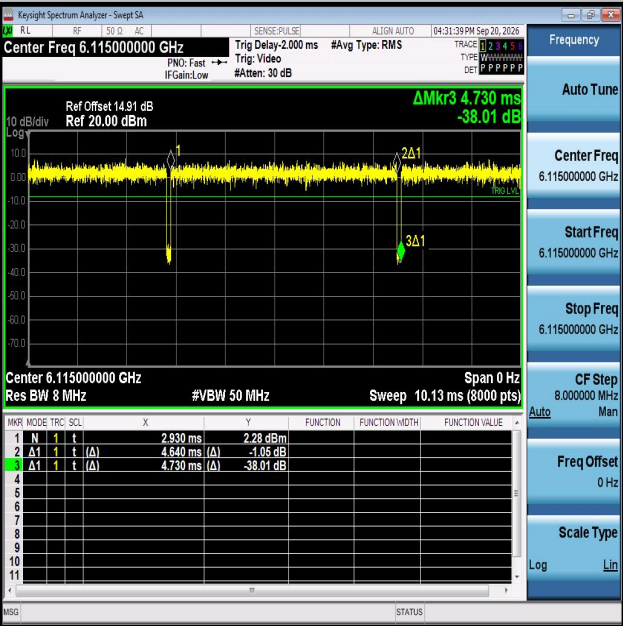
NTNV-11AX20MIMO-Ant2-6115
