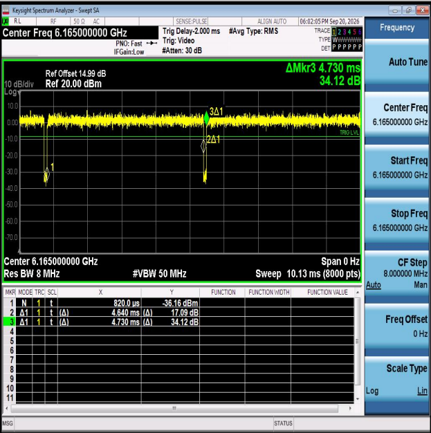
NTNV-11AX40MIMO-Ant2-6165
