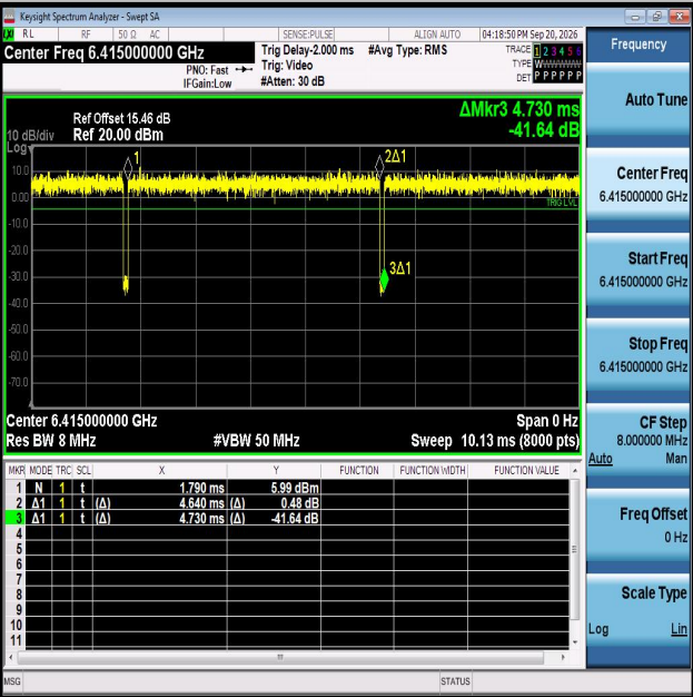
NTNV-11AX20MIMO-Ant2-6415
