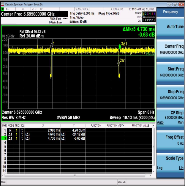
NTNV-11AX20MIMO-Ant2-6695
