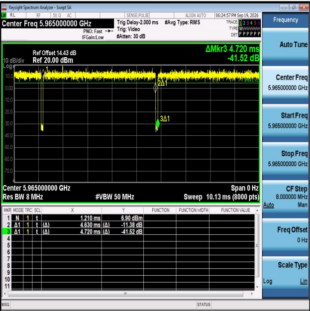
NTNV-11AX40MIMO-Ant1-5965
