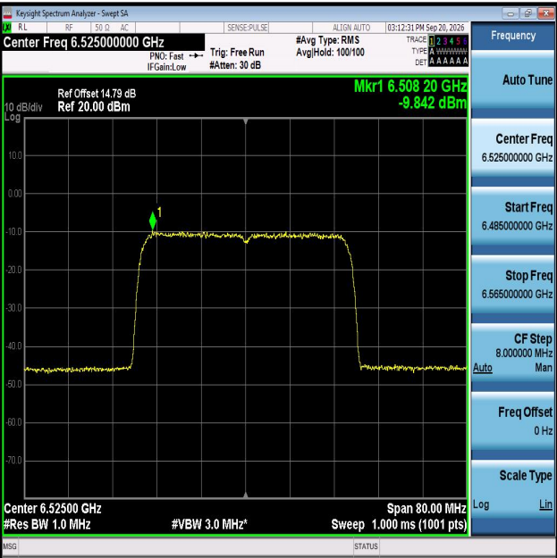
11AX40MIMO-Ant1-6525-PASS
