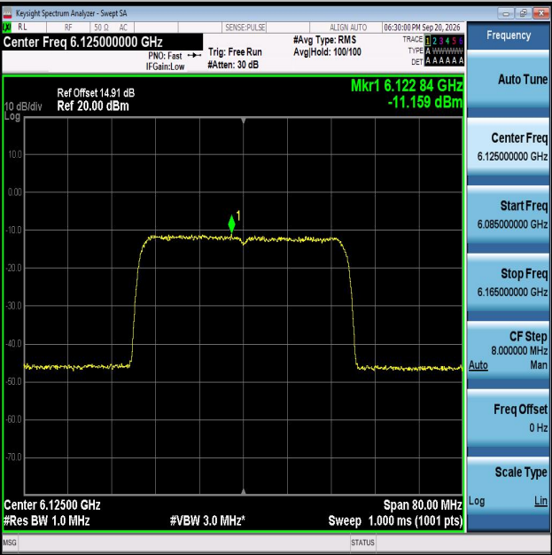
11AX40MIMO-Ant2-6125-PASS
