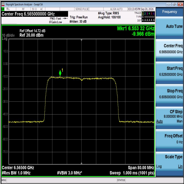
11AX40MIMO-Ant1-6565-PASS
