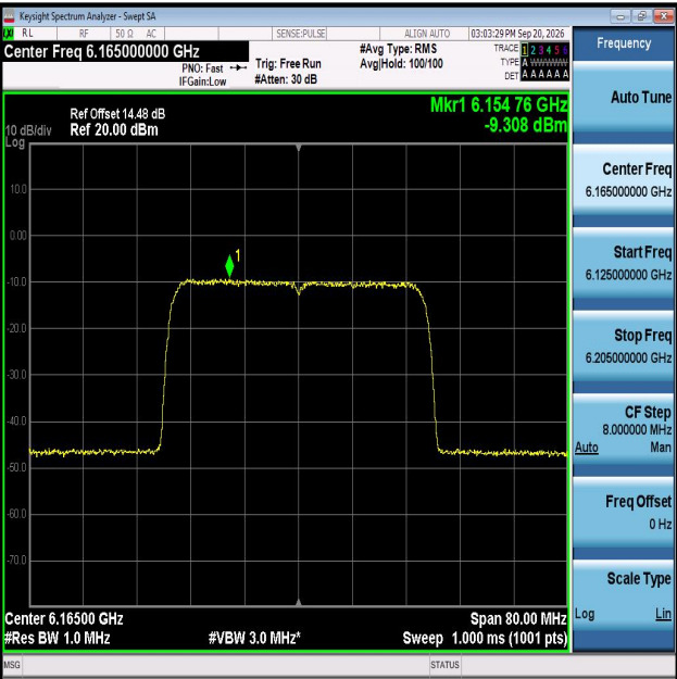
11AX40MIMO-Ant1-6165-PASS
