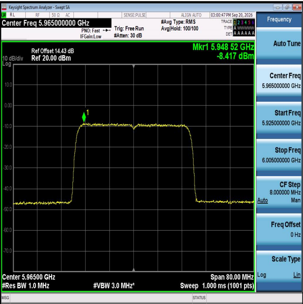
11AX40MIMO-Ant1-5965-PASS
