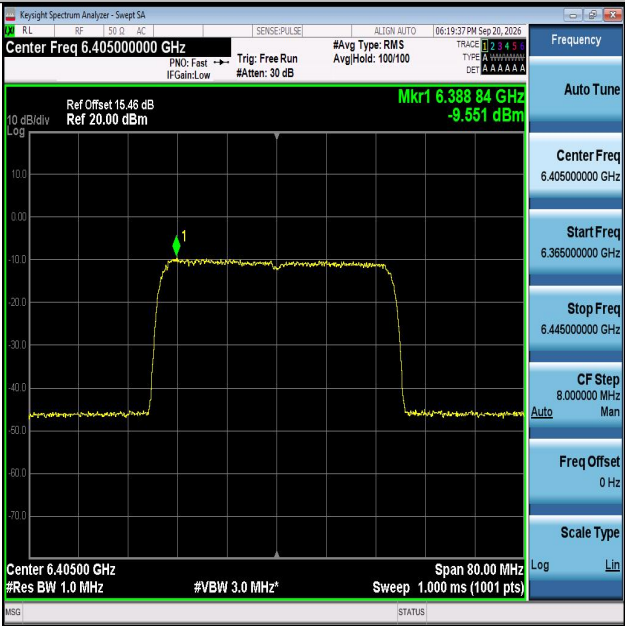
11AX40MIMO-Ant2-6405-PASS
