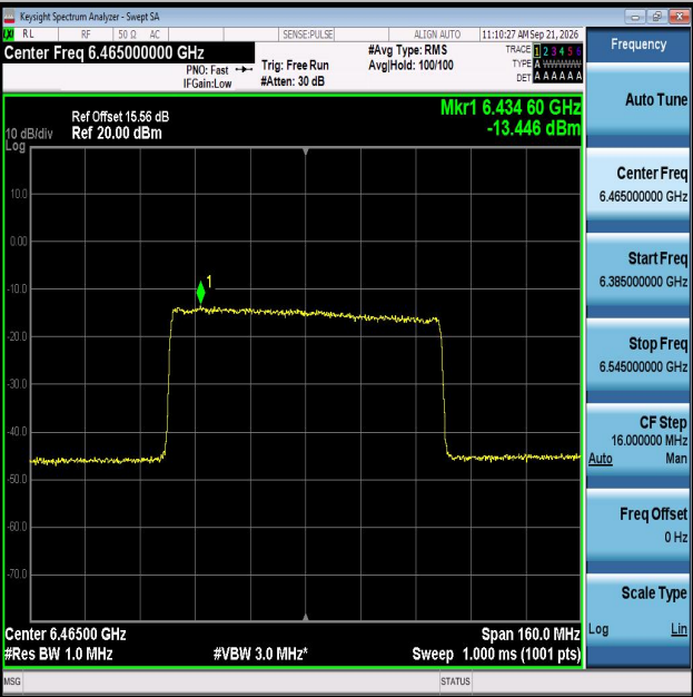
11AX80MIMO-Ant2-6465-PASS
