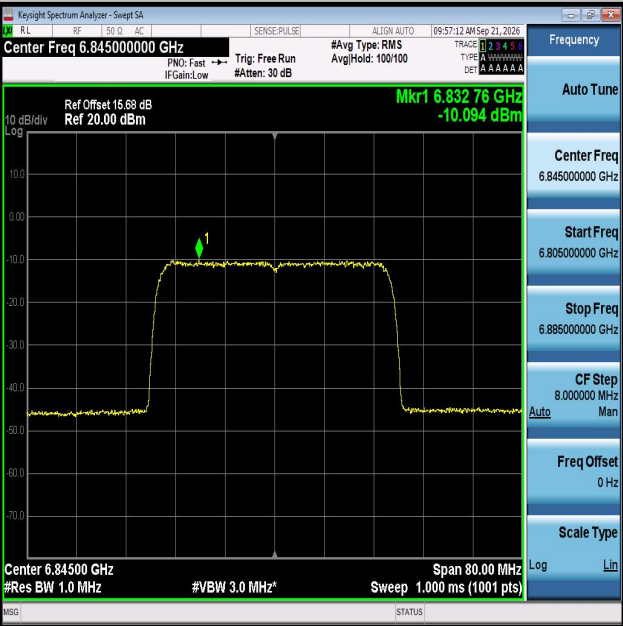
11AX40MIMO-Ant2-6845-PASS
