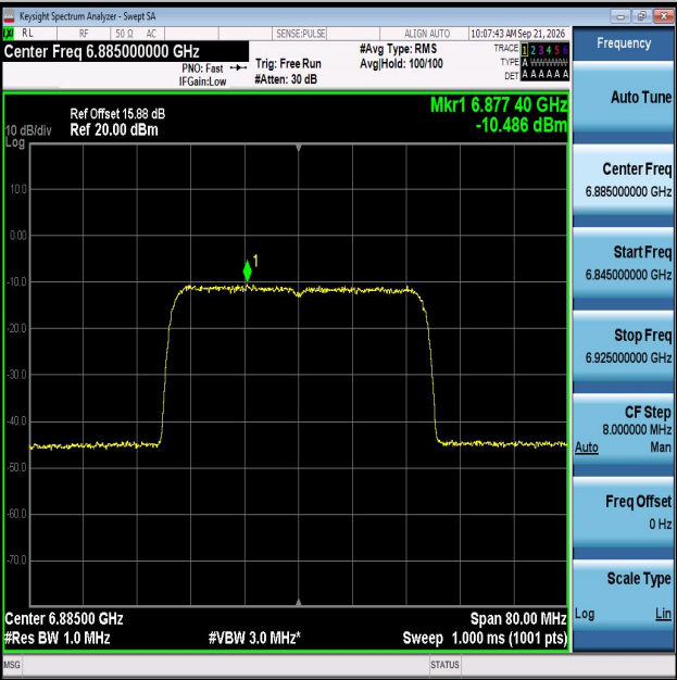
11AX40MIMO-Ant2-6885-PASS
