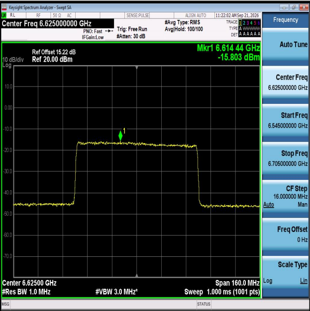
11AX80MIMO-Ant2-6625-PASS
