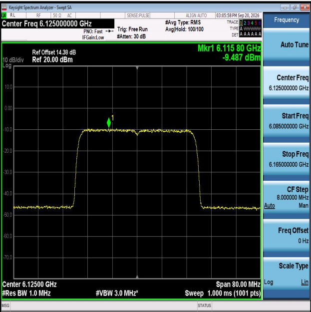
11AX40MIMO-Ant1-6125-PASS
