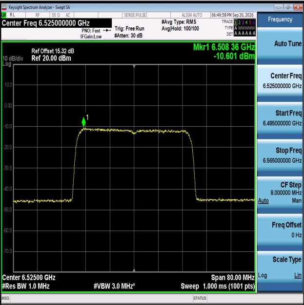
11AX40MIMO-Ant2-6525-PASS
