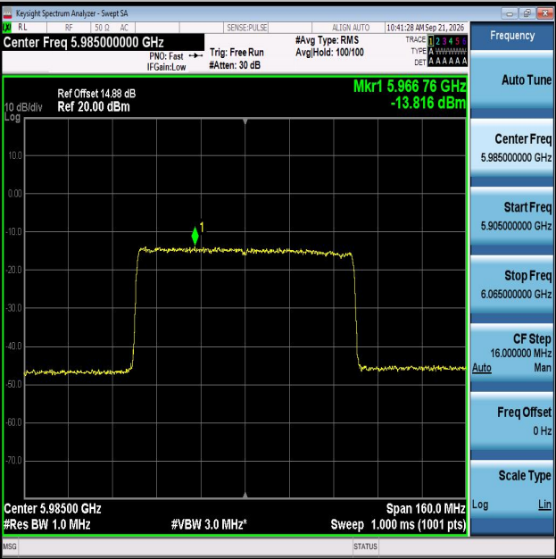
11AX80MIMO-Ant2-5985-PASS
