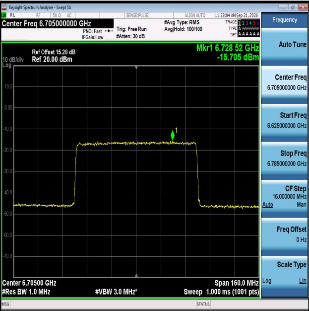
11AX80MIMO-Ant2-6705-PASS
