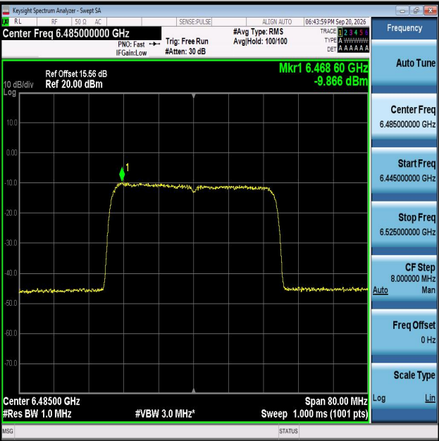
11AX40MIMO-Ant2-6485-PASS
