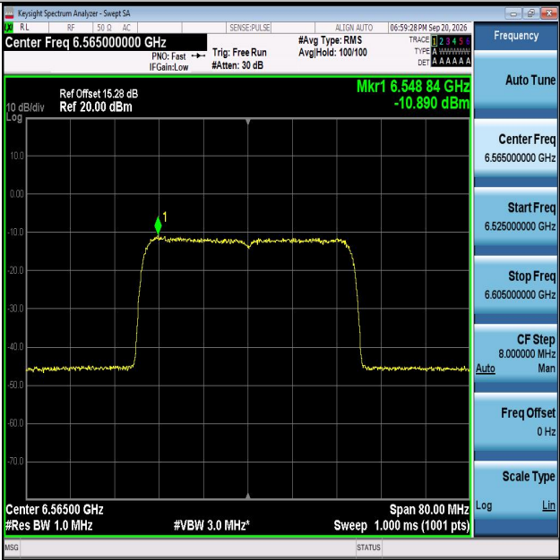
11AX40MIMO-Ant2-6565-PASS
