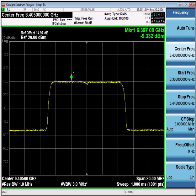
11AX40MIMO-Ant1-6405-PASS
