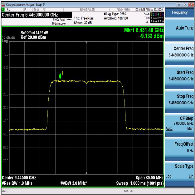
11AX40MIMO-Ant1-6445-PASS
