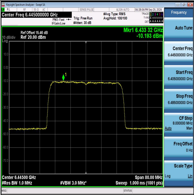
11AX40MIMO-Ant2-6445-PASS
