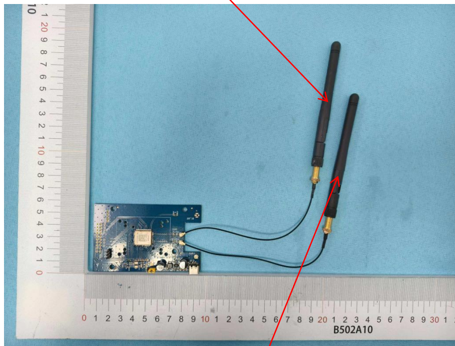
BT+WiFi ANT2
