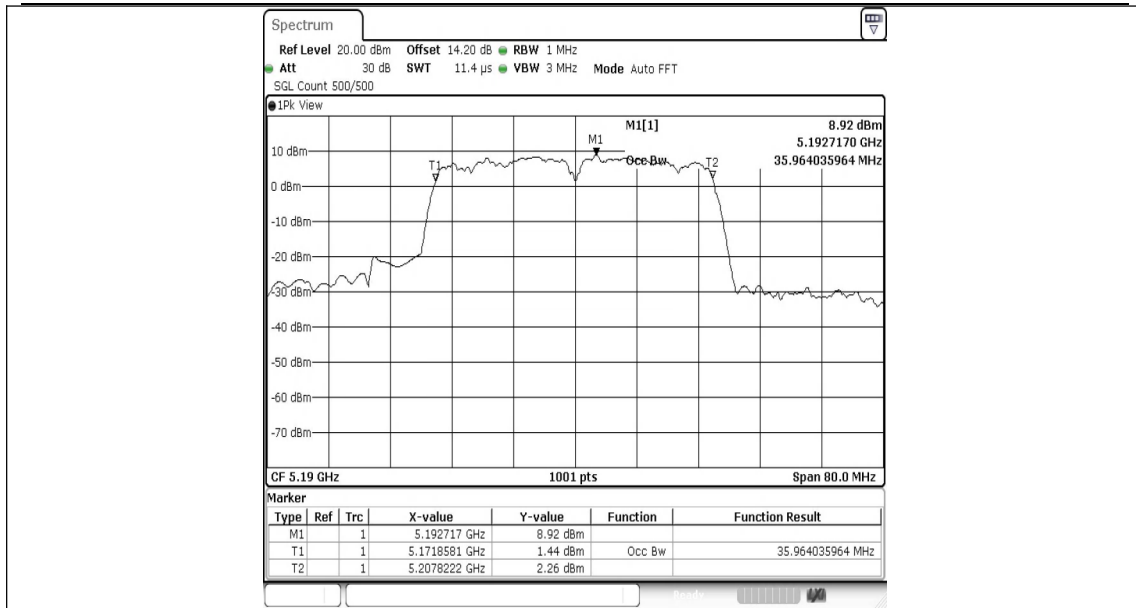
11AC40MIMO-Ant1-5190
