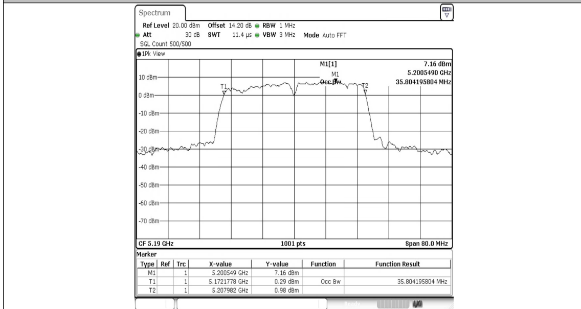
11AC40MIMO-Ant1-5190
