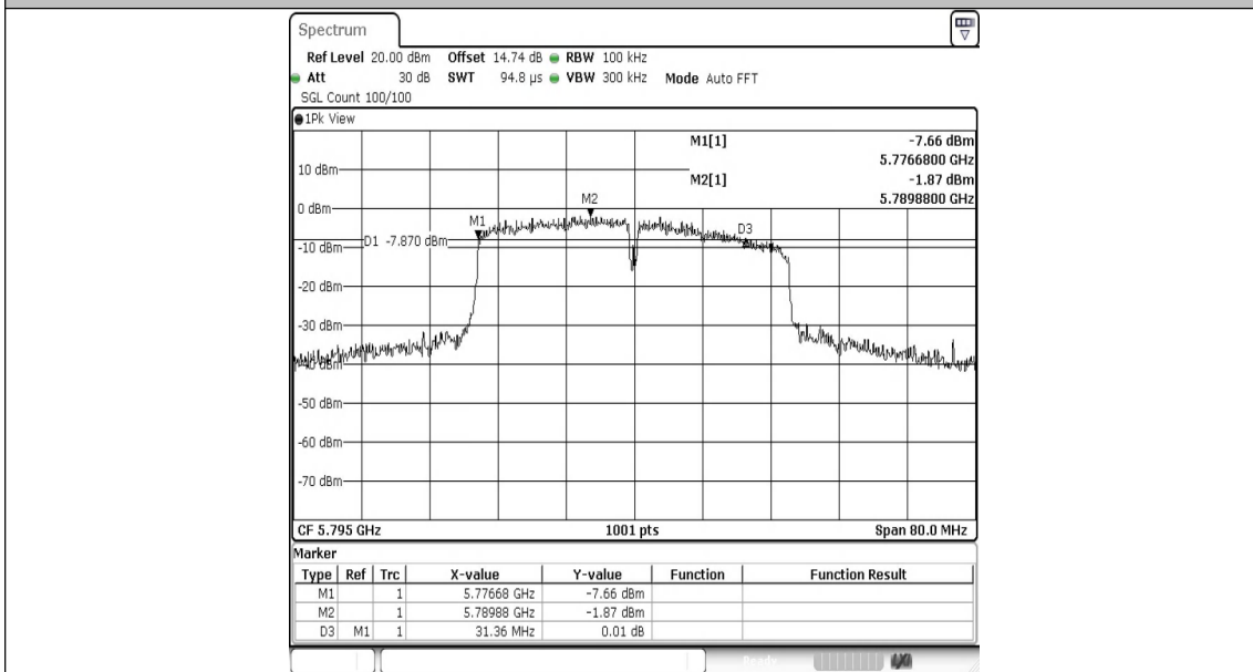
11AC40MIMO-Ant1-5795-PASS
