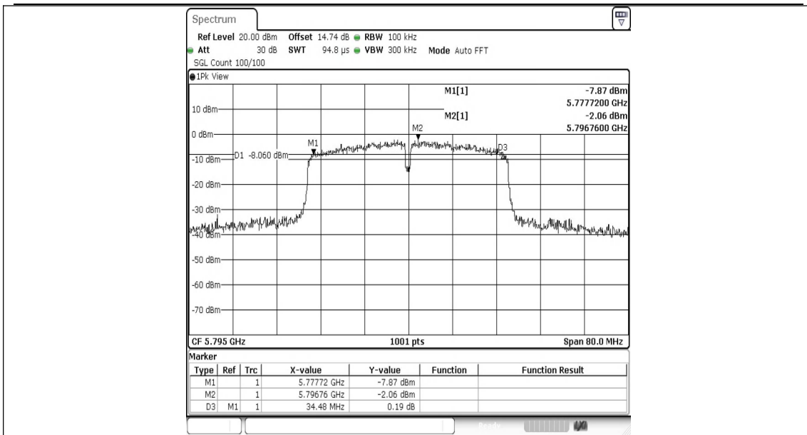
11AC40MIMO-Ant1-5795-PASS
