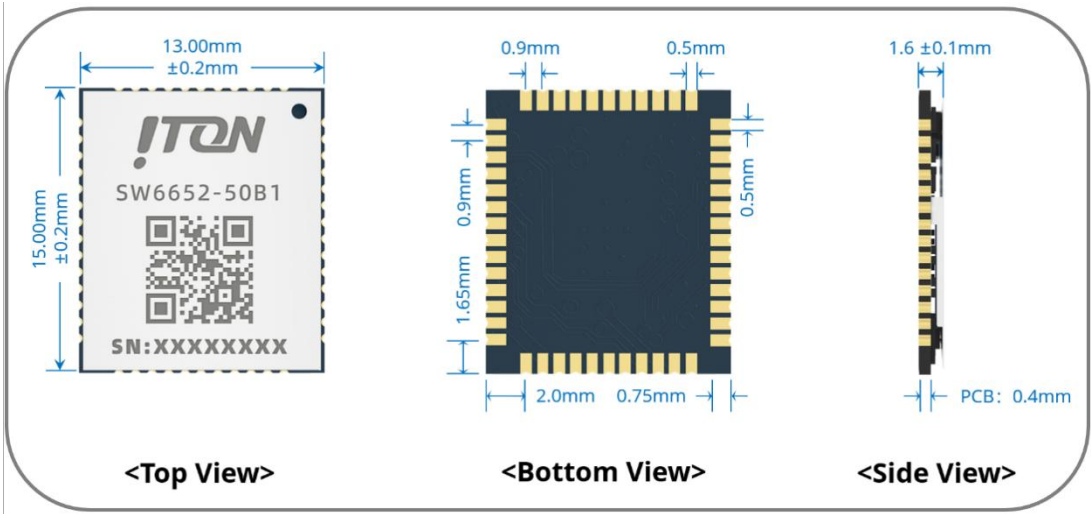
Figure 5. Module Size of SW6652-50B1(2)
