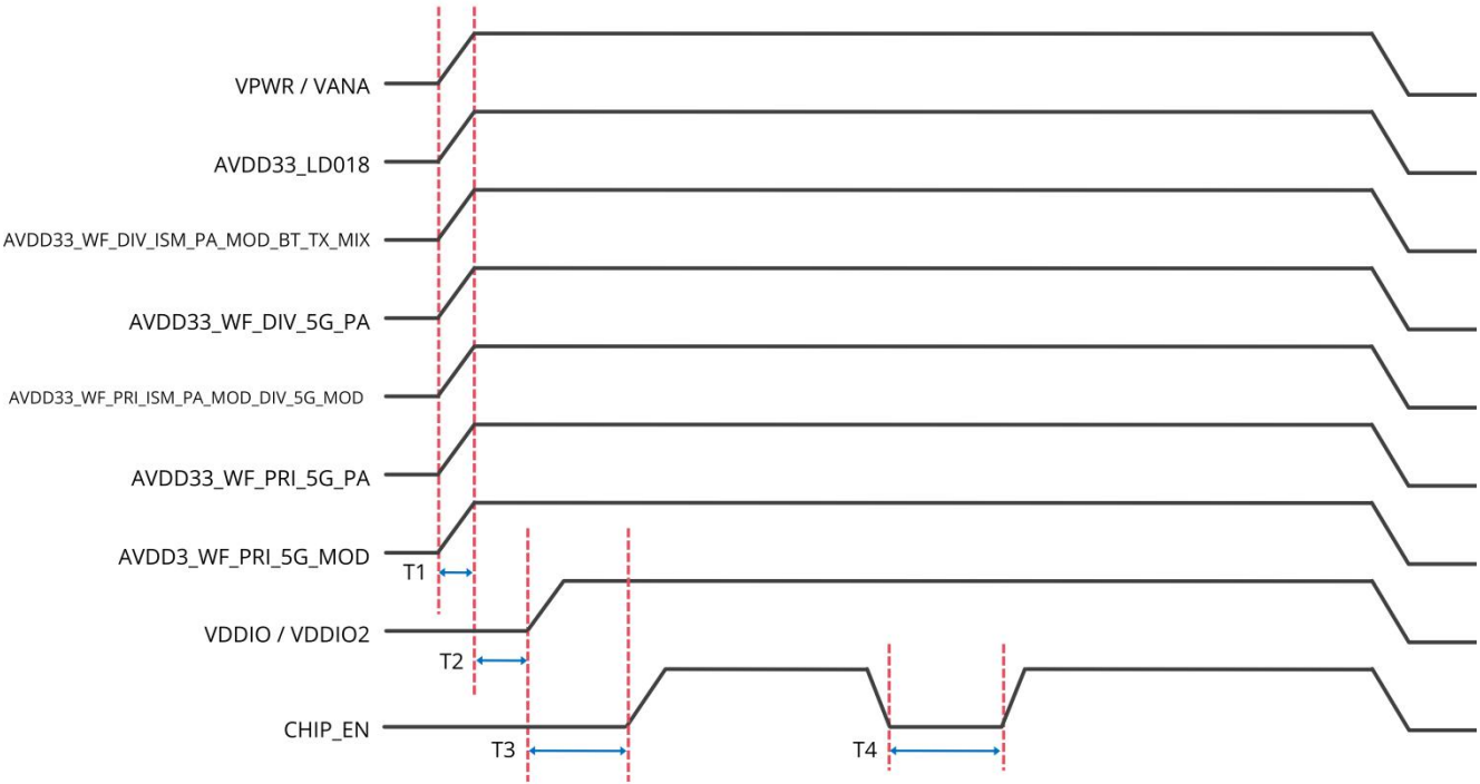
Figure 3. Power on/off and Reset timing of SW6652-50B1(2)
