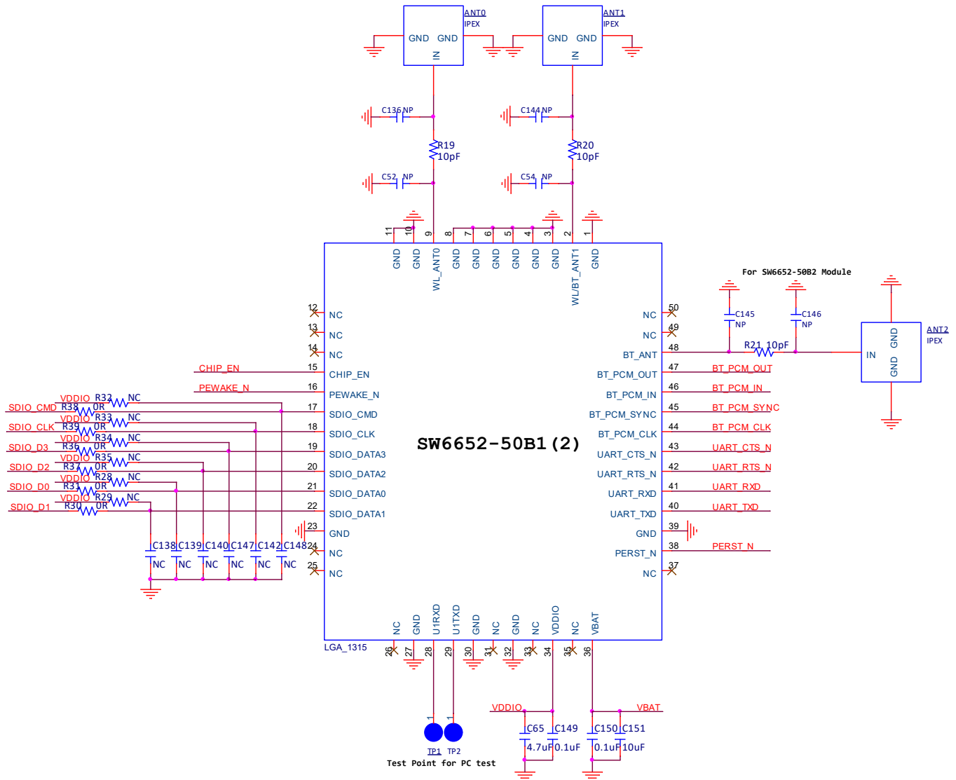
Figure 4. Application Schematic Diagram of SW6652-50B1(2)
