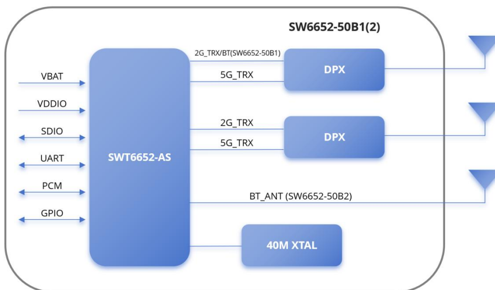
Figure 1. Block Diagram of SW6652-50B1(2)
