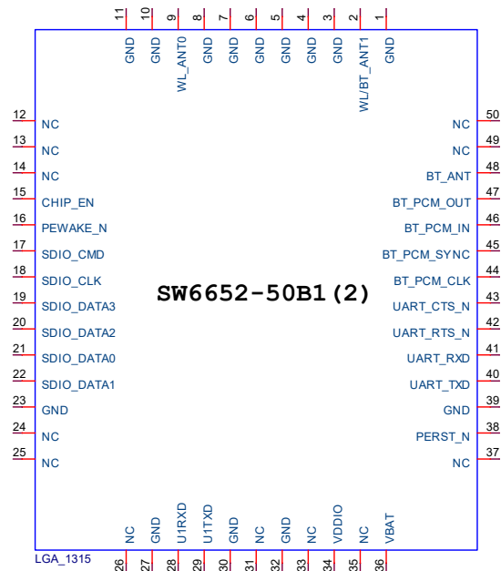
Figure 2. Pin Diagram of SW6652-50B1(2)
