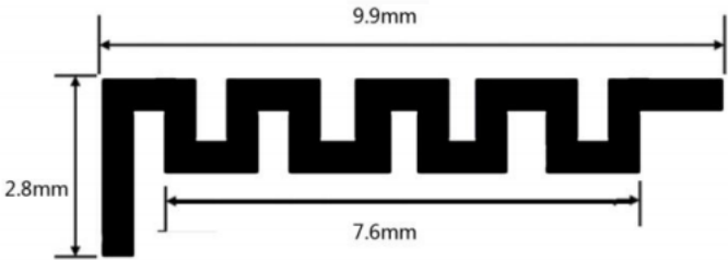
Antenna Photo & Length (mm)
