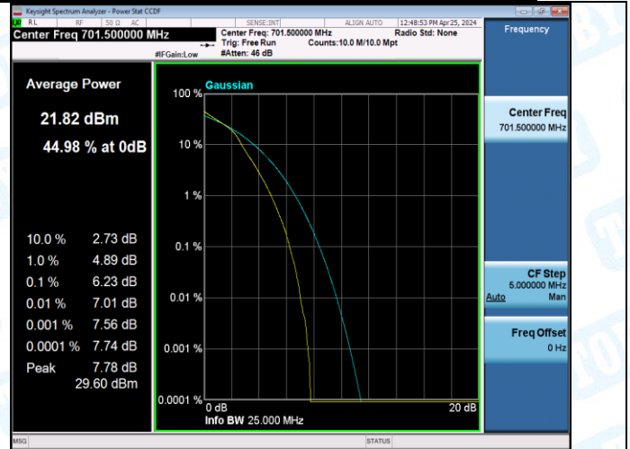
Band12-5MHz-16QAM-23095-25RB#0-PASS
