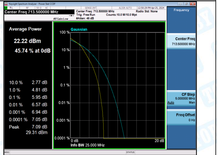
Band12-10MHz-QPSK-23060-50RB#0-PASS
