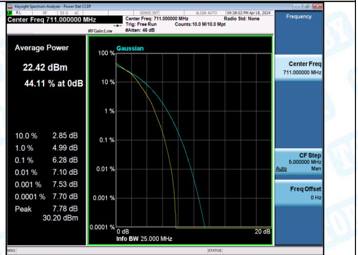
Band12-10MHz-16QAM-23130-27RB#0-PASS
