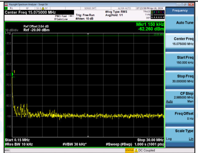
Band12_1.4MHz_QPSK_23173_6RB#0_1000~3000_1000~3000
