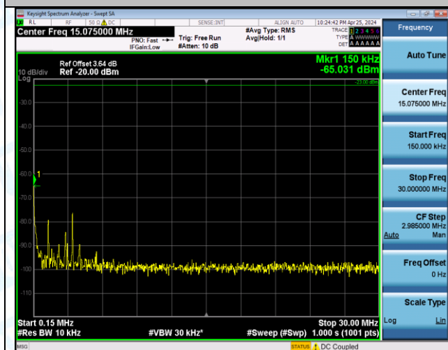
Band12_10MHz_QPSK_23095_50RB#0_1000~3000_1000~3000
