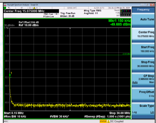
Band13_5MHz_QPSK_23205_25RB#0_1000~3000_1000~3000
