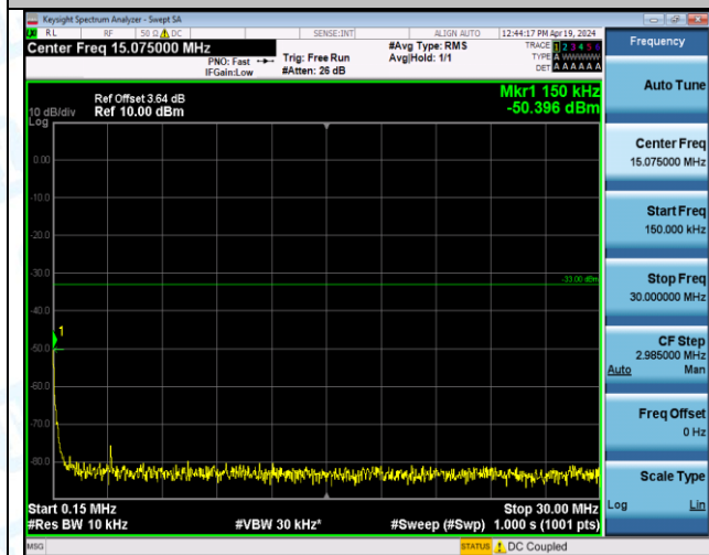
Band2_15MHz_QPSK_18675_75RB#0_1000~3000_1000~3000
