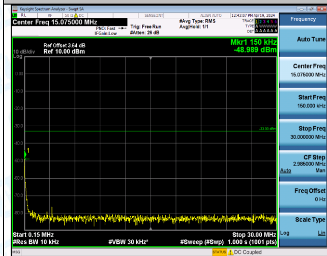
Band2_15MHz_16QAM_19125_1RB#74_1000~3000_1000~3000
