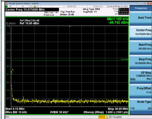
Band2_20MHz_QPSK_18900_1RB#0_1000~3000_1000~3000
