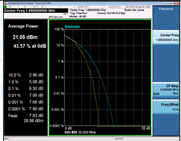
Band2-10MHz-16QAM-19150-27RB#0-PASS
