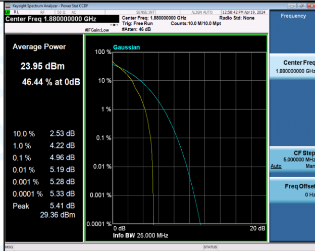
Band2-15MHz-QPSK-18800-1RB#0-PASS
