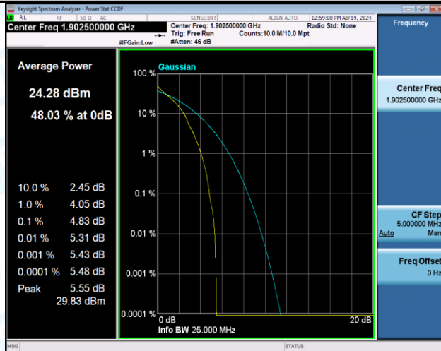
Band2-15MHz-QPSK-19125-1RB#0-PASS
