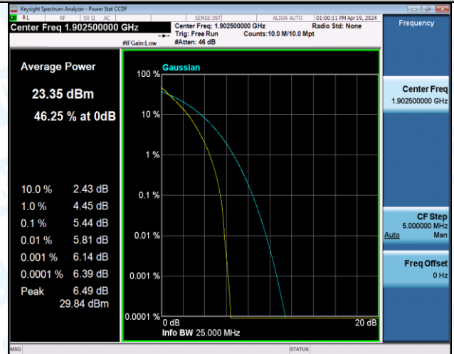
Band2-15MHz-QPSK-19125-75RB#0-PASS
