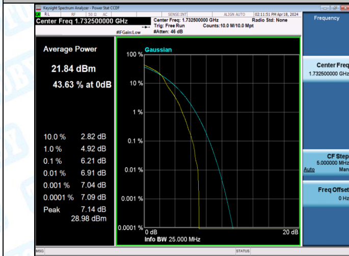
Band4-5MHz-16QAM-20375-1RB#0-PASS
