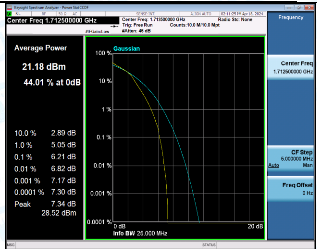
Band4-5MHz-16QAM-20175-25RB#0-PASS
