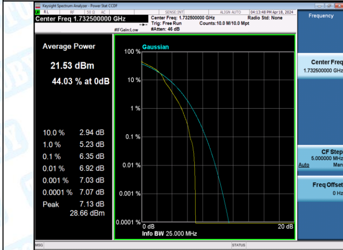
Band4-15MHz-16QAM-20325-1RB#0-PASS
