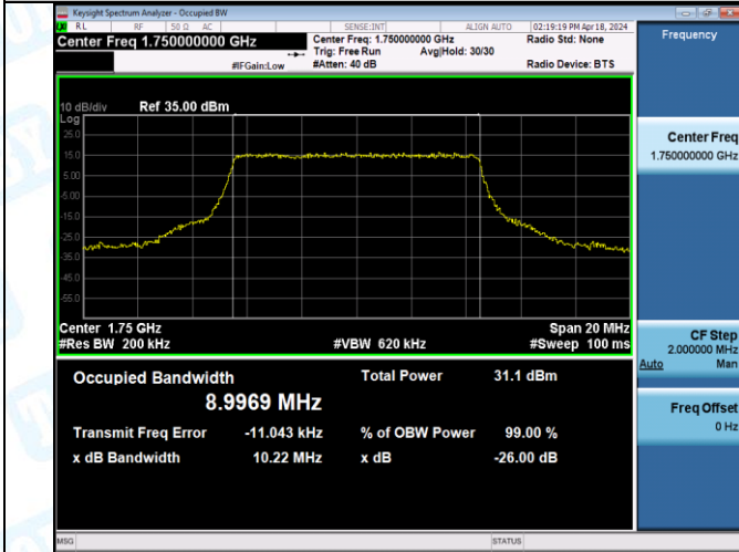
Band4-10MHz-16QAM-20175-27RB#0-PASS
