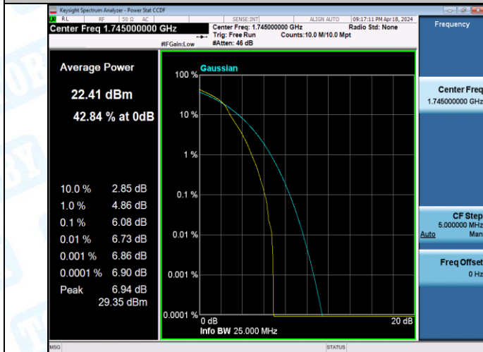
Band4-20MHz-16QAM-20300-1RB#0-PASS
