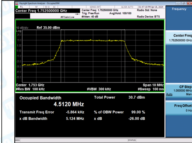
Band4-5MHz-16QAM-20175-25RB#0-PASS
