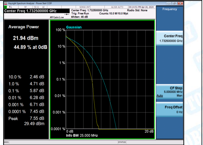
Band4-15MHz-QPSK-20325-75RB#0-PASS
