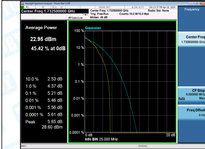
Band4-15MHz-QPSK-20325-1RB#0-PASS
