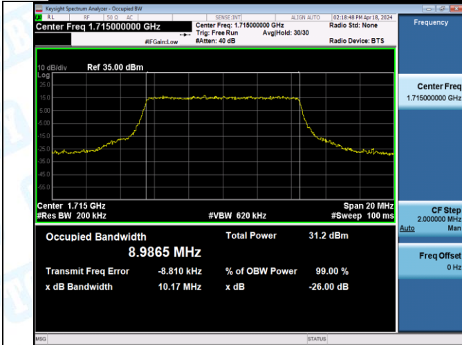
Band4-10MHz-QPSK-20350-50RB#0-PASS
