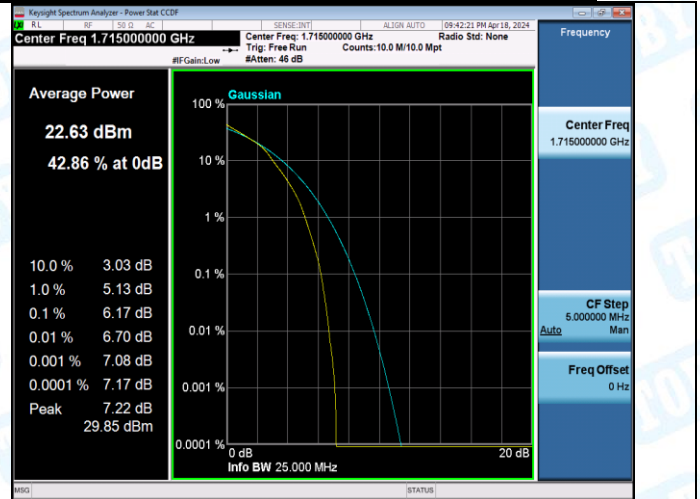
Band4-10MHz-16QAM-20175-27RB#0-PASS
