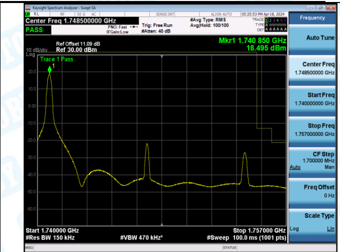
Band4_15MHz_QPSK_20325_75RB#0
