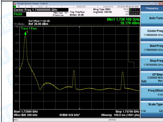
Band4_20MHz_16QAM_20300_1RB#0
