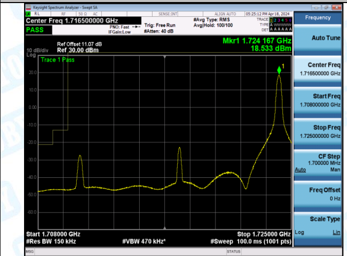
Band4_15MHz_QPSK_20325_1RB#0
