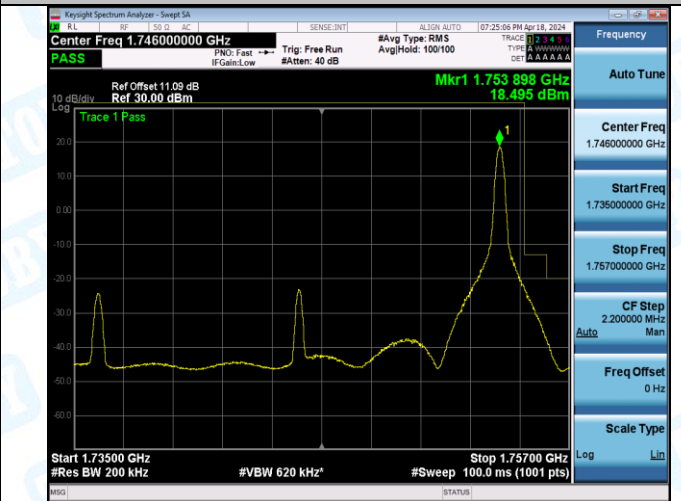
Band4_20MHz_16QAM_20300_1RB#99
