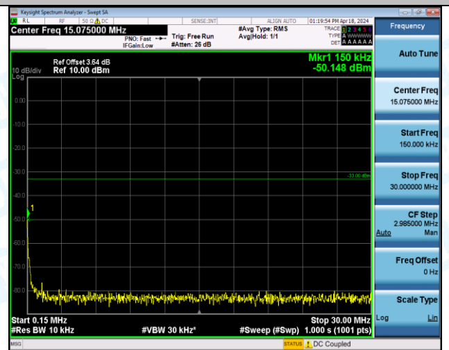
Band4_3MHz_QPSK_19965_15RB#0_1000~3000_1000~3000
