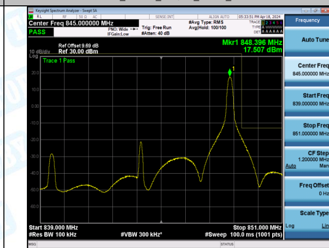
Band5_10MHz_16QAM_20600_1RB#49
