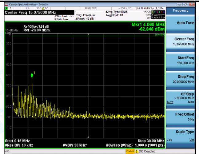
Band5_10MHz_QPSK_20450_50RB#0_1000~3000_1000~3000
