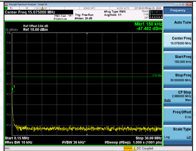
Band66_5MHz_QPSK_132647_25RB#0_1000~3000_1000~3000
