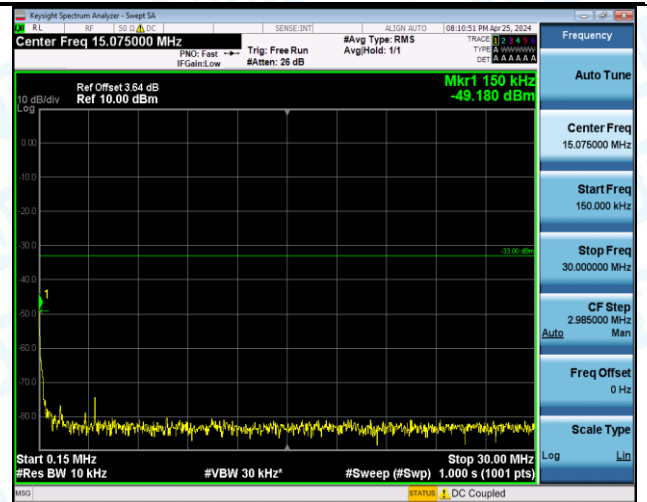
Band66_15MHz_16QAM_132047_1RB#0_1000~3000_1000~3000
