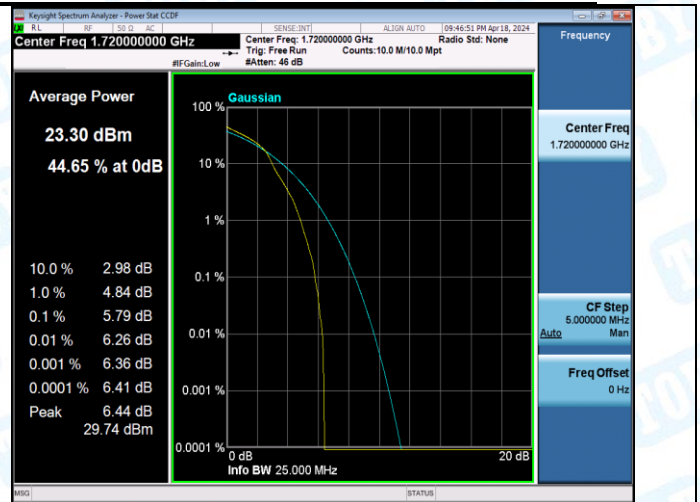
Band66-20MHz-16QAM-132322-1RB#0-PASS
