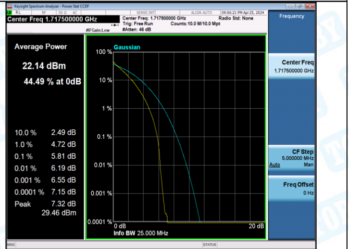
Band66-15MHz-QPSK-132322-75RB#0-PASS
