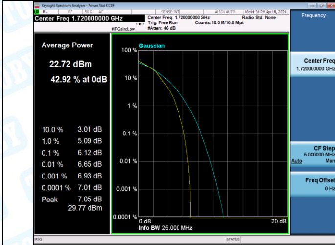
Band66-20MHz-16QAM-132322-27RB#0-PASS
