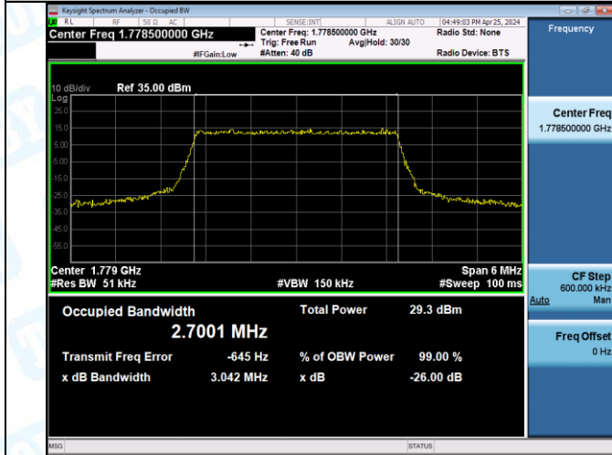
Band66-3MHz-16QAM-132322-15RB#0-PASS
