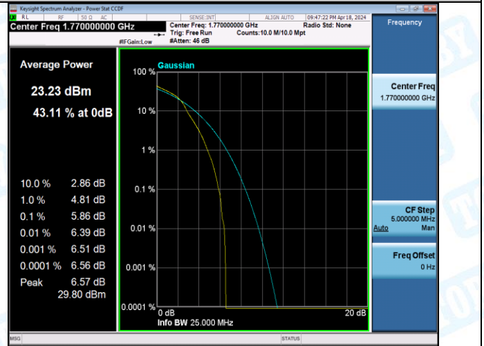
Band66-20MHz-16QAM-132572-1RB#0-PASS
