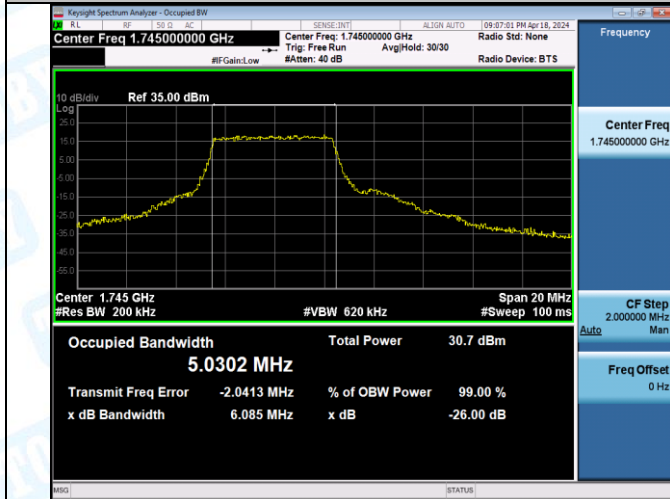
Band66-15MHz-QPSK-132047-75RB#0-PASS
