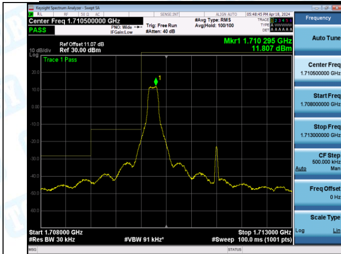
Band66_3MHz_16QAM_131987_15RB#0
