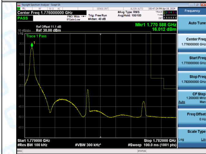
Band66_10MHz_16QAM_132622_1RB#0
