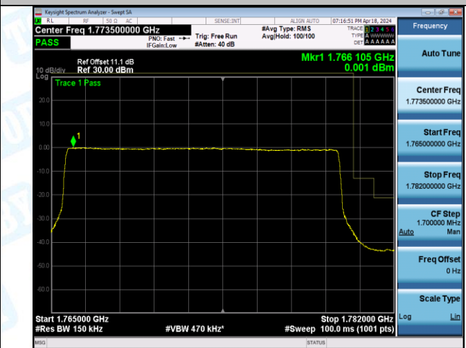
Band66_15MHz_QPSK_132597_75RB#0
