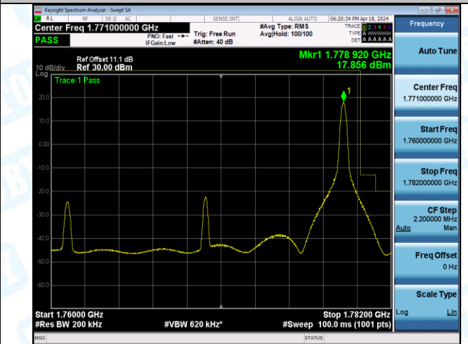
Band66_20MHz_16QAM_132572_1RB#99
