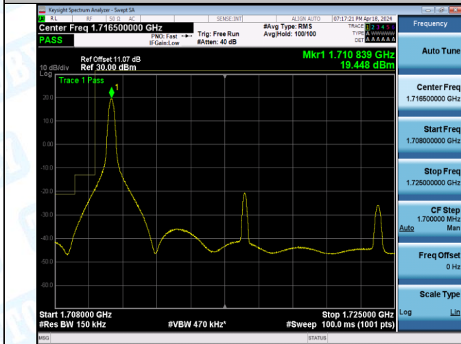
Band66_15MHz_QPSK_132047_1RB#0
