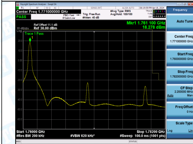
Band66_20MHz_16QAM_132572_1RB#0
