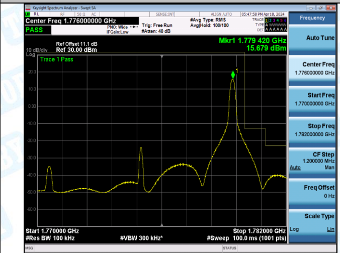
Band66_10MHz_16QAM_132622_1RB#49
