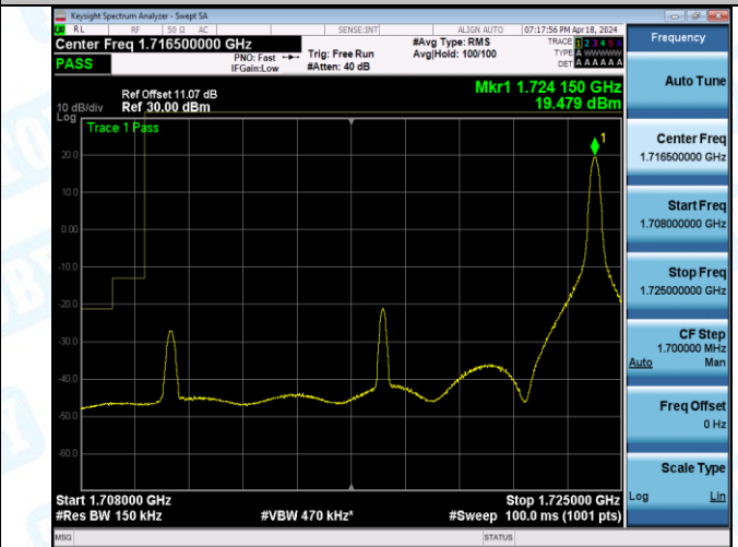
Band66_15MHz_QPSK_132047_1RB#74
