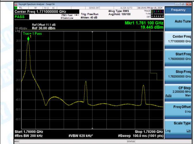
Band66_20MHz_QPSK_132572_100RB#0
