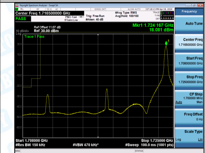
Band66_15MHz_16QAM_132047_1RB#74
