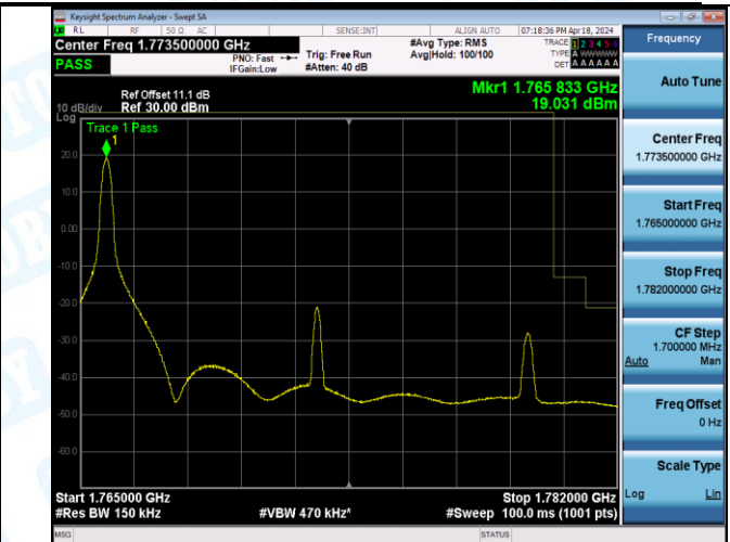
Band66_15MHz_QPSK_132597_75RB#0
