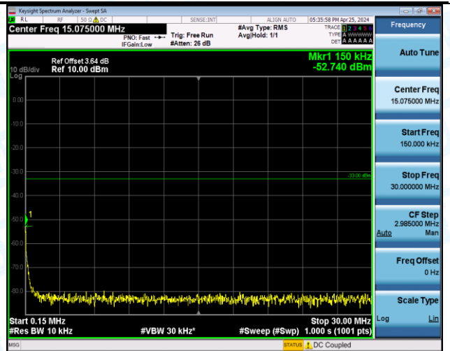
Band66_3MHz_QPSK_132657_1RB#0_1000~3000_1000~3000
