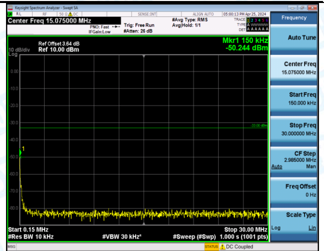
Band66_3MHz_16QAM_132322_1RB#0_1000~3000_1000~3000
