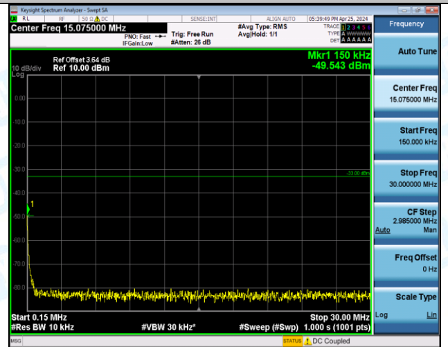
Band66_3MHz_QPSK_132657_15RB#0_1000~3000_1000~3000
