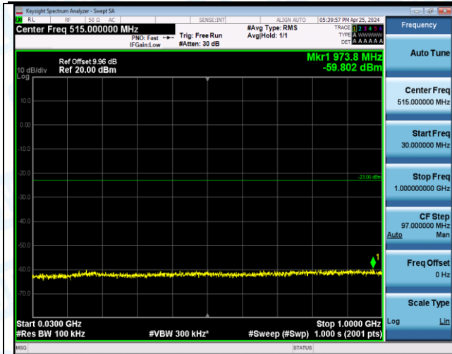
Band66_3MHz_QPSK_132657_15RB#0_3000~20000_3000~20000
