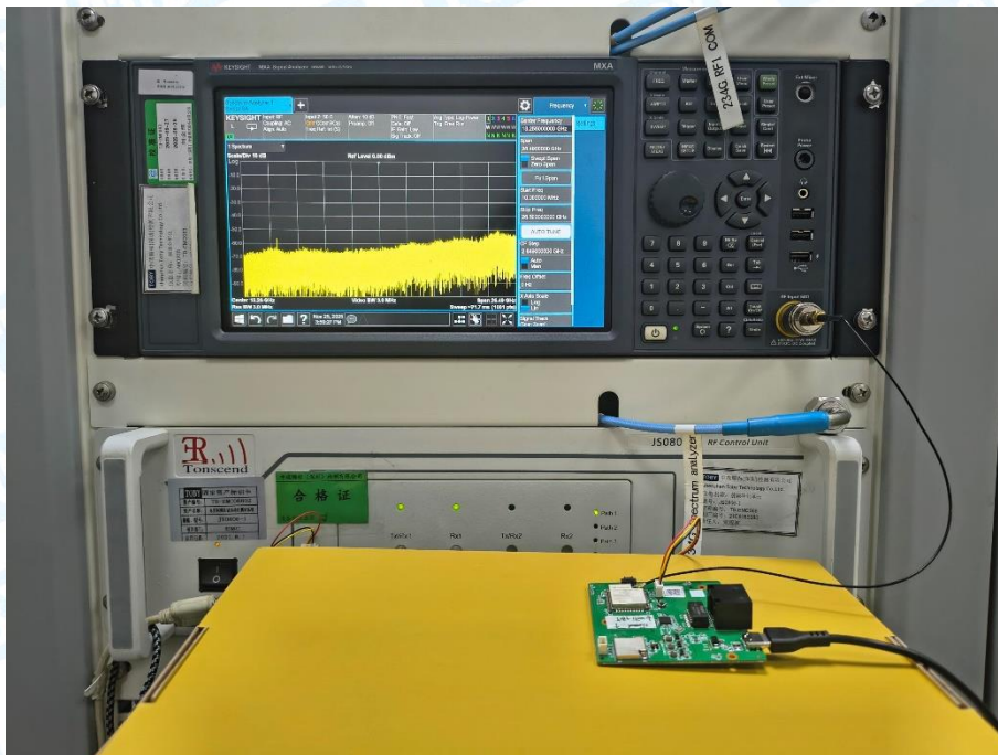
Photo of Setup for RF Conducted----BT&WIFI
